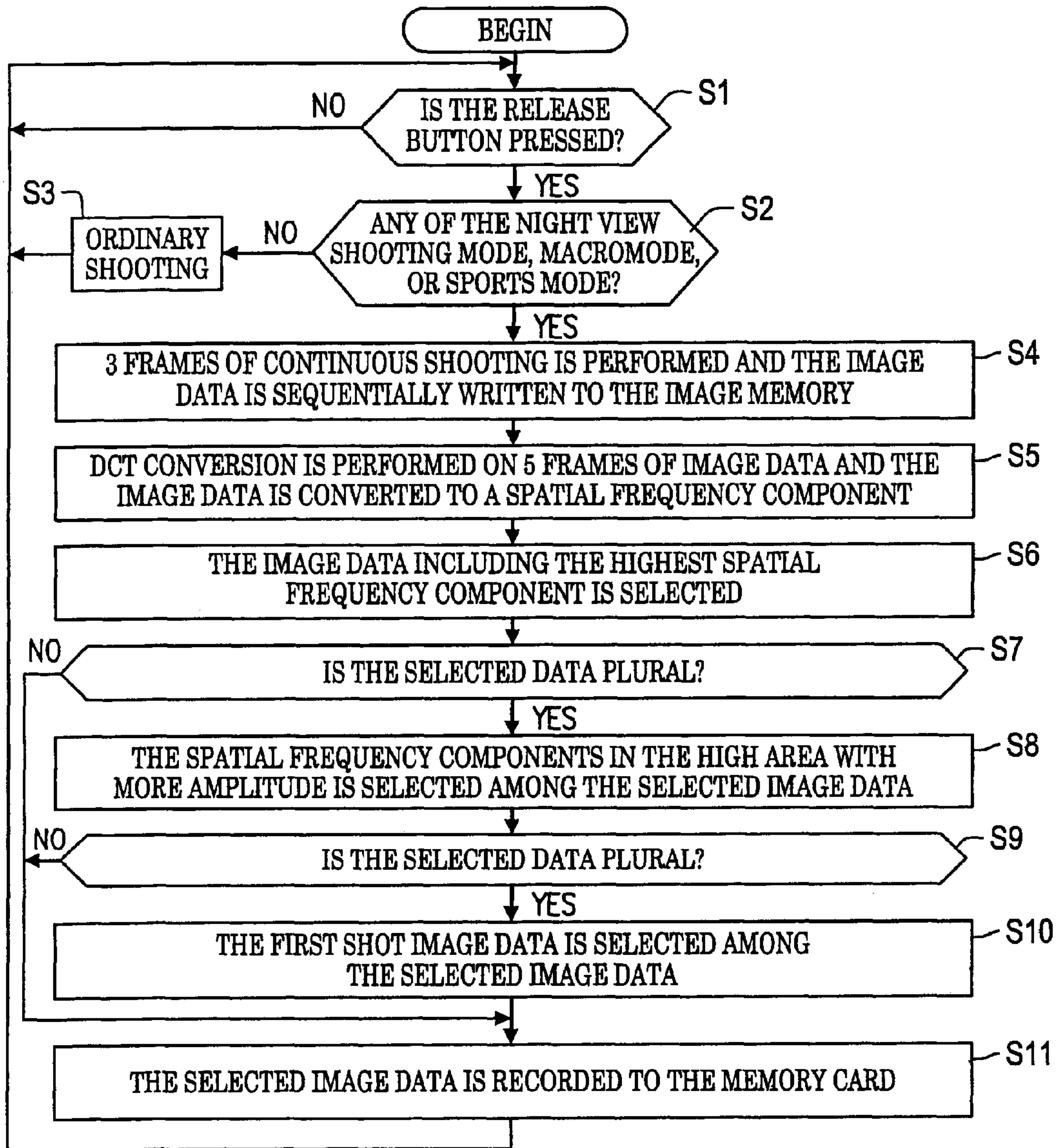
FLOW CHART EXPLAINING THE OPERATION OF THE FOURTH EMBODIMENT
