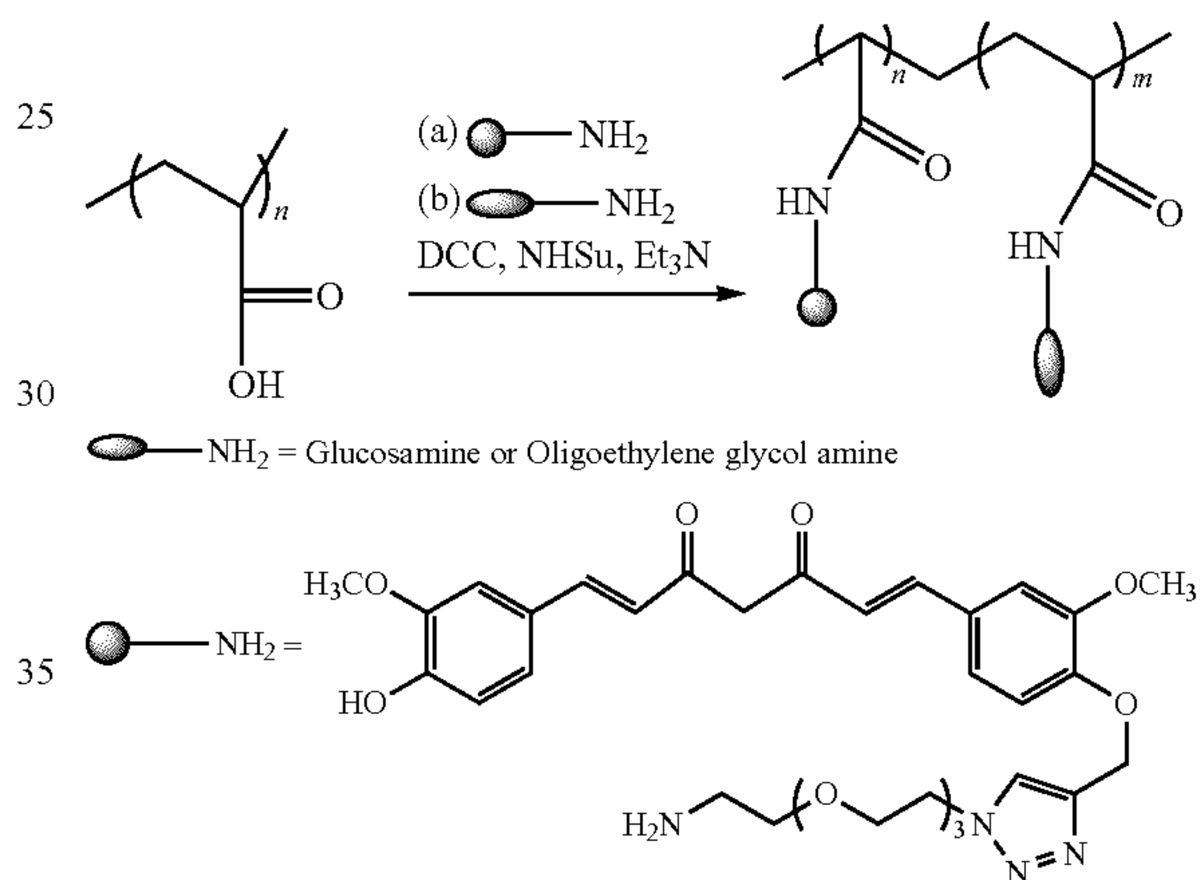
Scheme 2.2 Synthesis of curcumin polyacrylic acid conjugate
