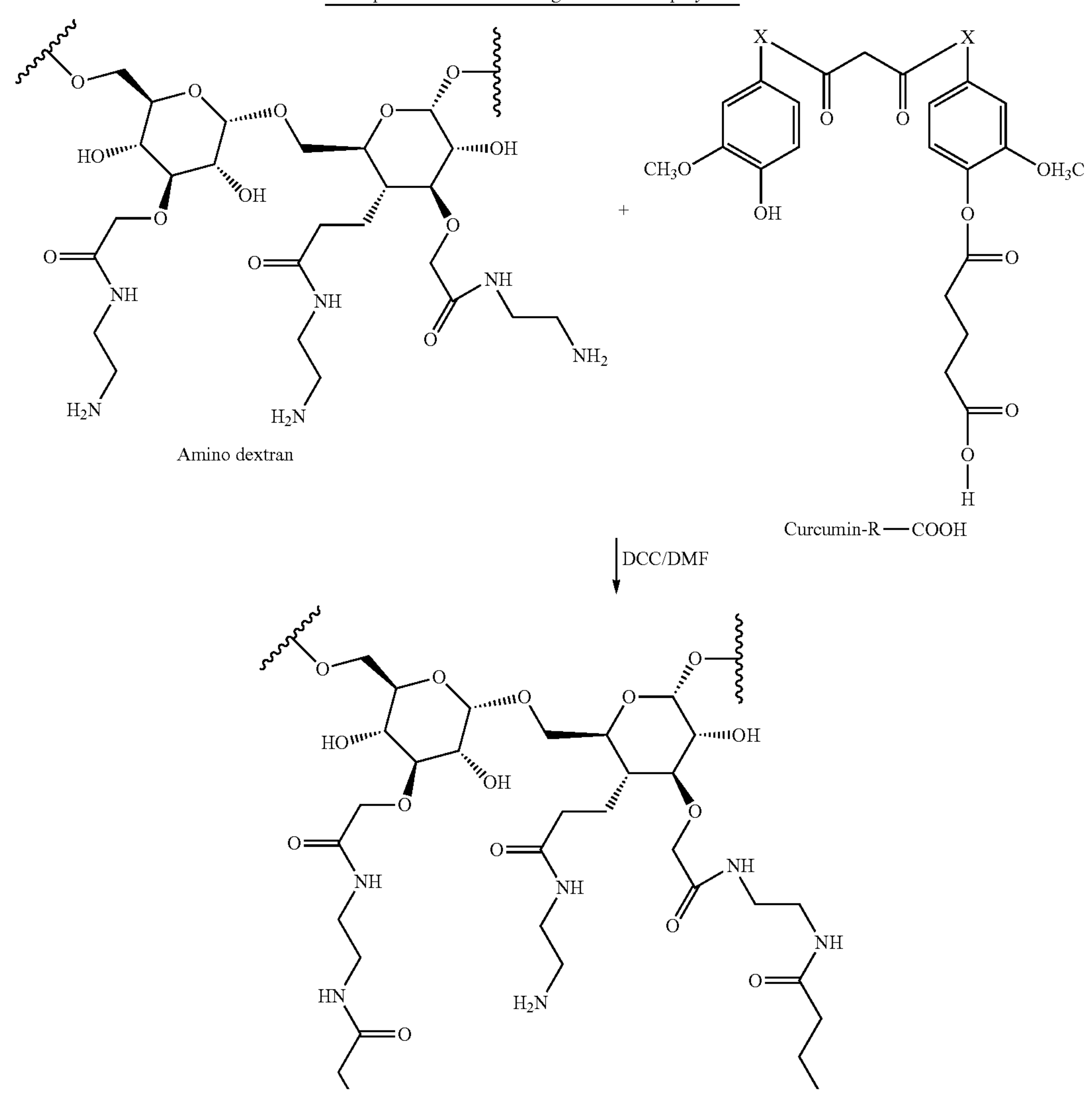
Scheme 4 Example of Curcumin Analog Modified Biopolymer
