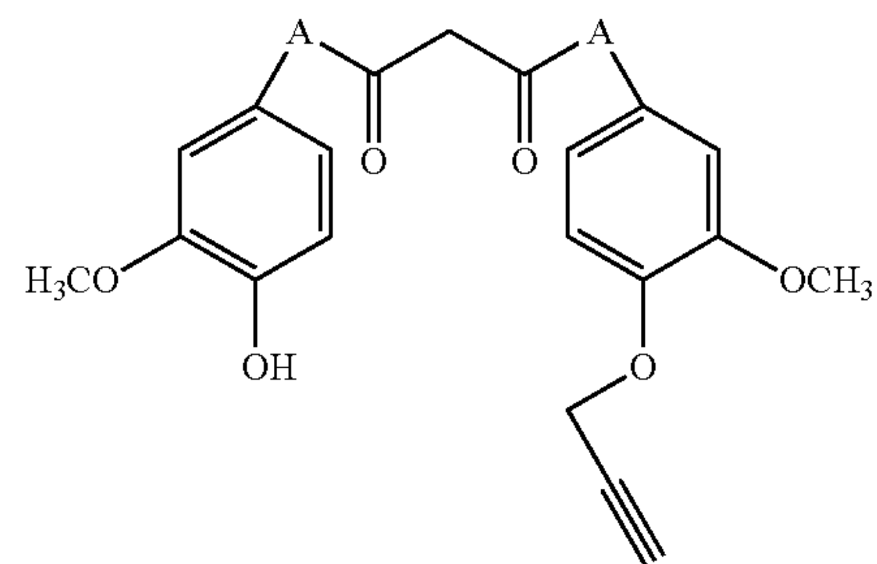
c) Curcumin alkyne
