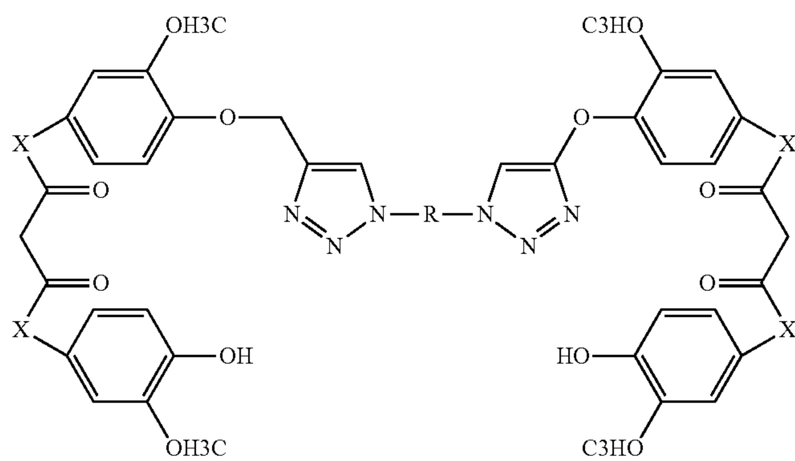
Curcumin Alkyne based Symmetric Dimer
