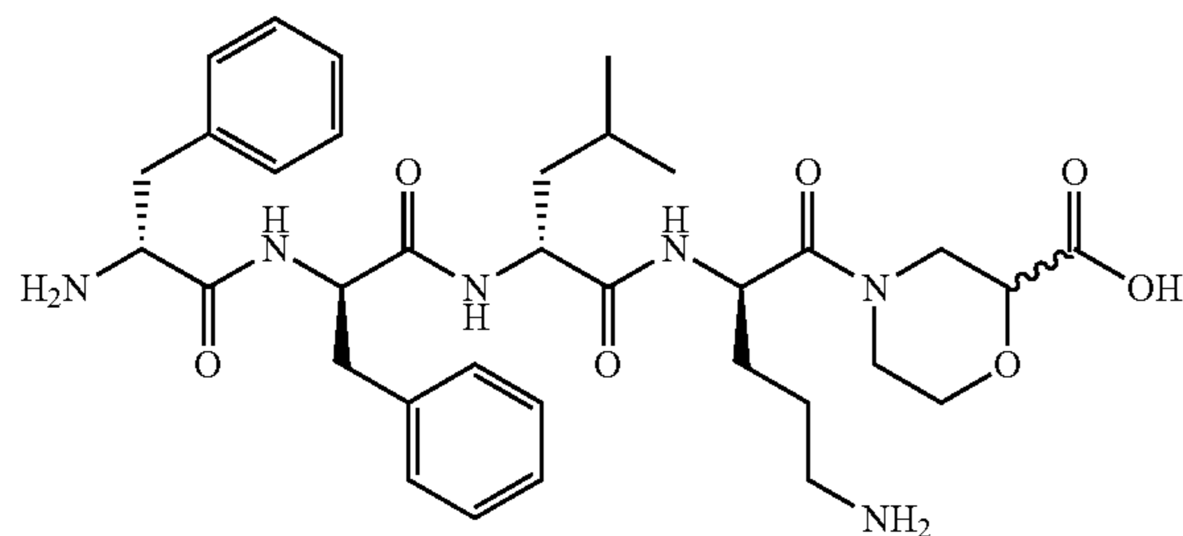
Synthesis of Compounds (91)-(103)
