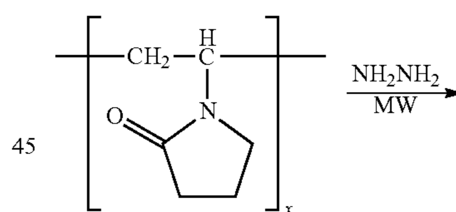
Scheme 2 Polyvinylpyrrolidone Synthesis
