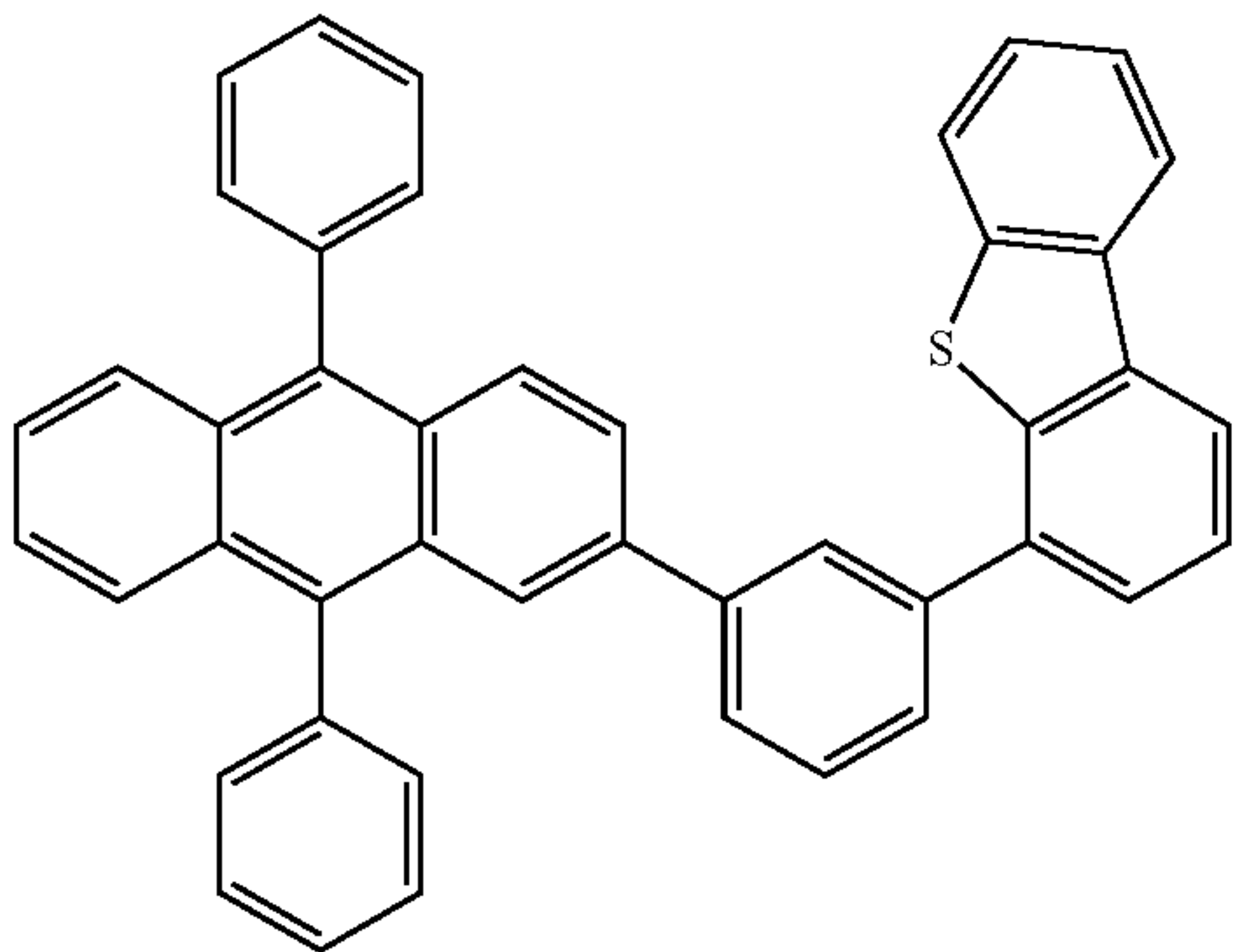
(2mPDBTPA-II)
