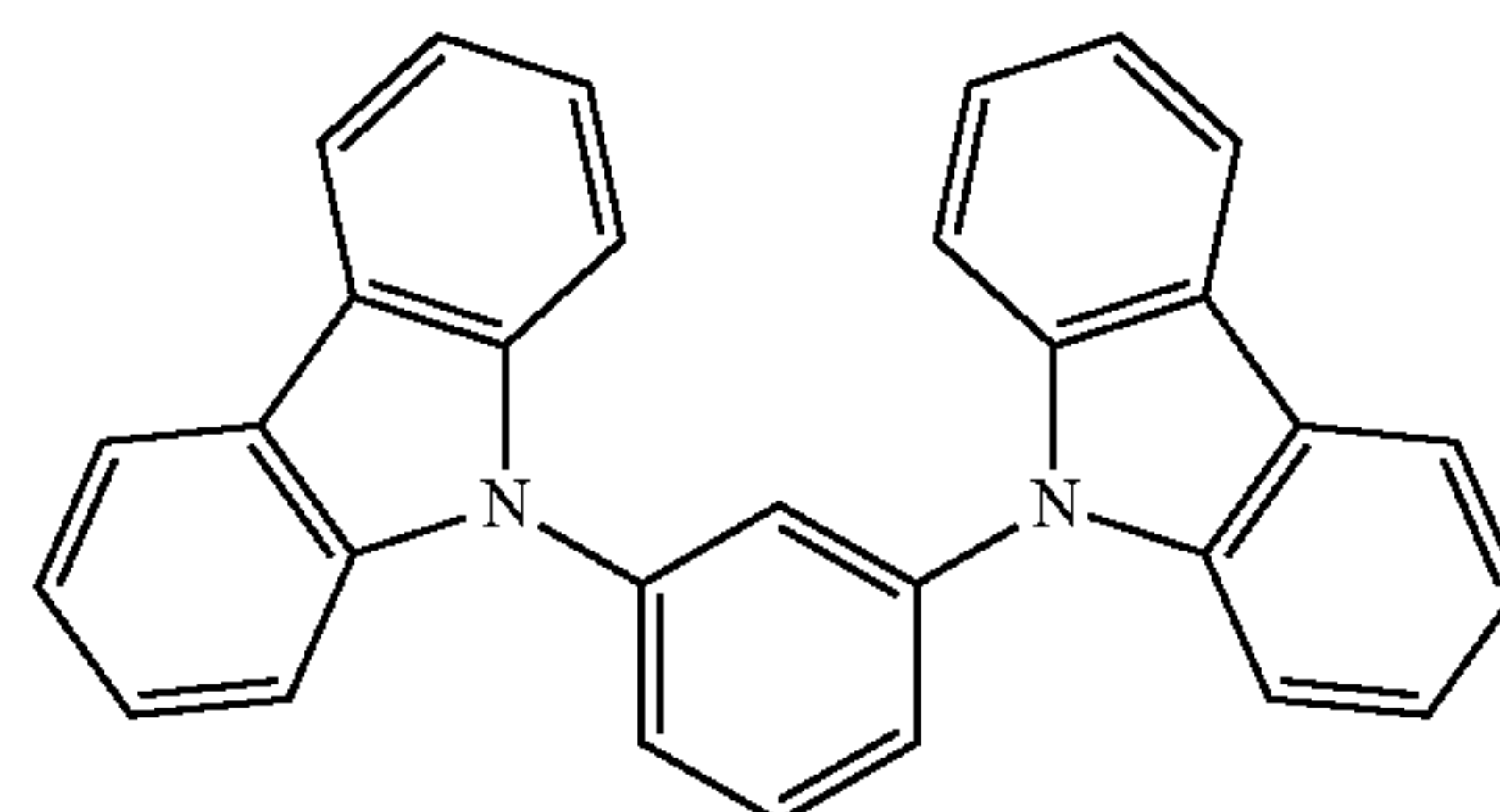
(mCP)
