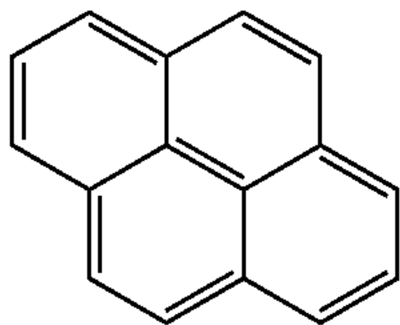
Pyrene
