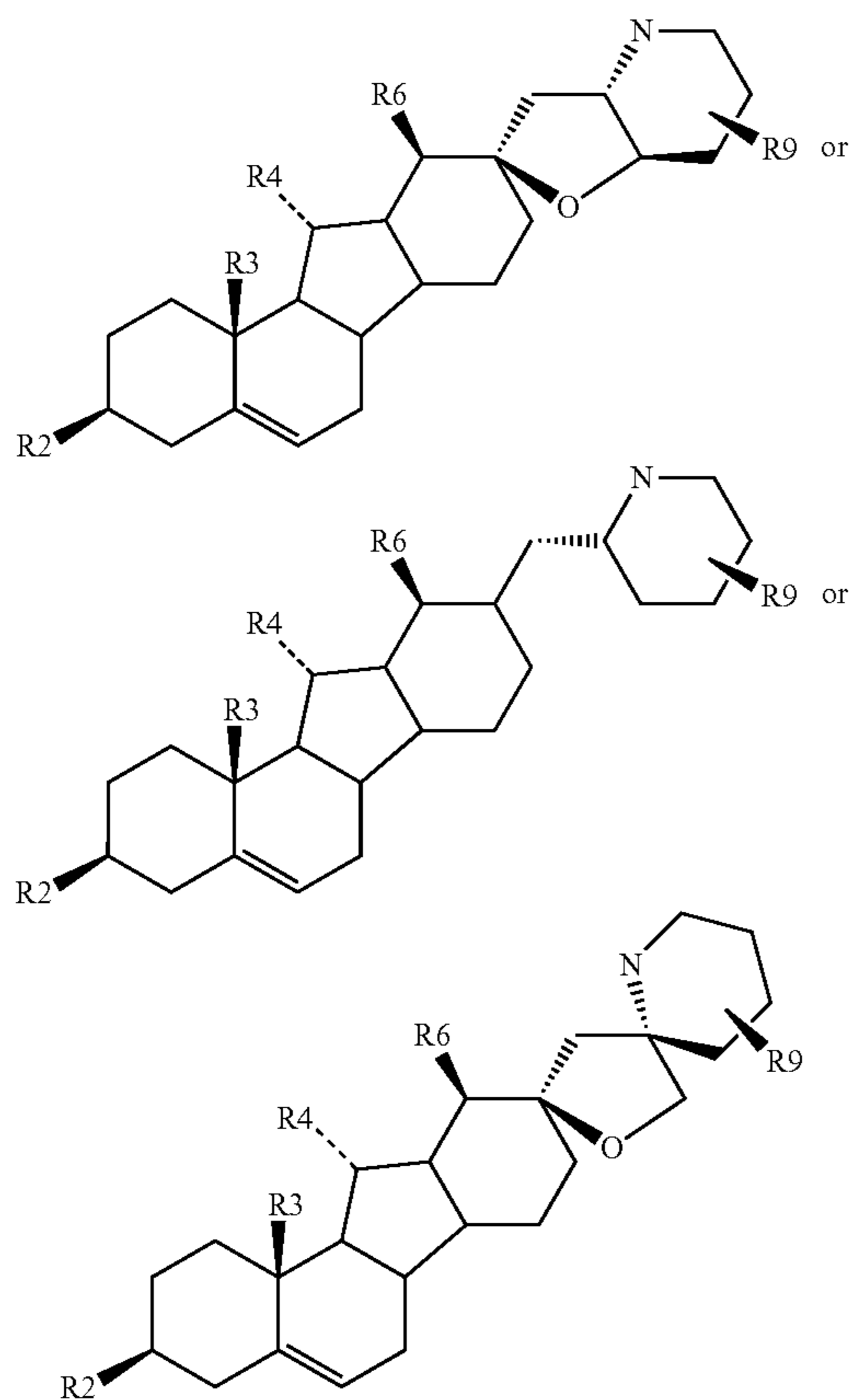
Formula XIIa
