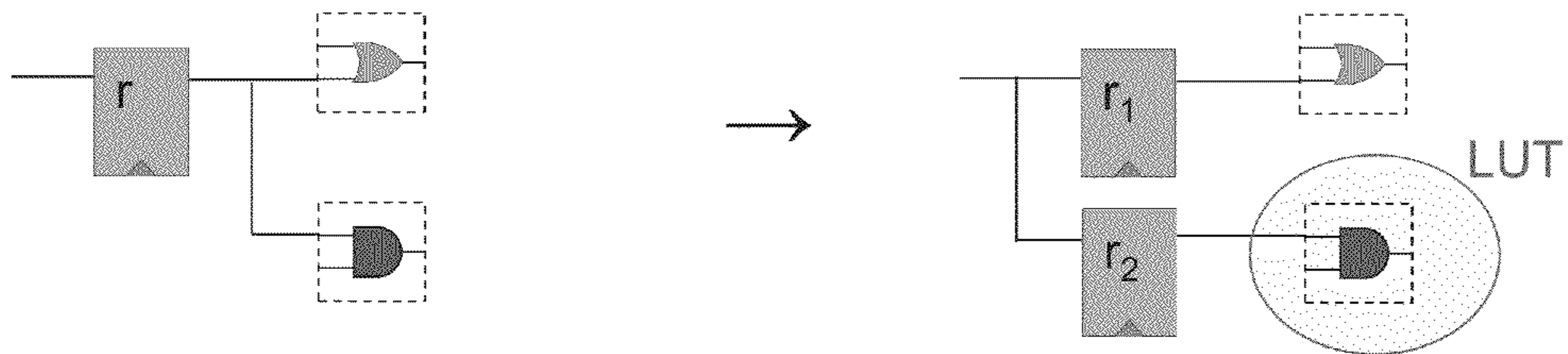
Extraction Netlist From 2 nd Compilation
