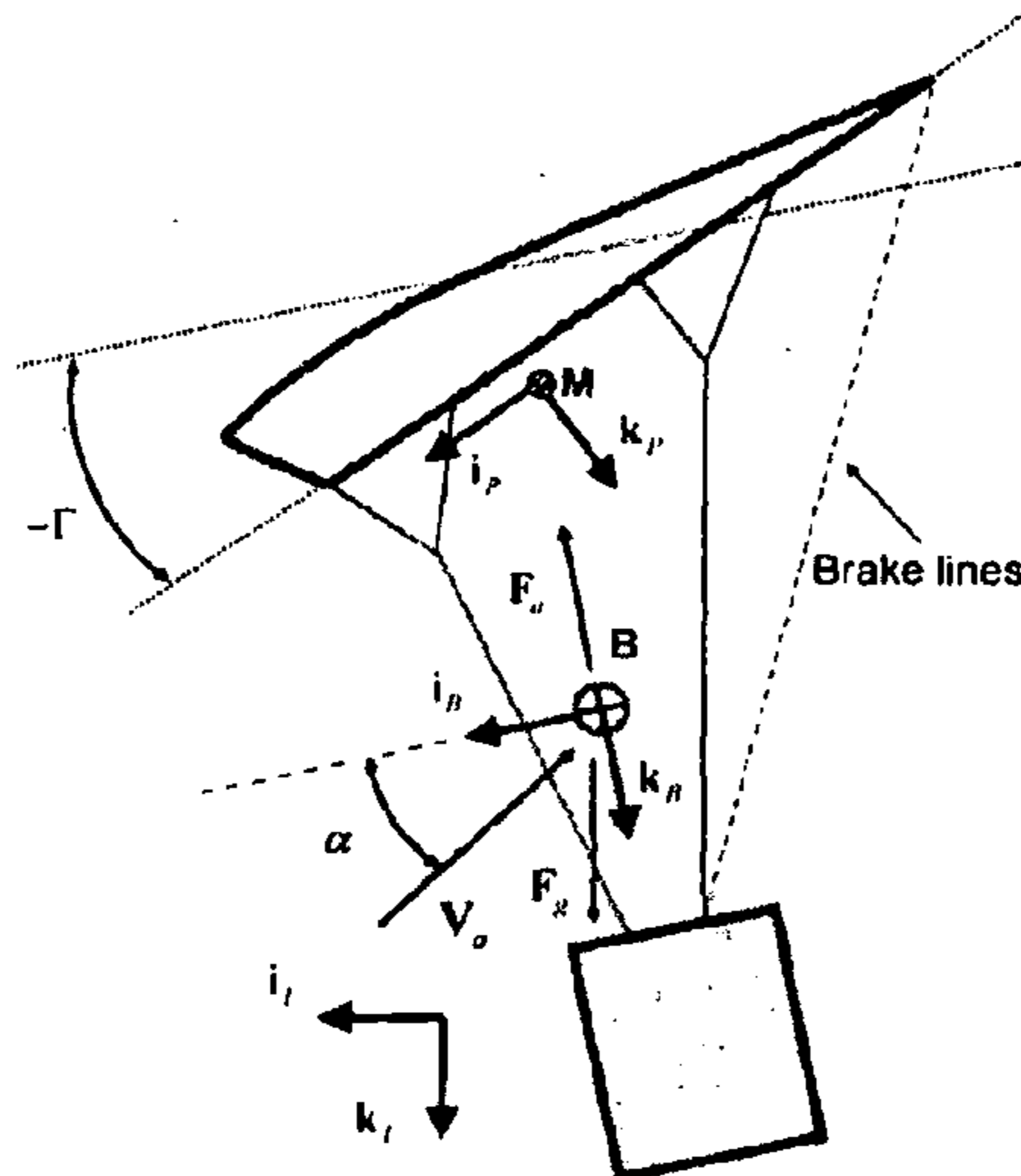
Fig. A A generic 6-DoF parafoil-payload system.
