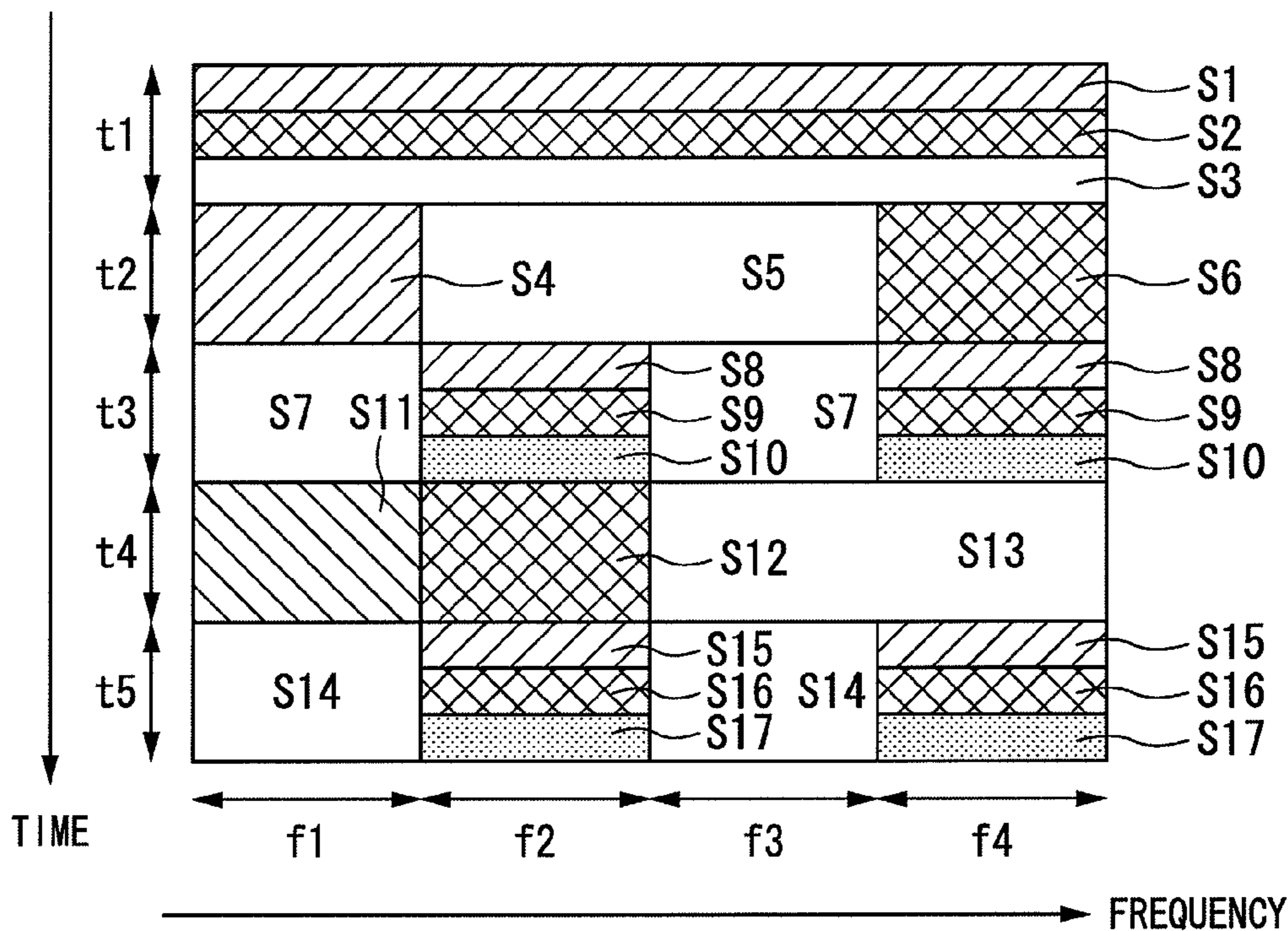
FIG. 32 CONVENTIONAL ART
