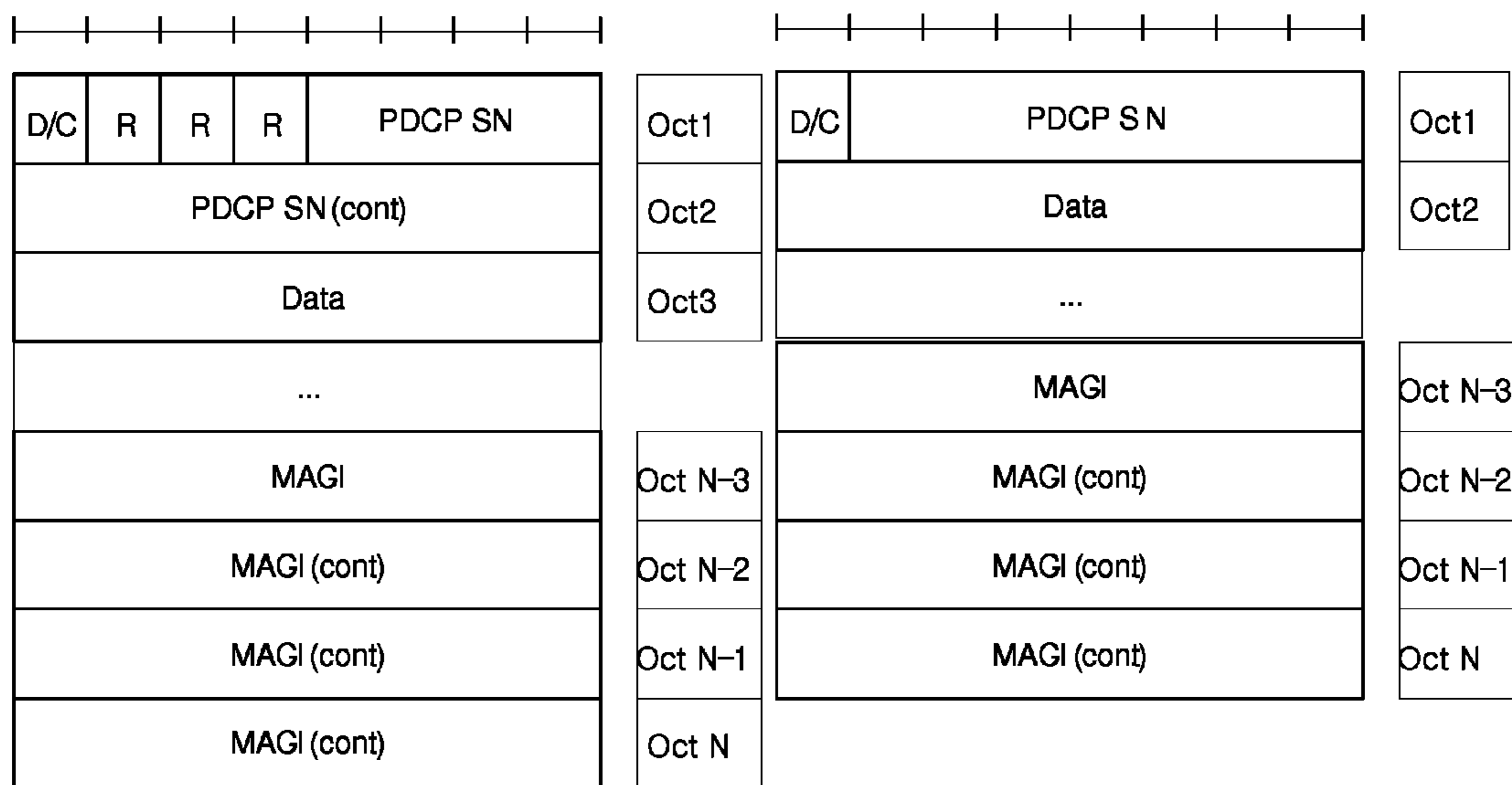
(a) Using 12 bits PDCP SN
