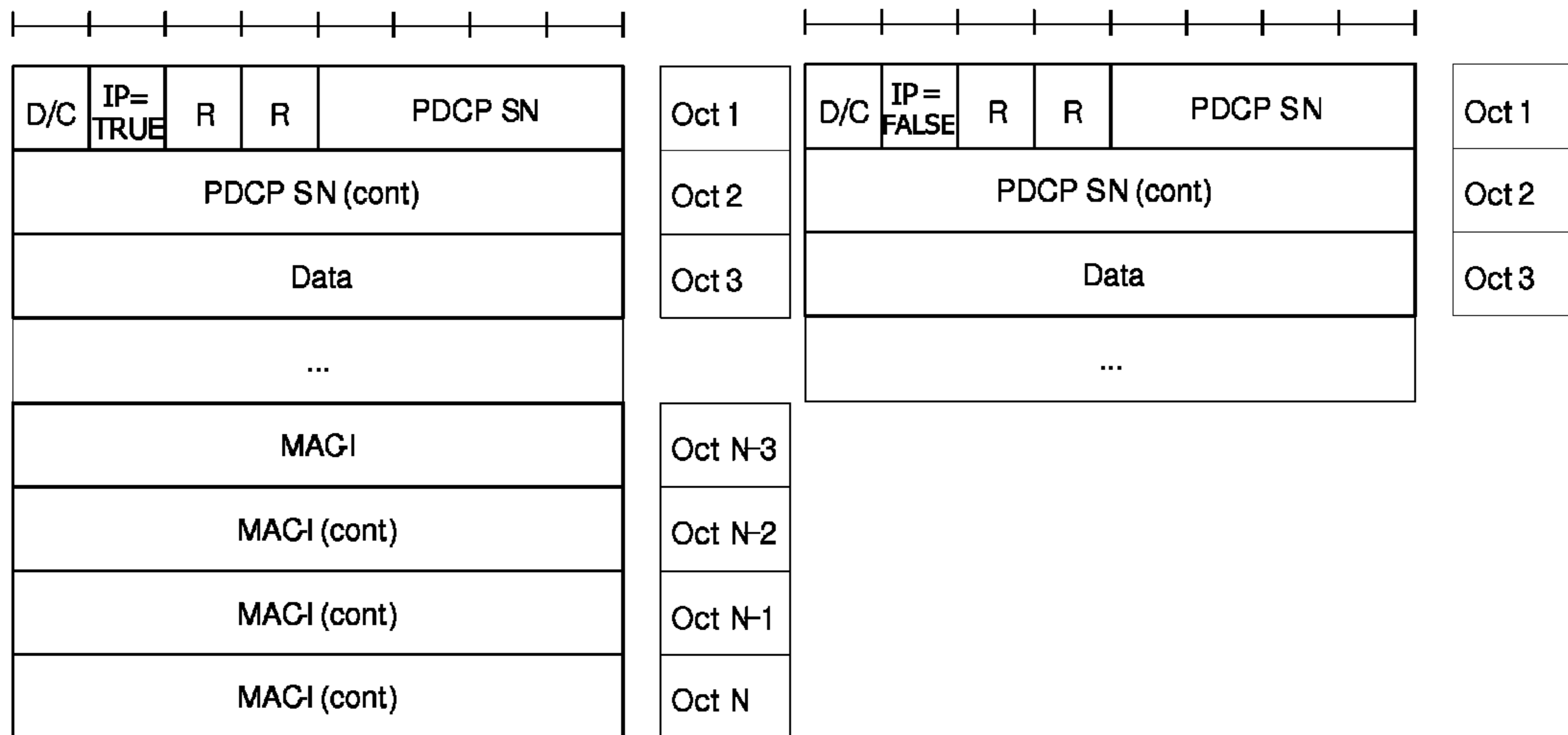
(a) PDCP Data PDU with MAC-I
