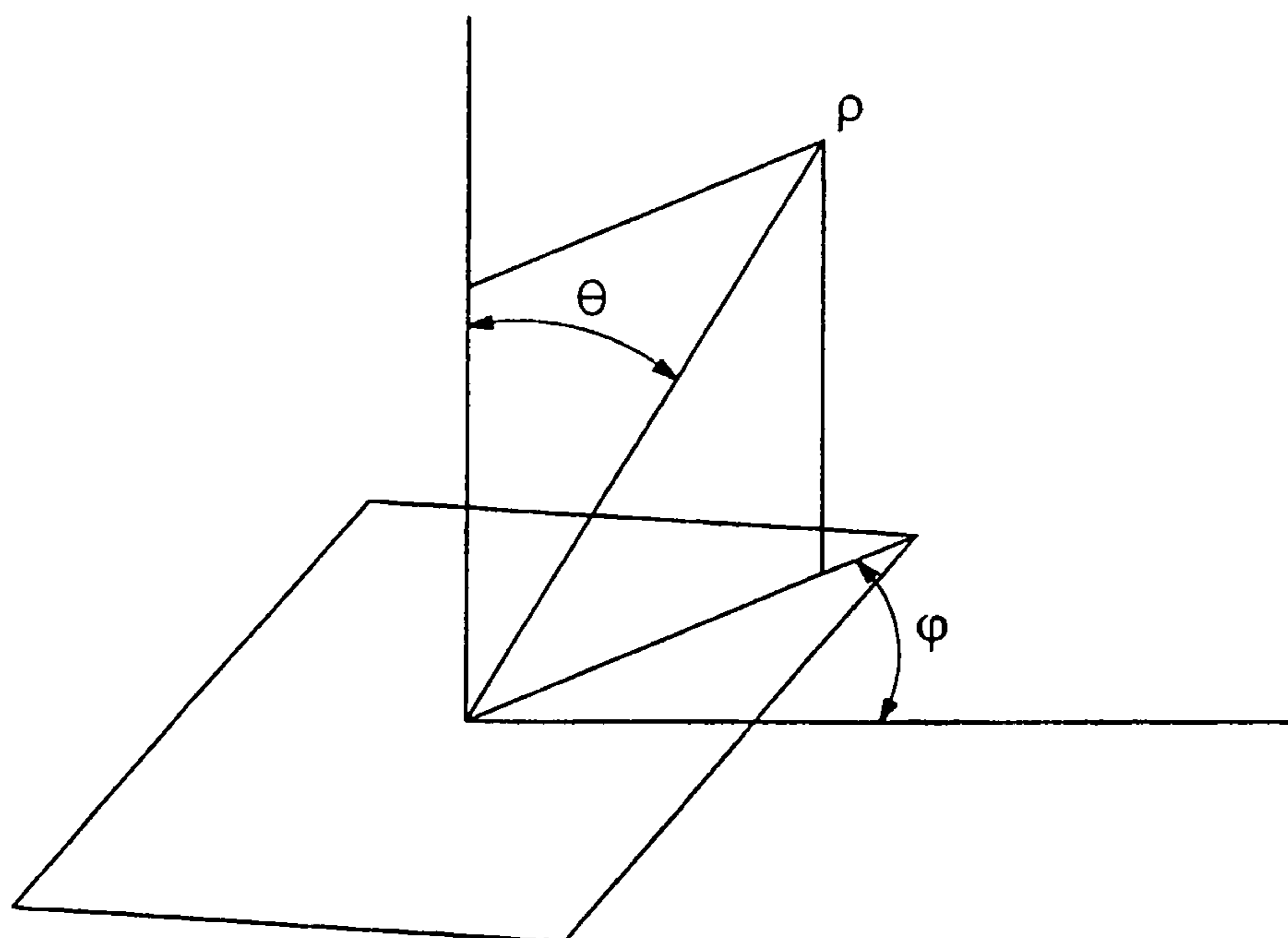
SPHERICAL SYSTEM OF COORDINATES
