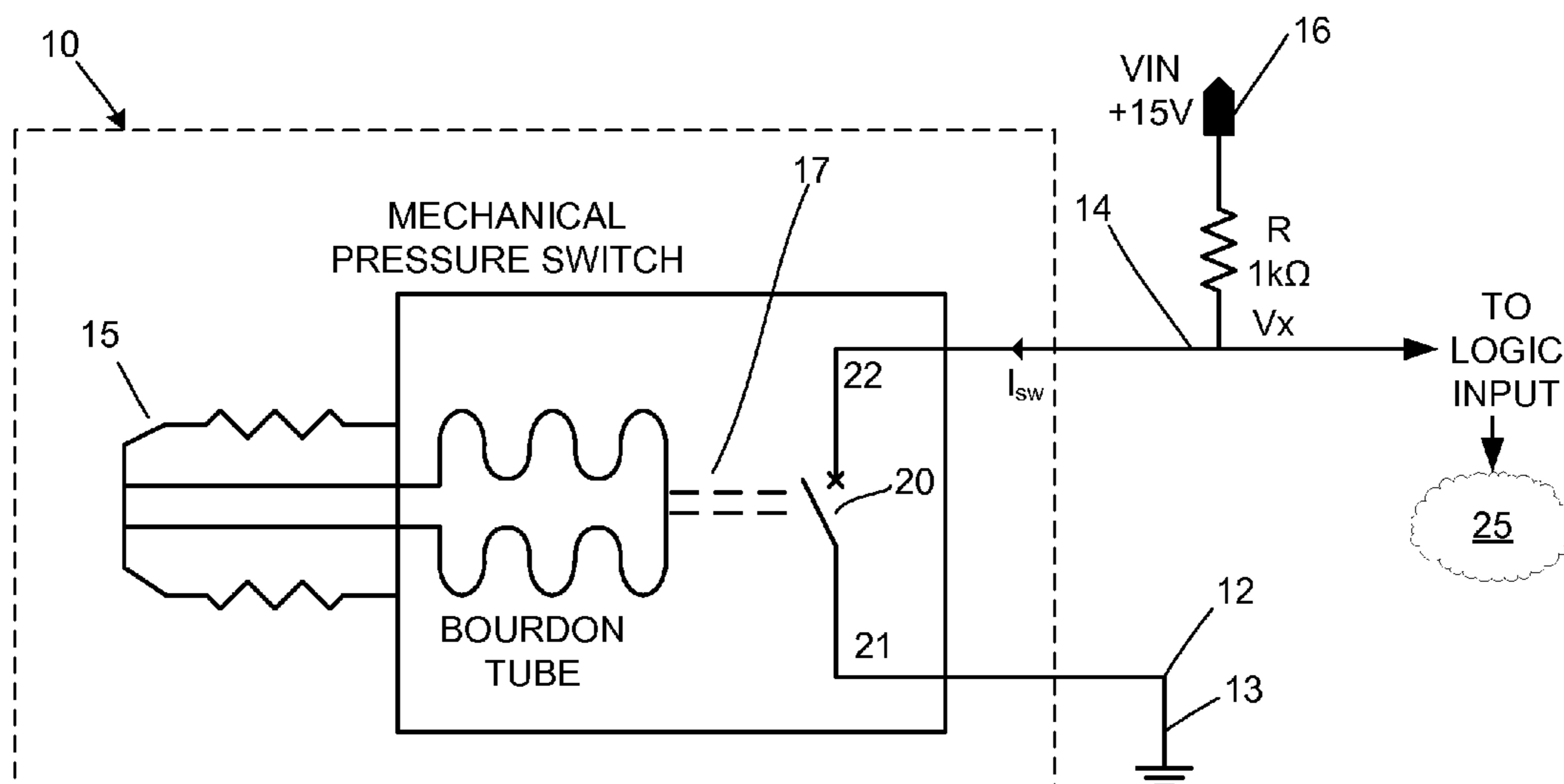
Fig. 1 PRIOR ART
