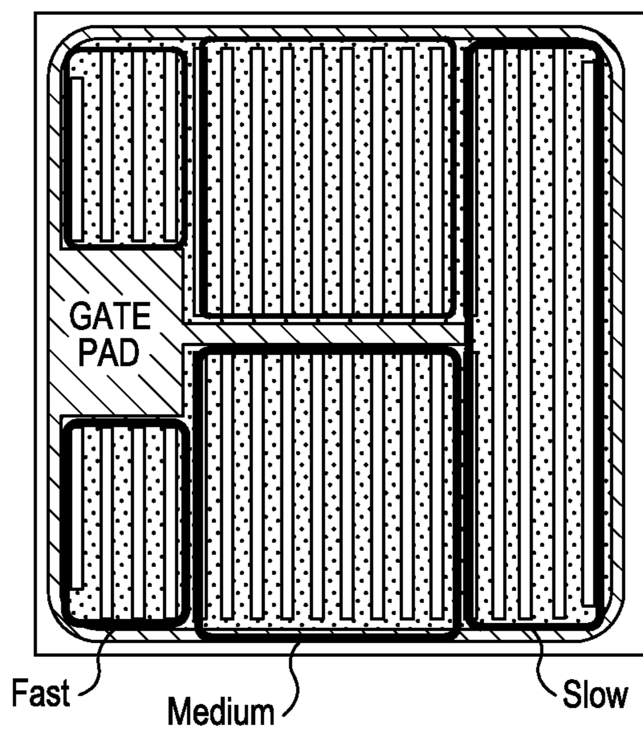
FIG. 9 PRIOR ART
