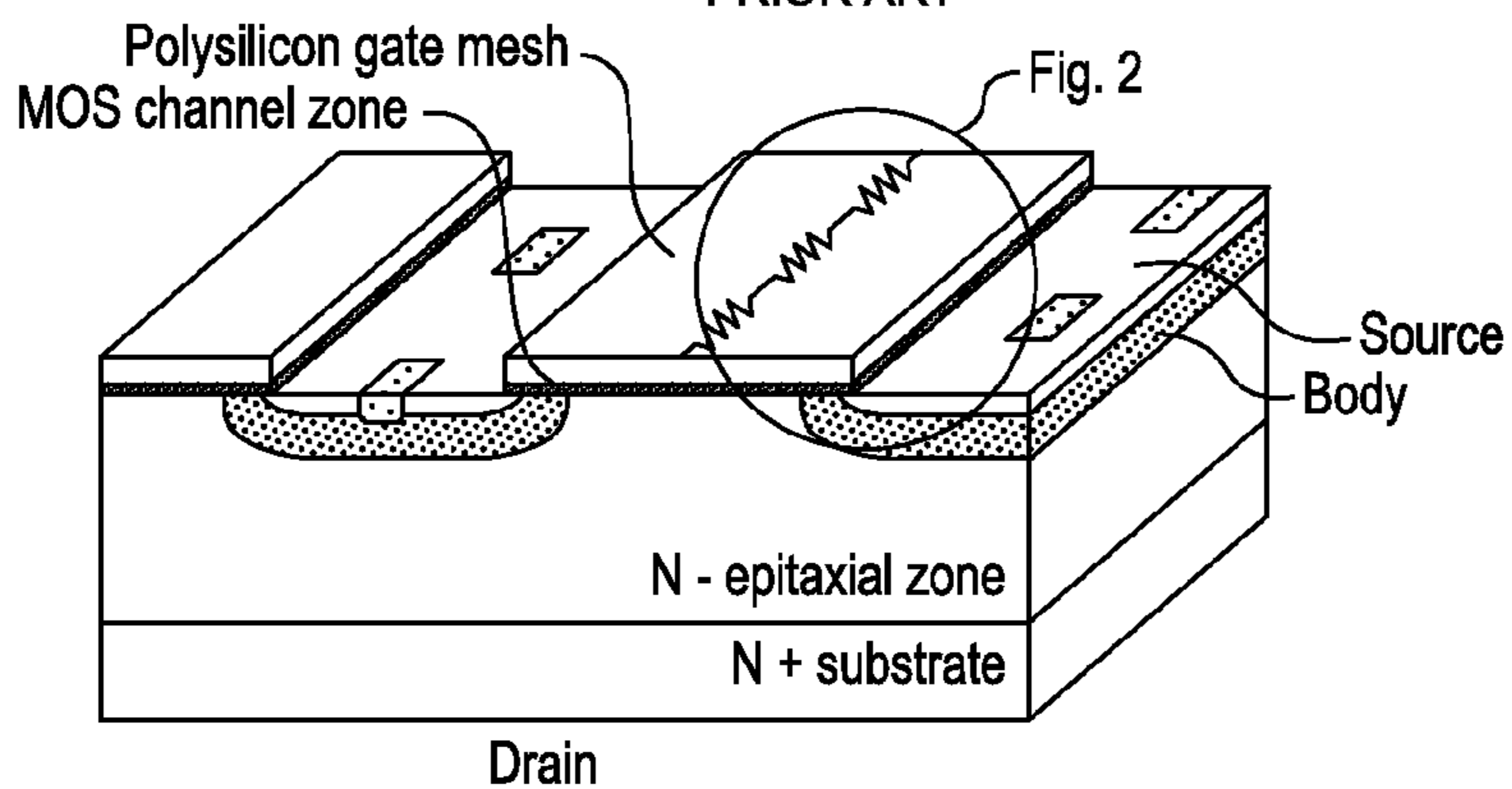
FIG. 1 PRIOR ART
