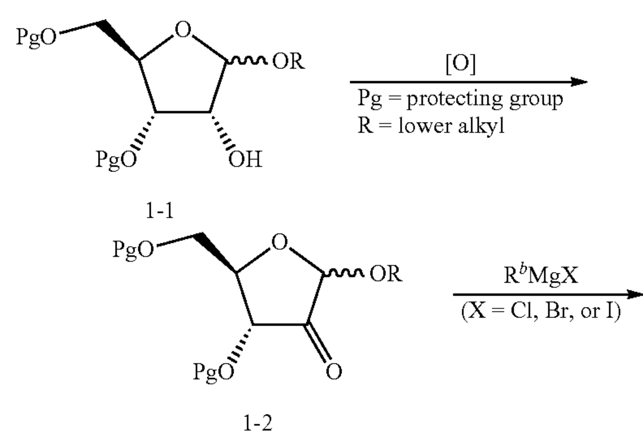
Scheme 1
