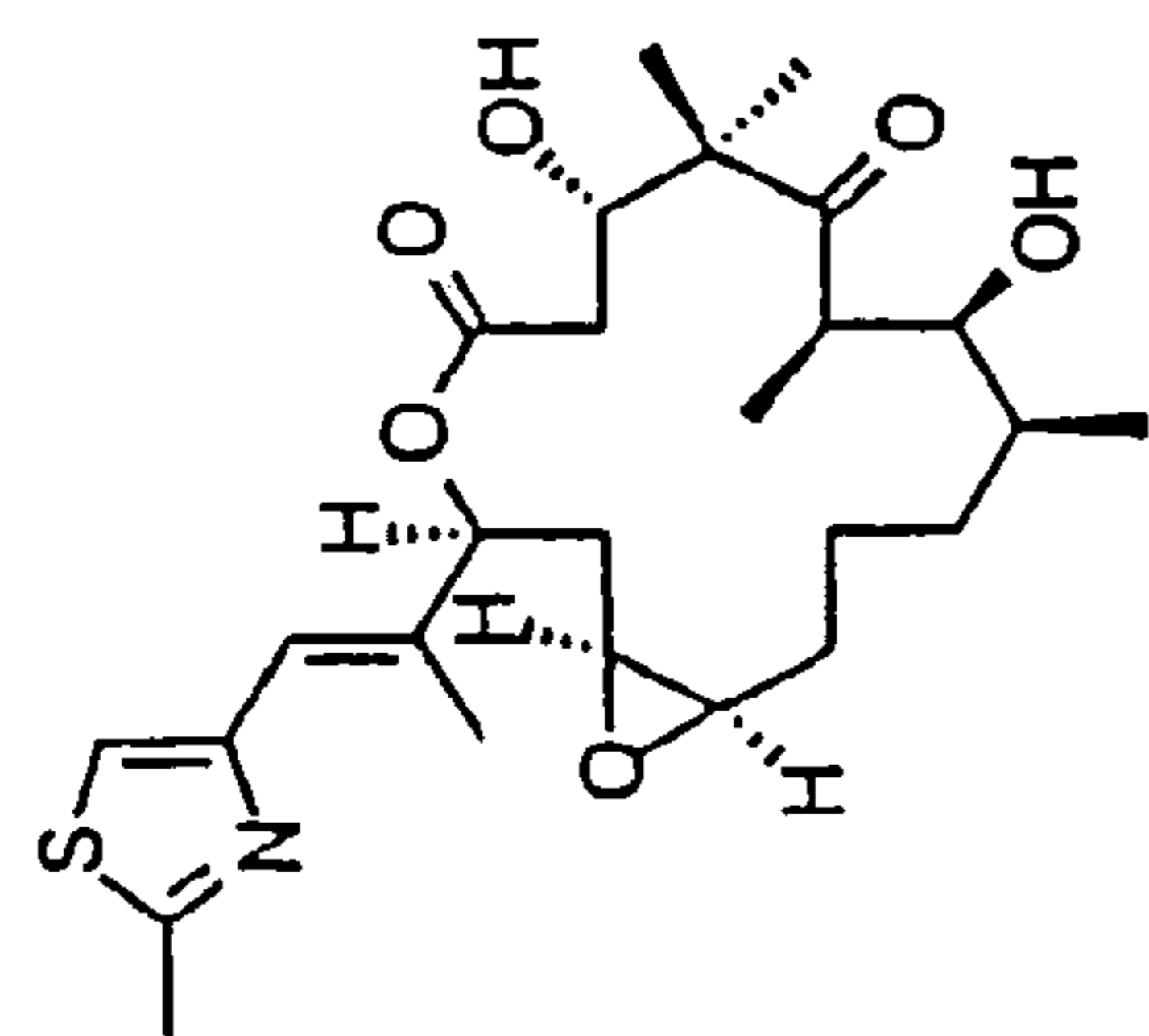
epothilone A
