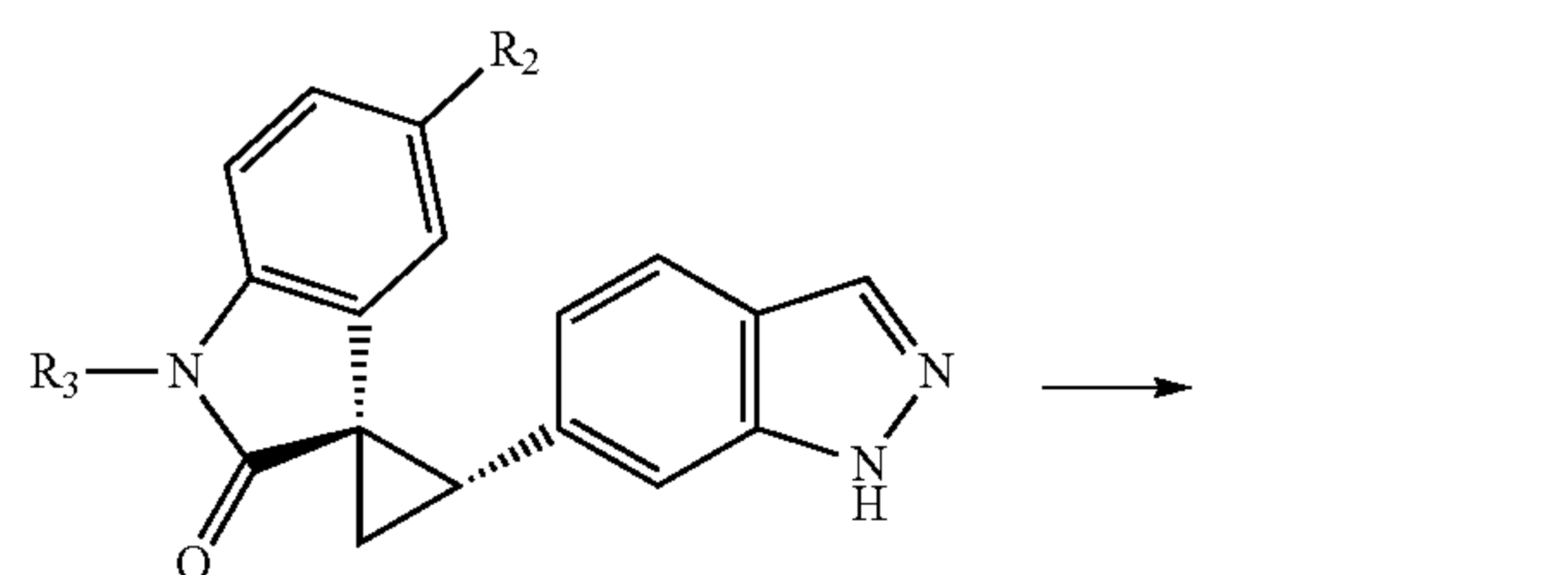
SCHEME 7
