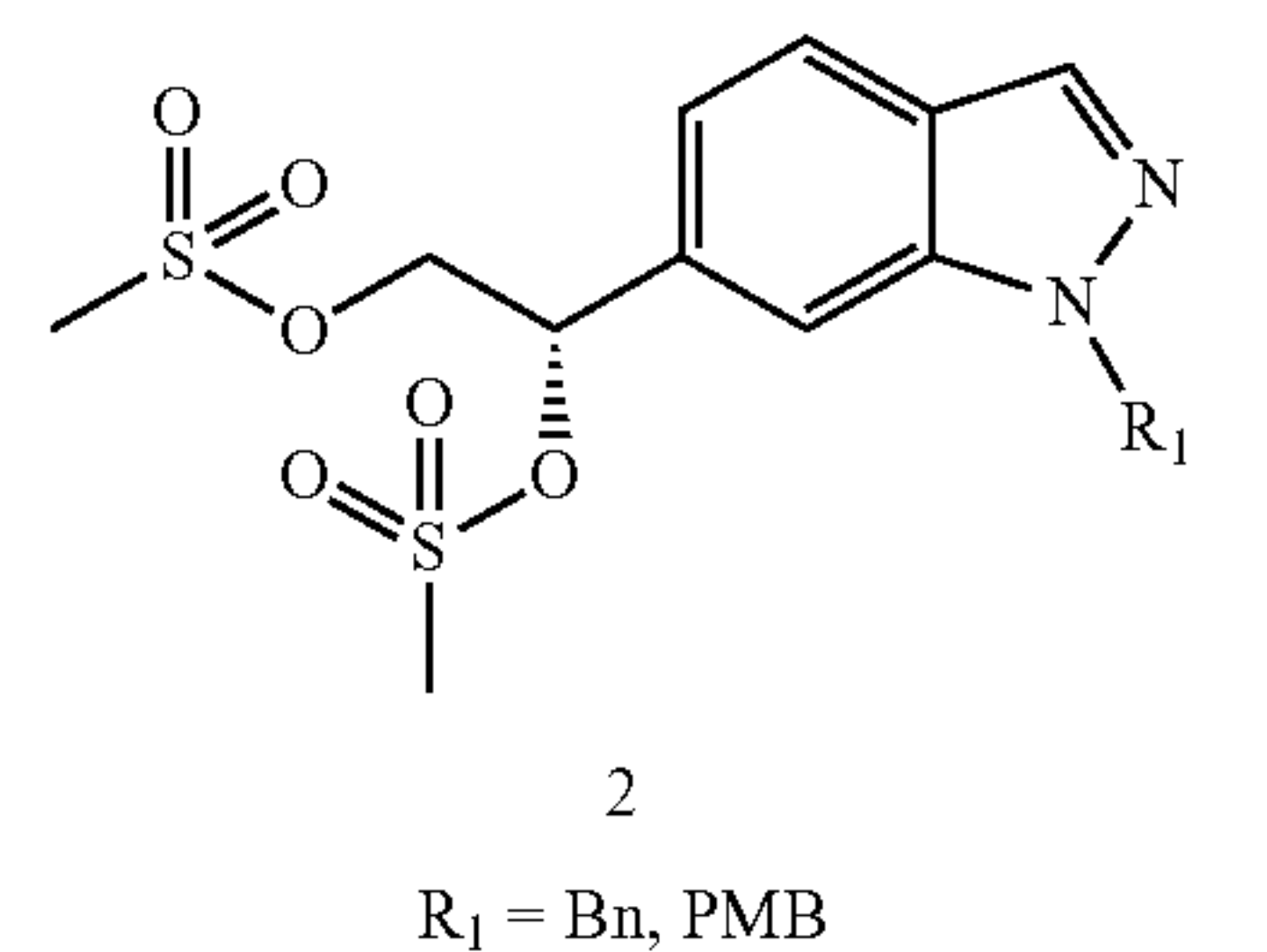
SCHEME 5
