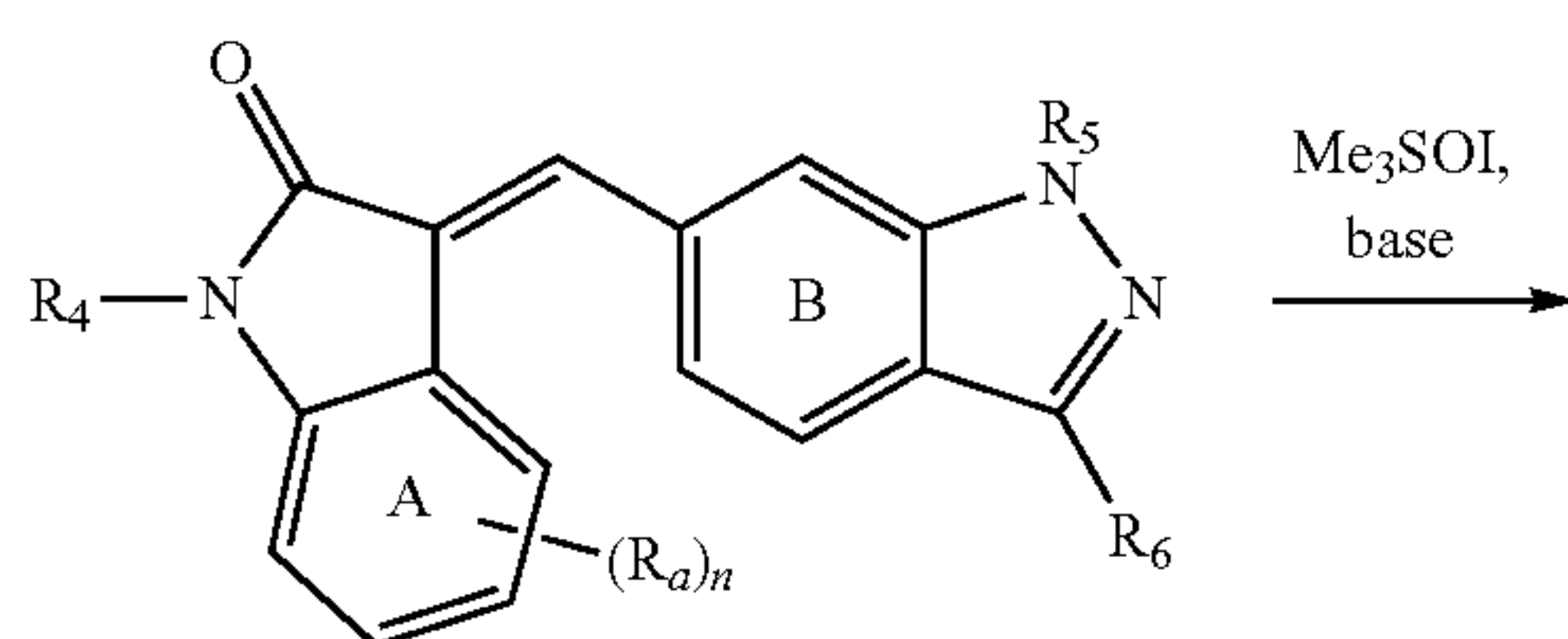
SCHEME 4
