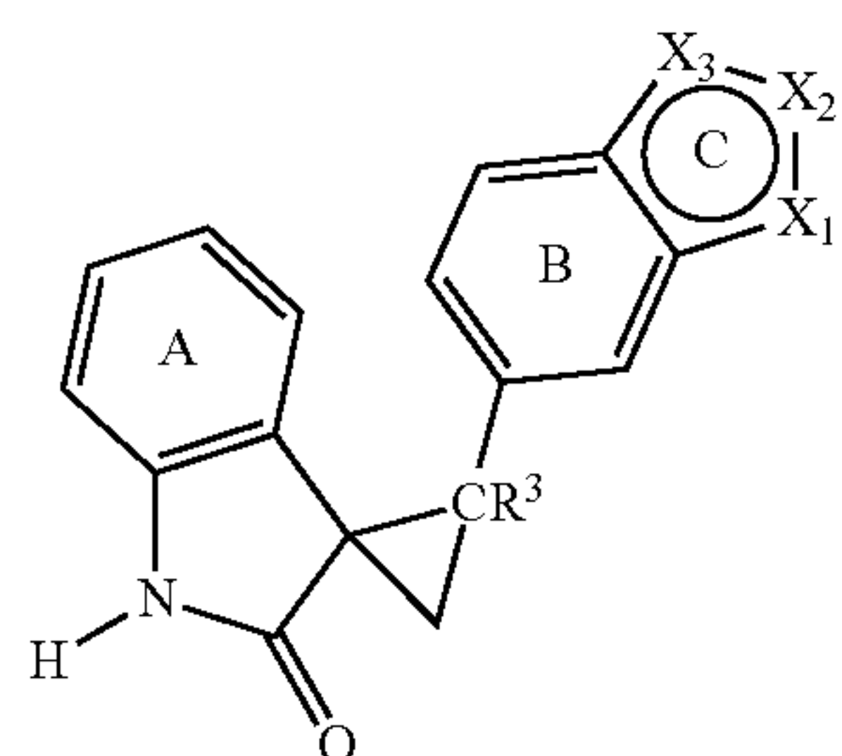
(indolinone form)
