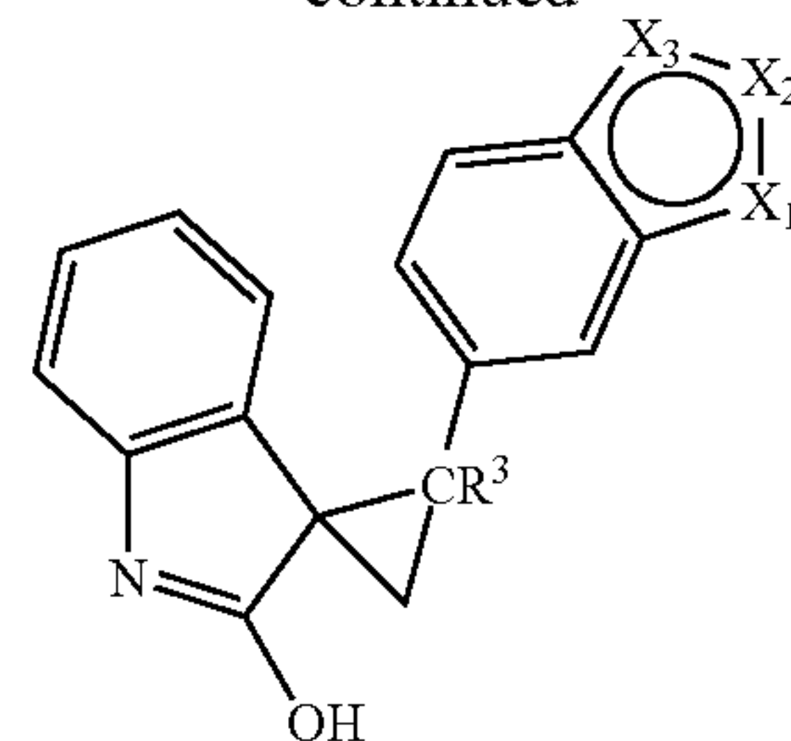
(indolol form)
