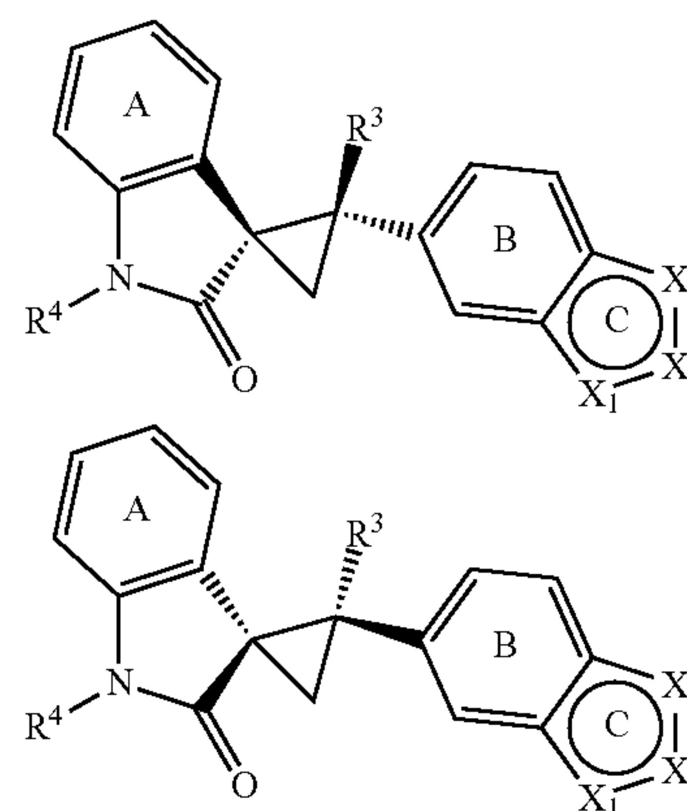
Ring A and Ring B are trans.
