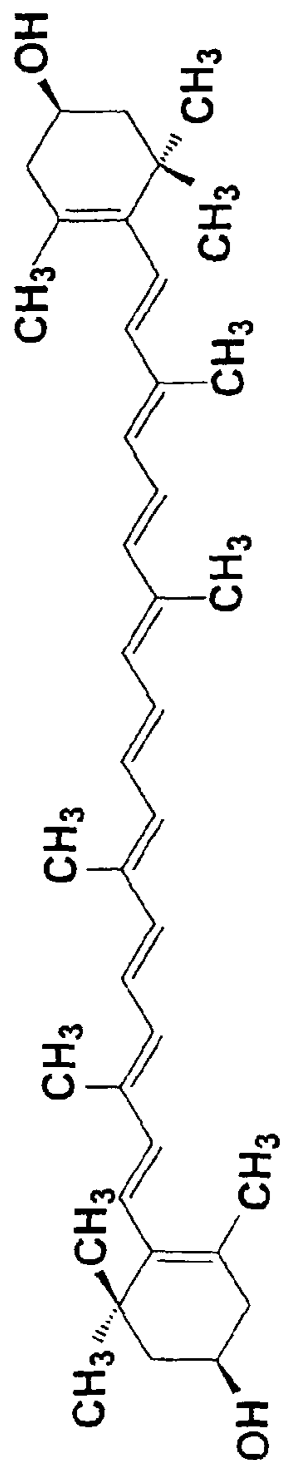
Zeaxanthin
