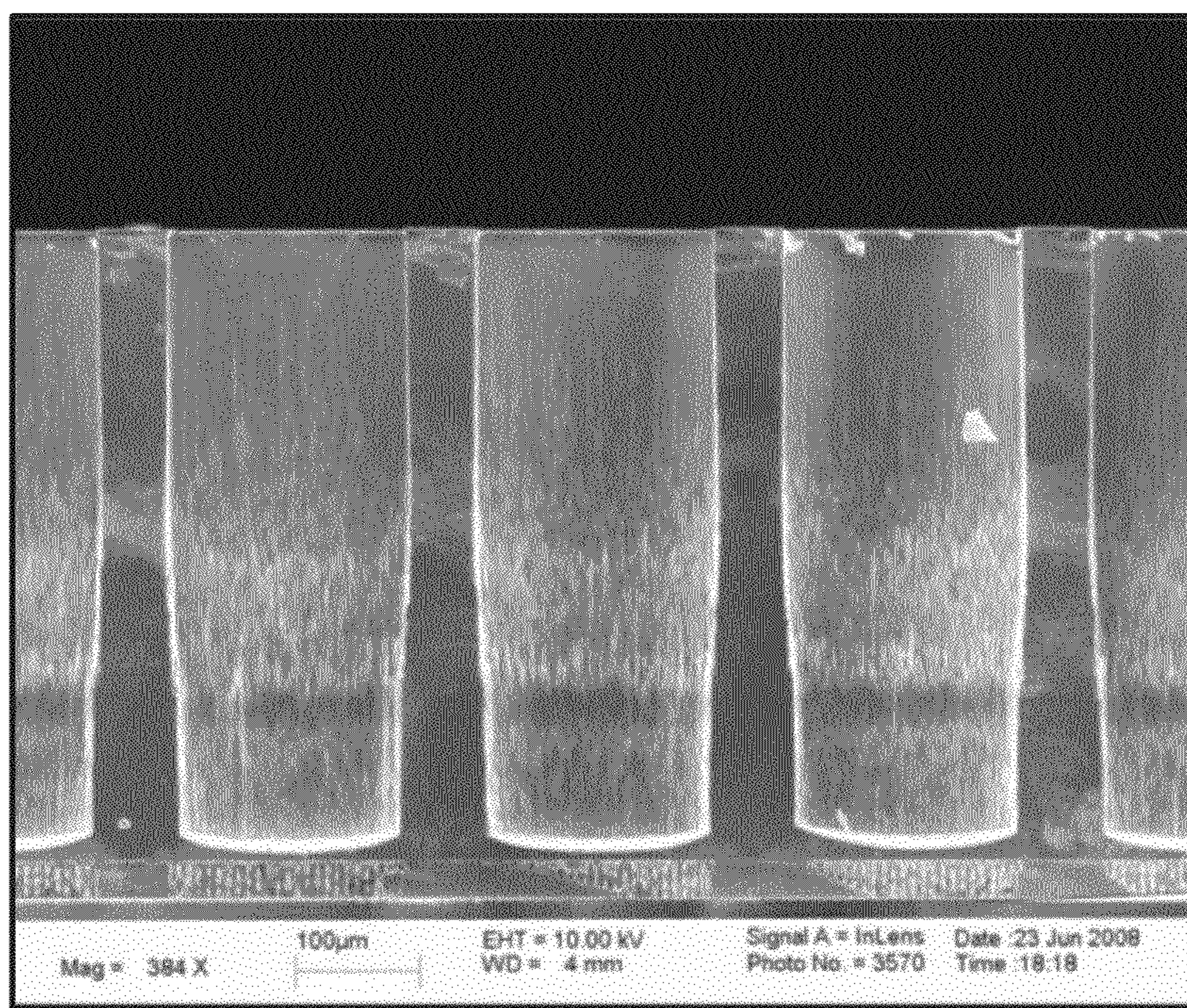
SEM image of deep etched 190µm x 190µm openings.
