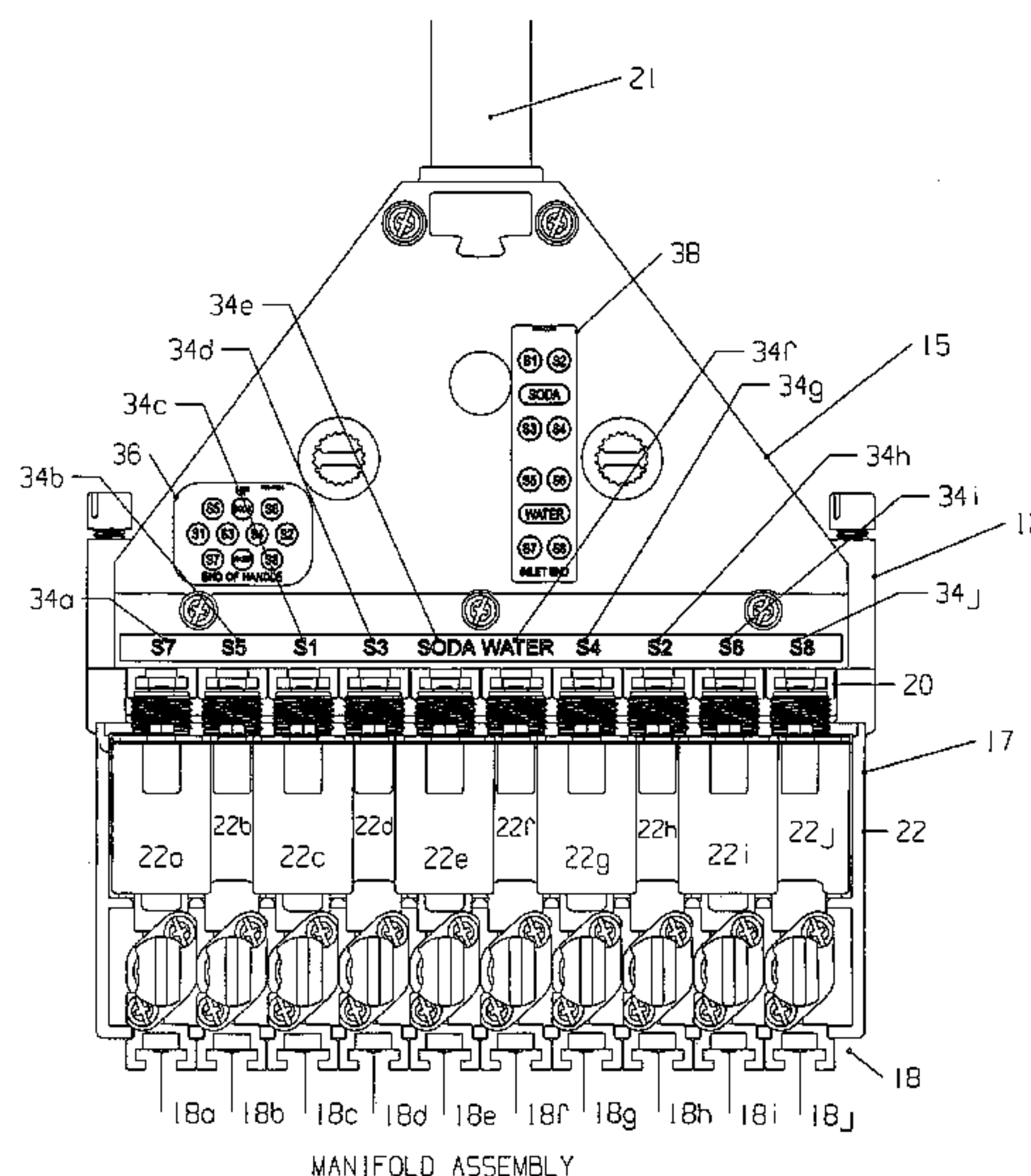
MANIFOLD ASSEMBLY
