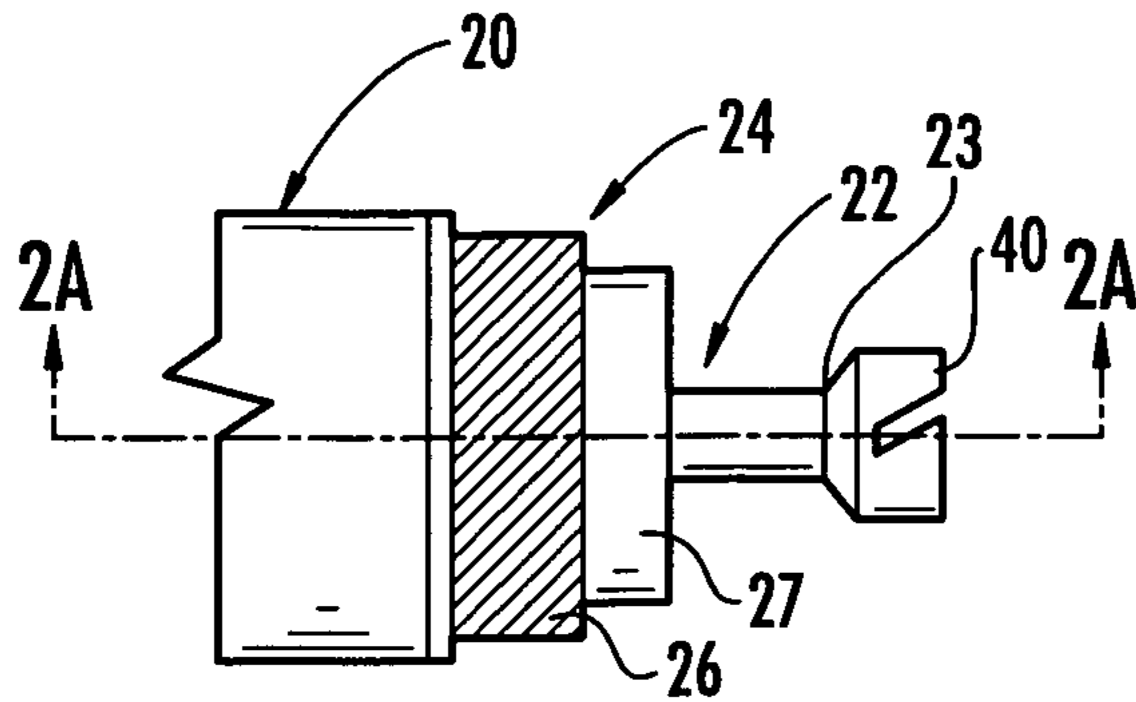
FIG. 1 (PRIOR ART)
