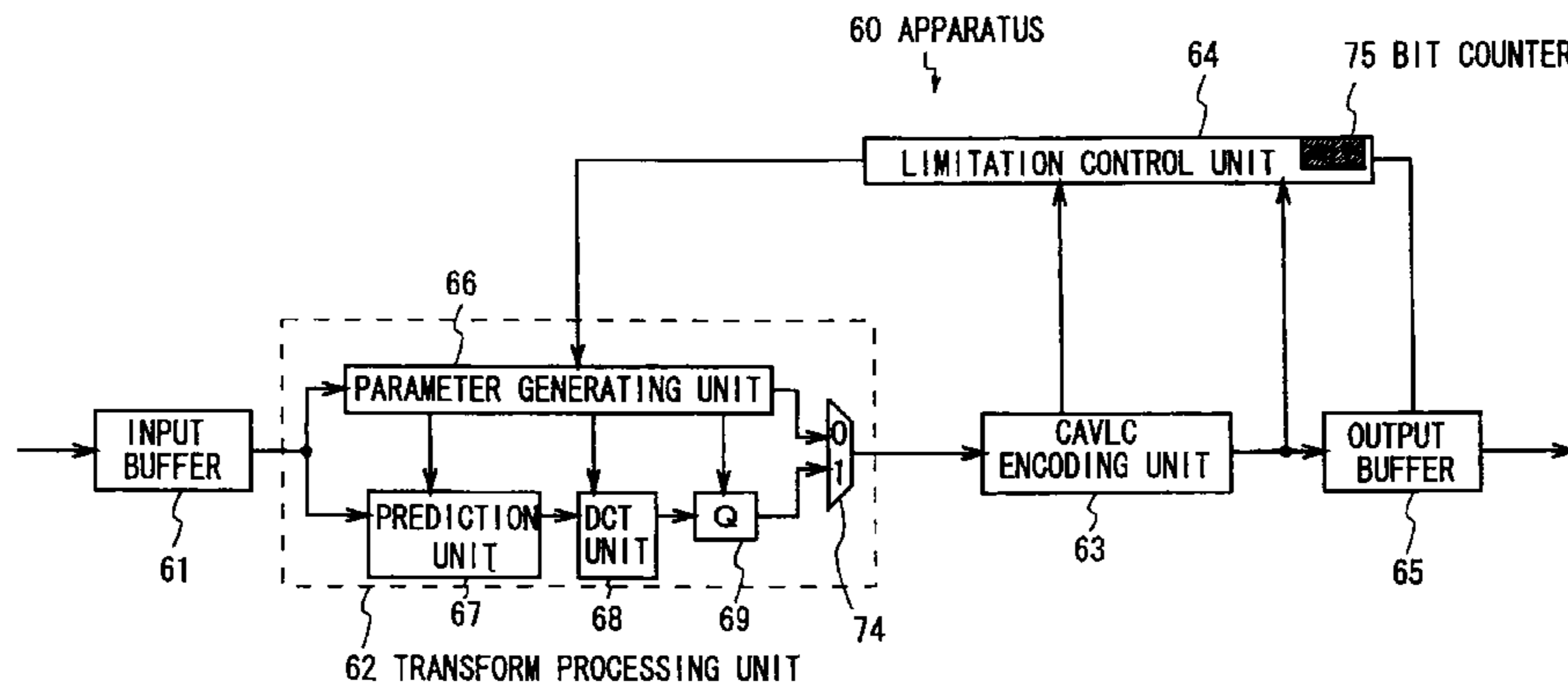
CONSTRUCTION OF VIDEO-INFORMATION ENCODING APPARATUS ACCORDING TO THIS INVENTION
