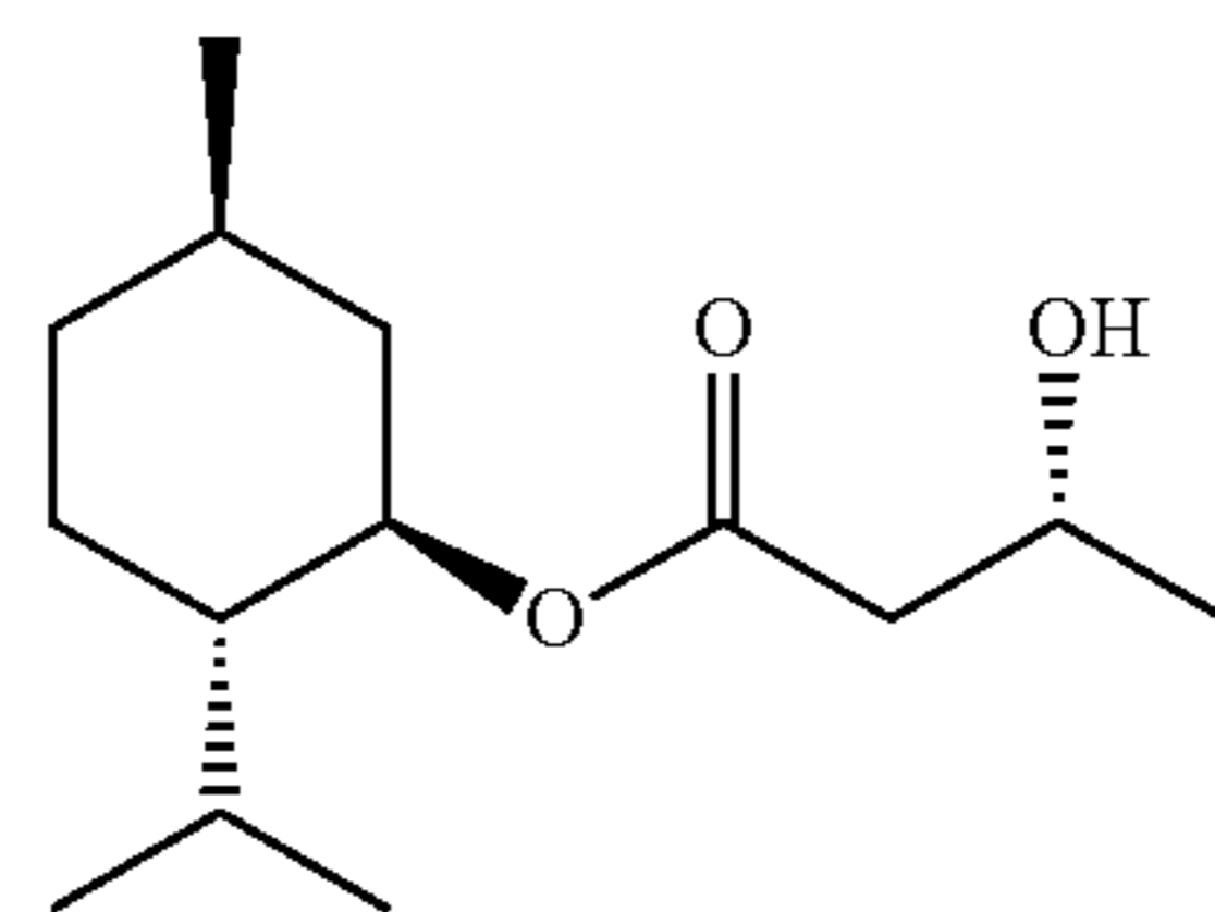
[Chem. 4]
