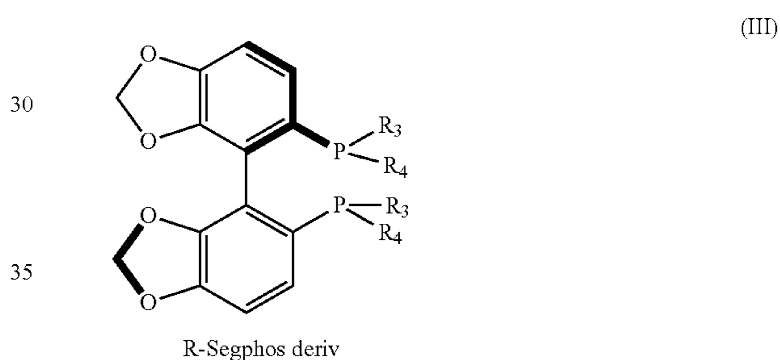
[Chem. 9]
