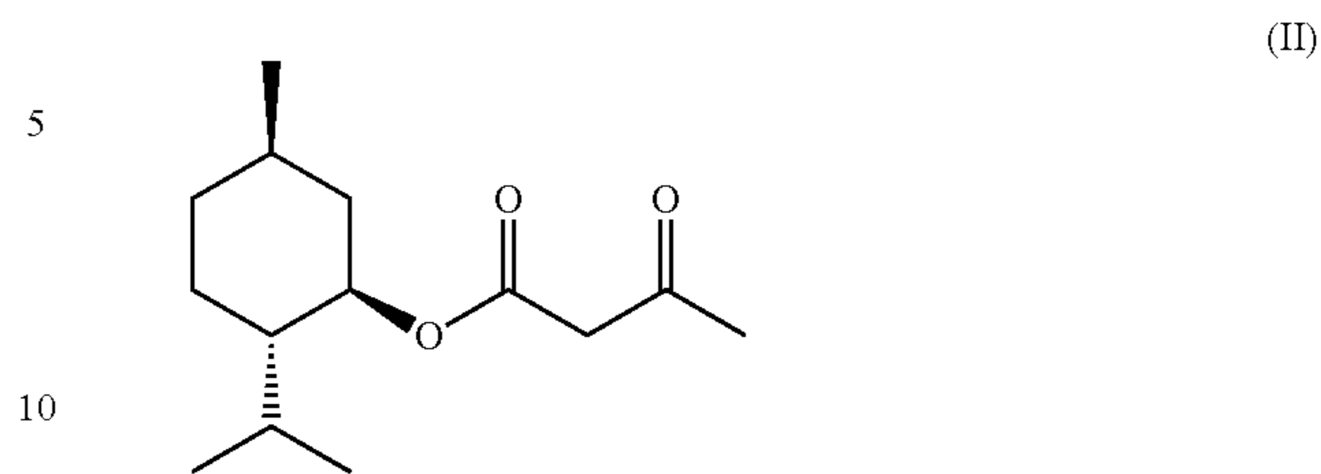
[Chem. 8]
