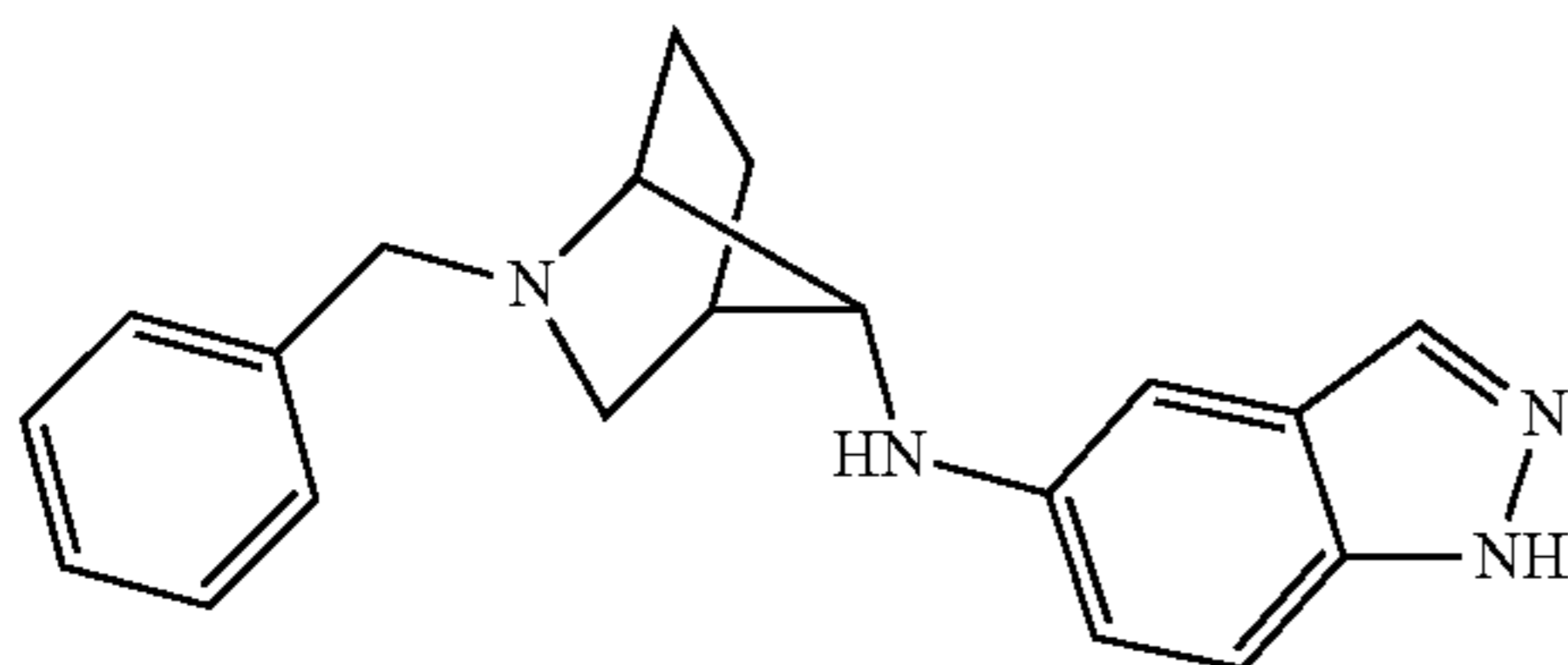
N-((1SR,4SR,7RS)-2-benzyl-2-azabicyclo[2.2.1]heptan-7-yl)-1H-indazol-5-amine, Compound 3.1.01
