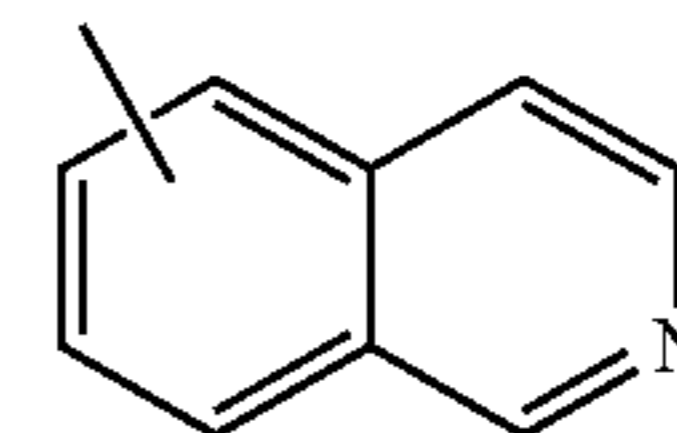
isoquinoline
