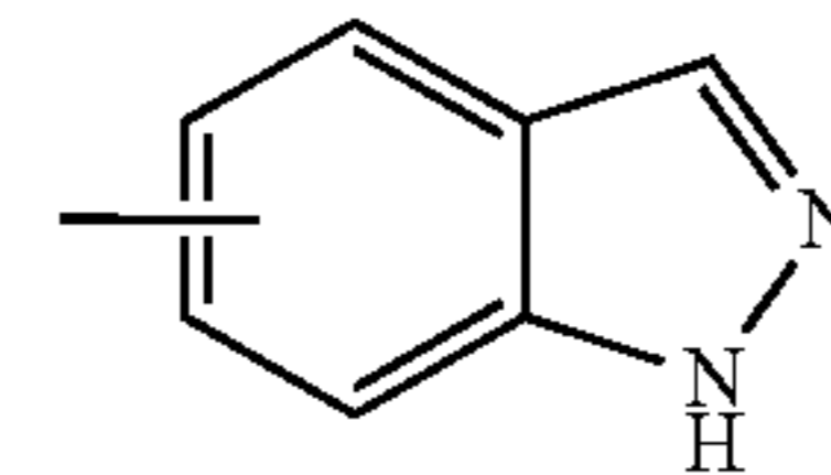
Indazole
