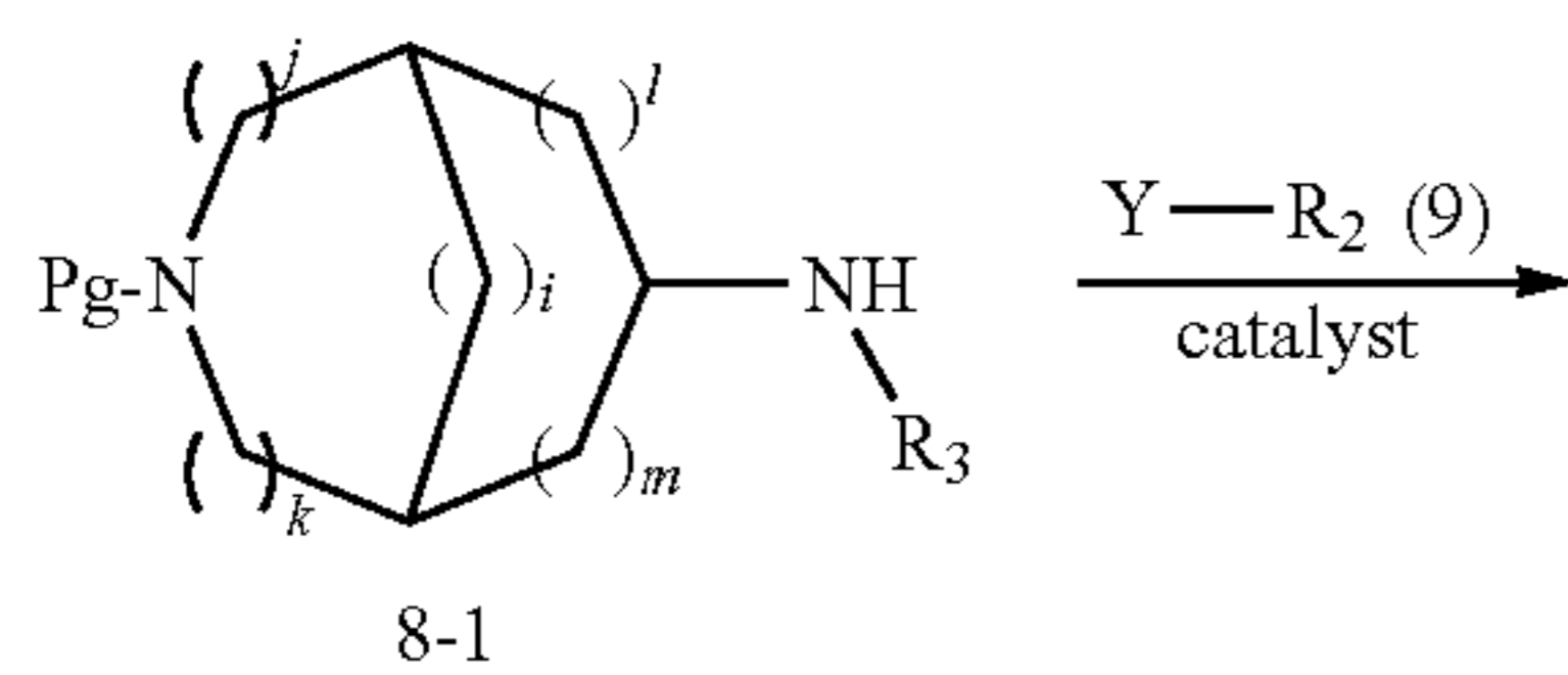
Scheme 2
