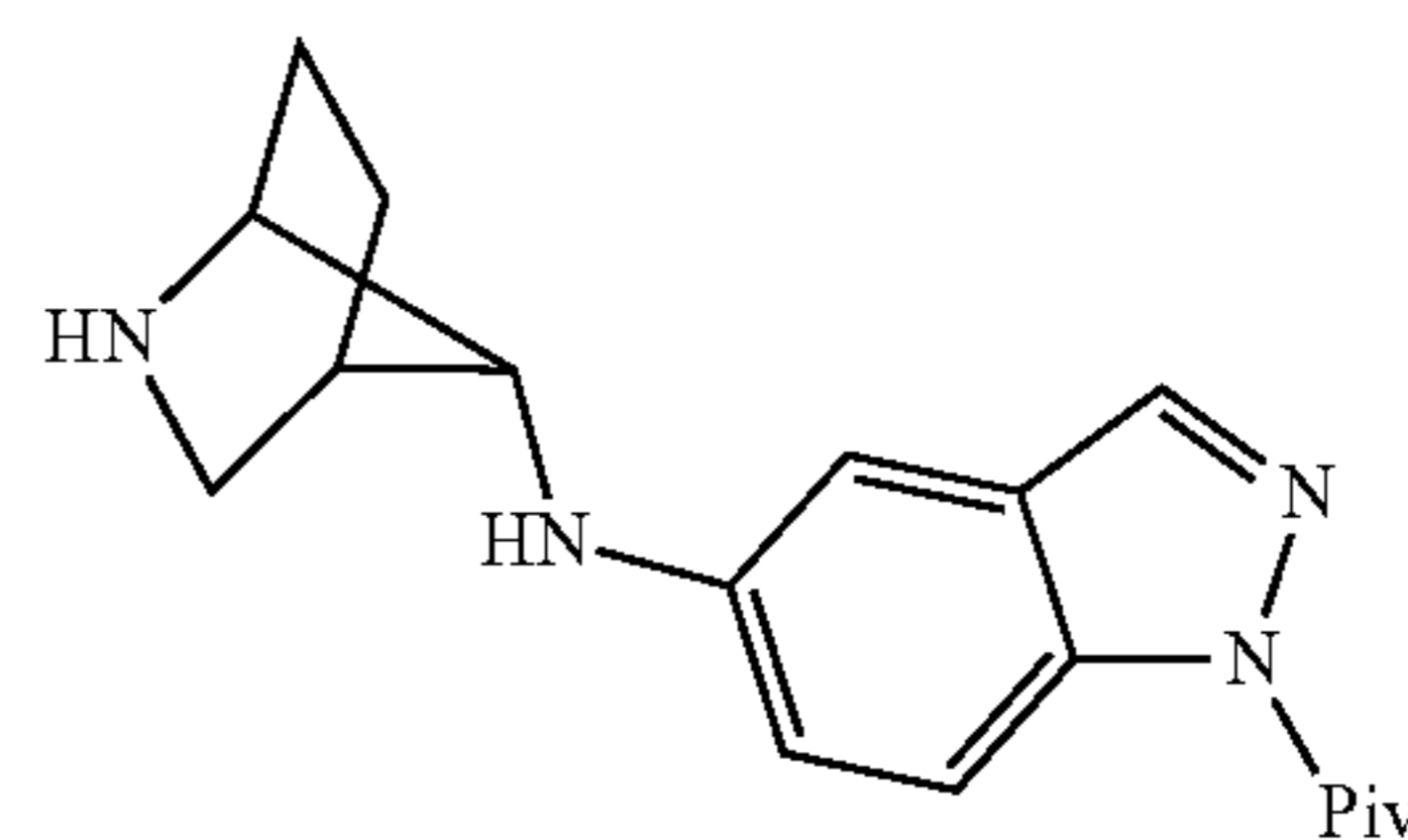
1-((1SR,4SR,7RS)-2-azabicyclo[2.2.1]heptan-7-ylamino)-1H-indazol-1-yl)-2,2-dimethylpropan-1-one, Intermediate 14
