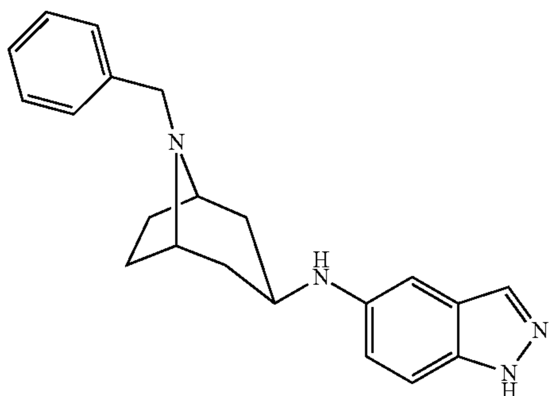
N-((1RS,3sr,5SR)-8-benzyl-8-azabicyclo[3.2.1]octan-3-yl)-1H-indazol-5-amine, Compound 2.1.01
