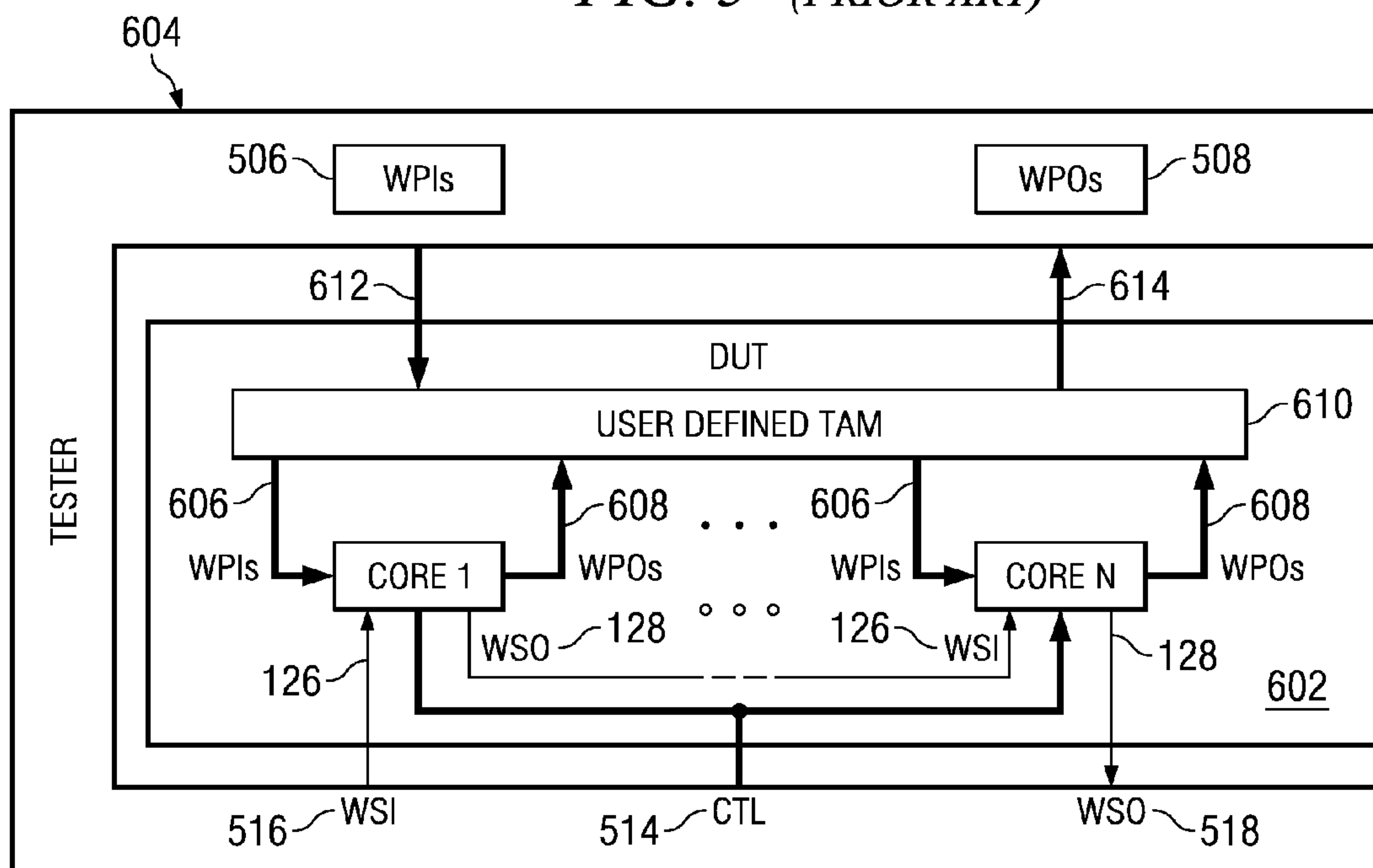
FIG. 6 (PRIOR ART)
