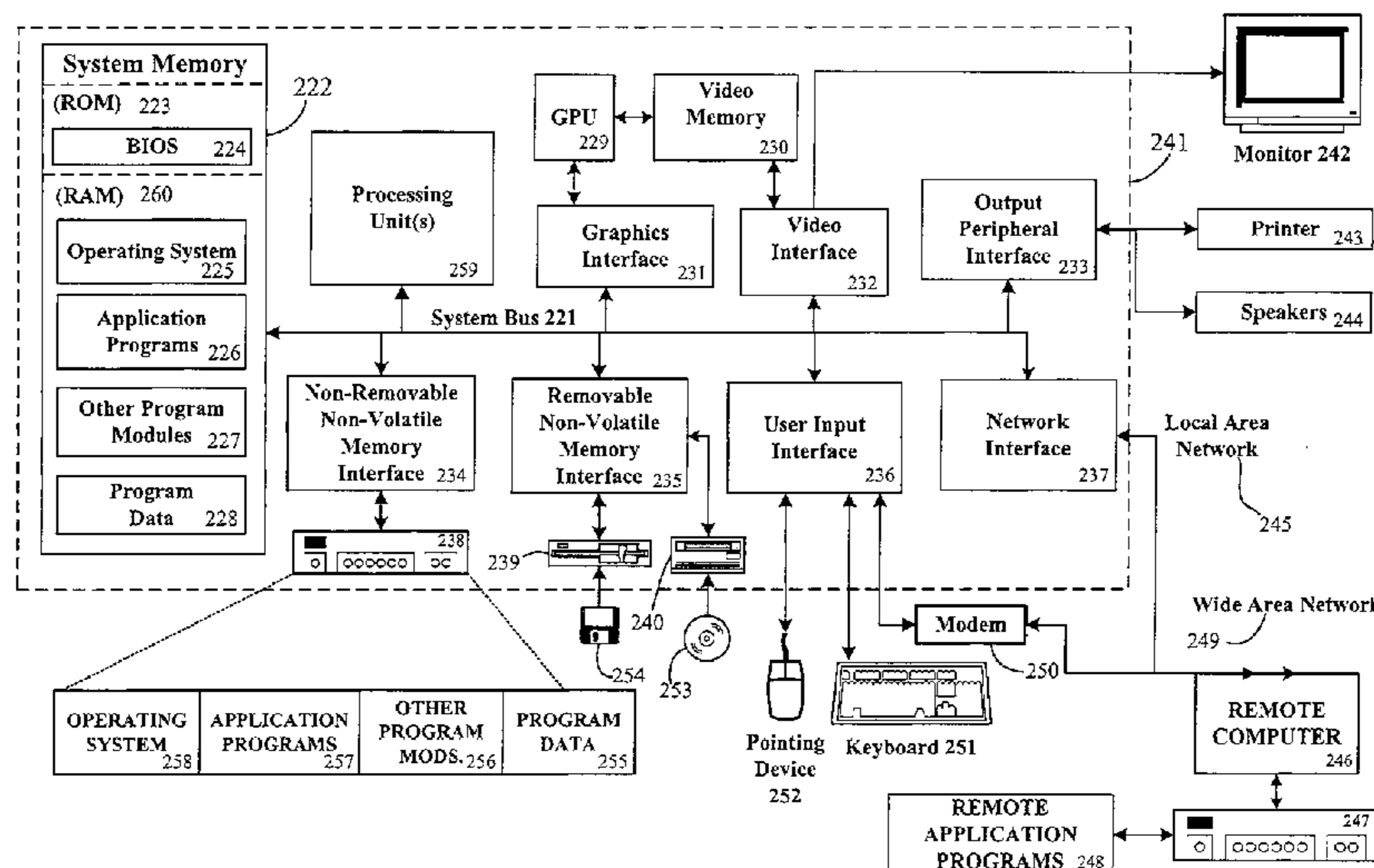
Computing Environment 220
