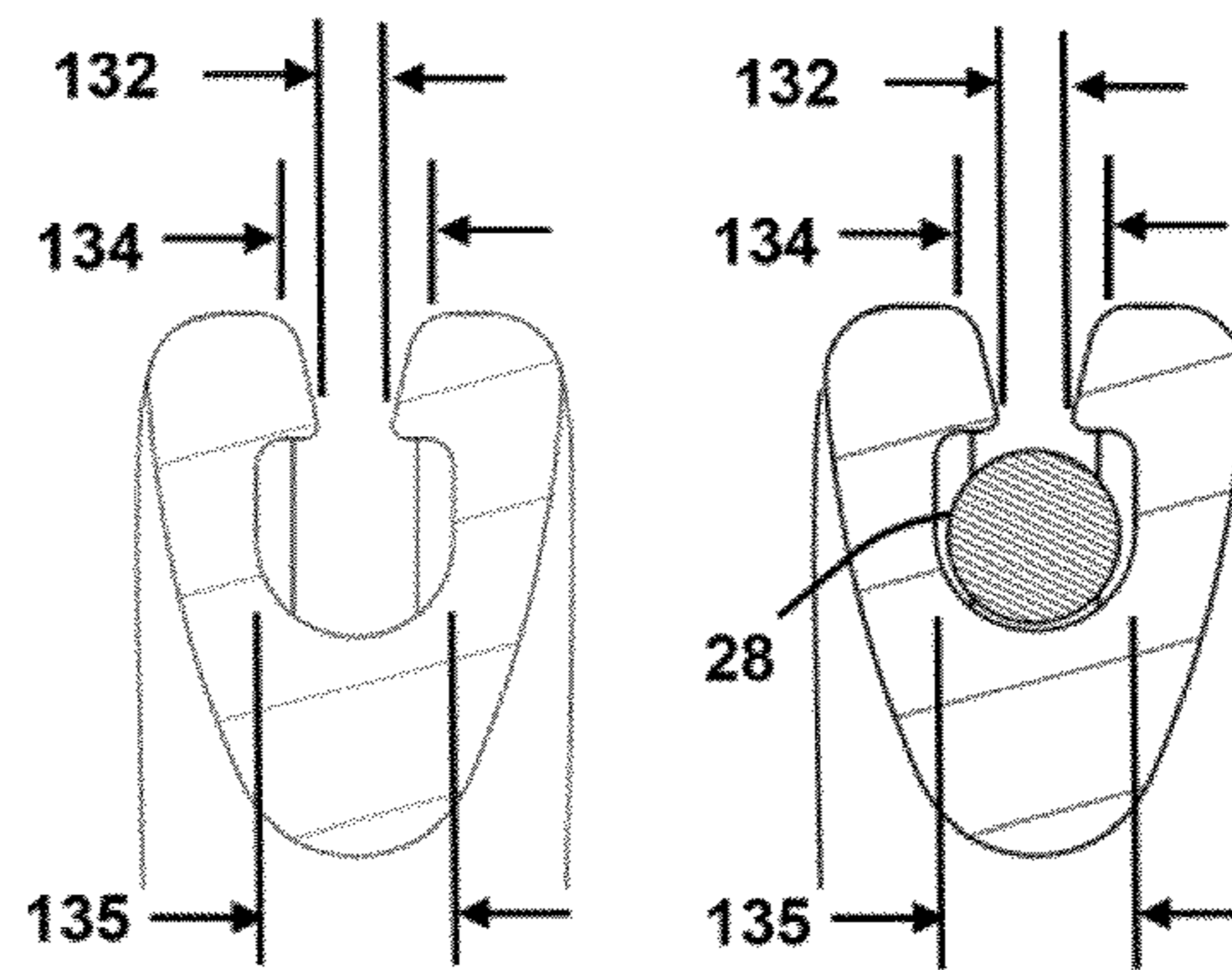
SECTION E-E
