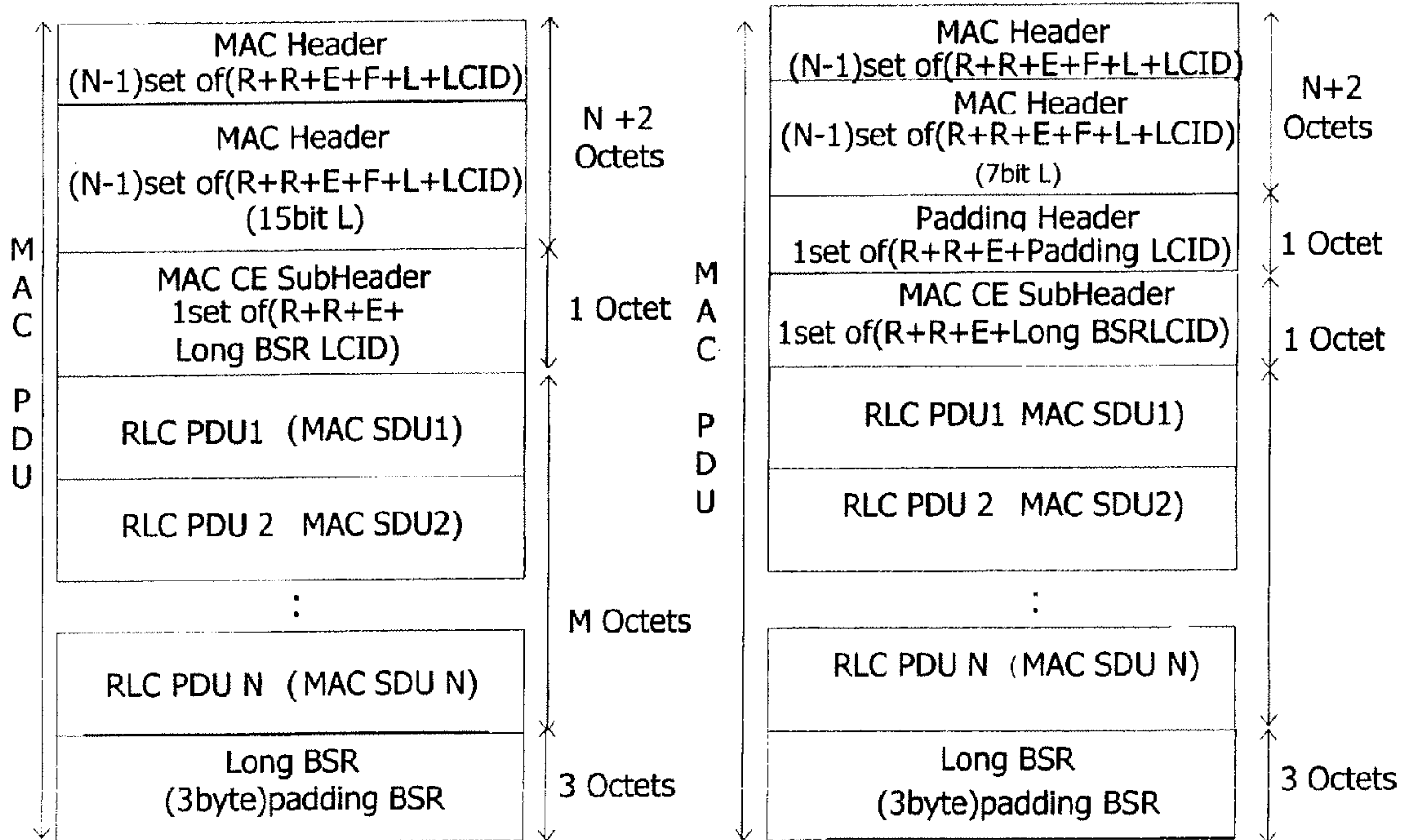
(b)case2, explicit padding BSR
