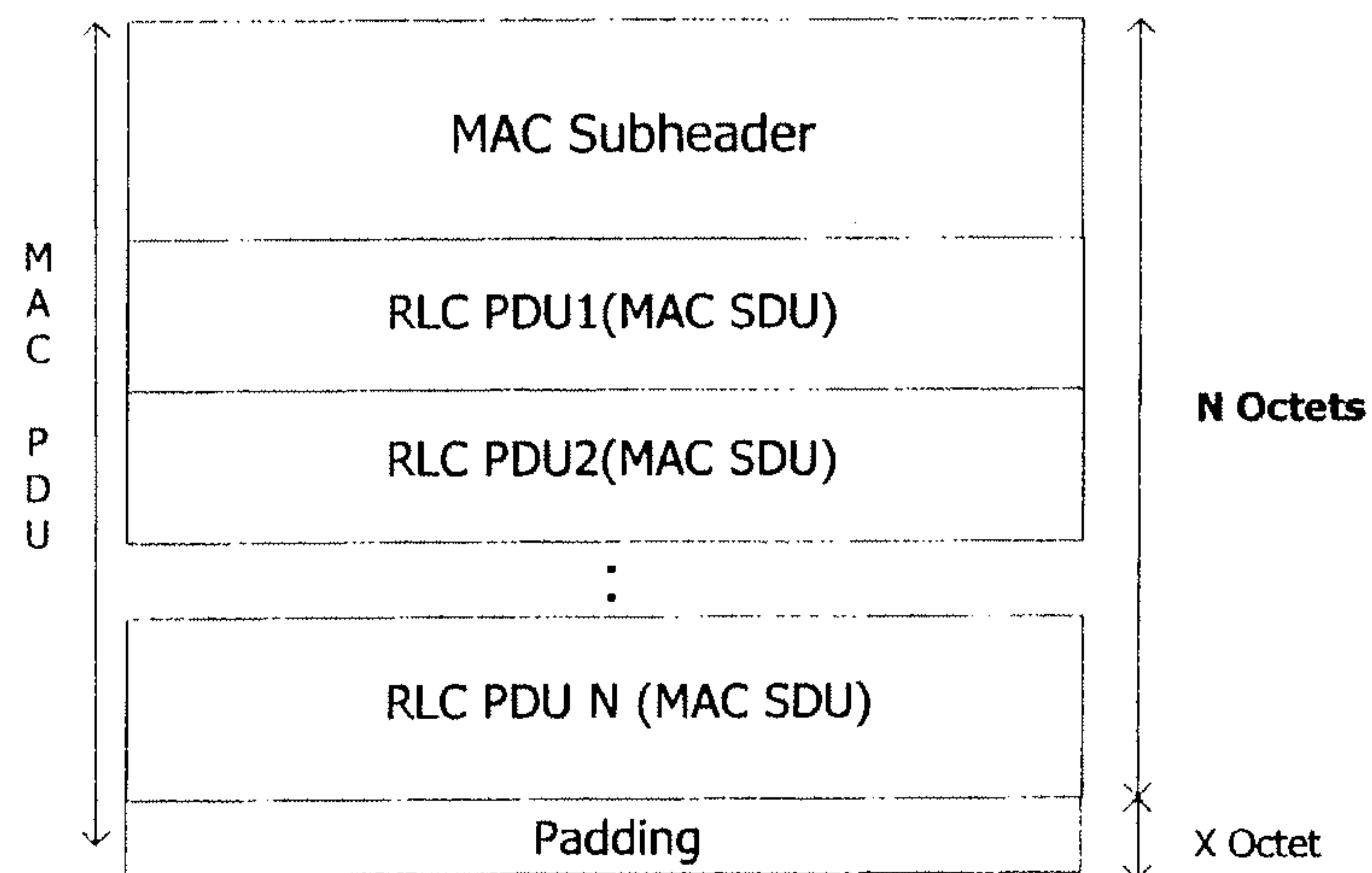
(a) MAC PDU with data and padding
