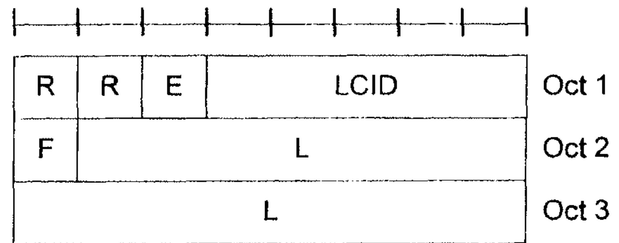
R/R/E/LCID/F/L sub-header with 15-bits L field
