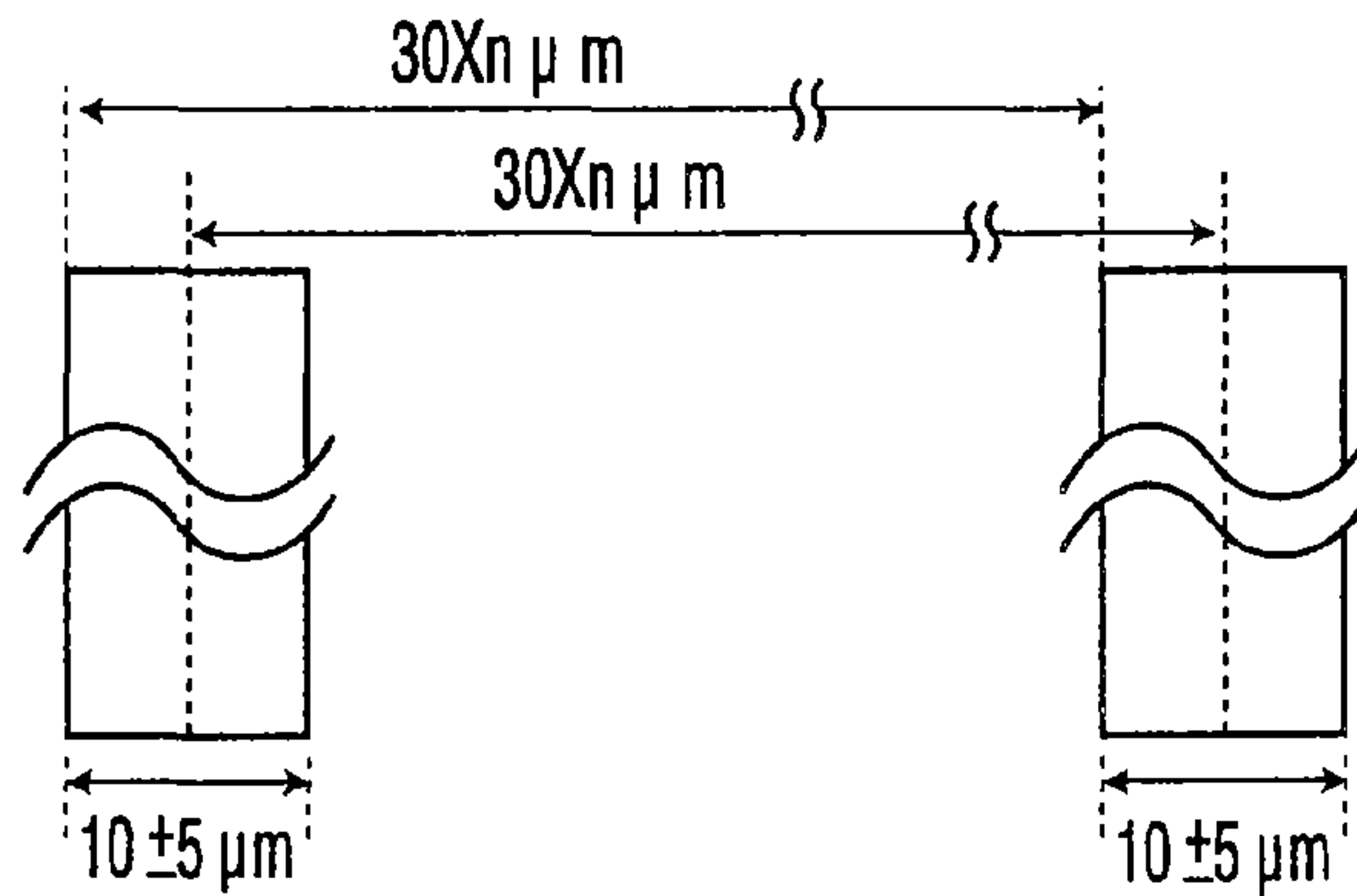
DIMENSIONAL ACCURACY OF SLIT (AT r=22.2mm )
