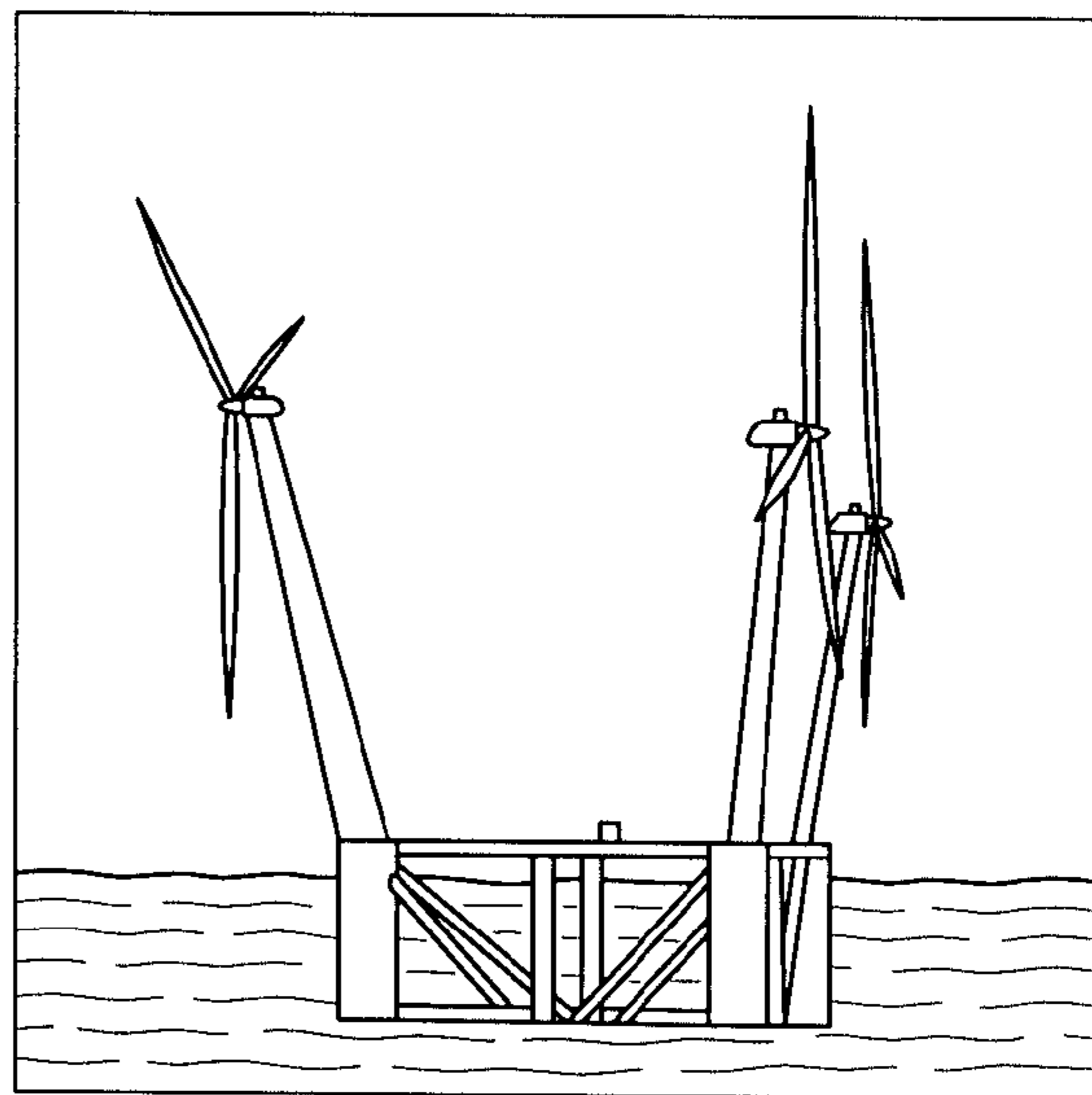
FIG. 4 (PRIOR ART)
