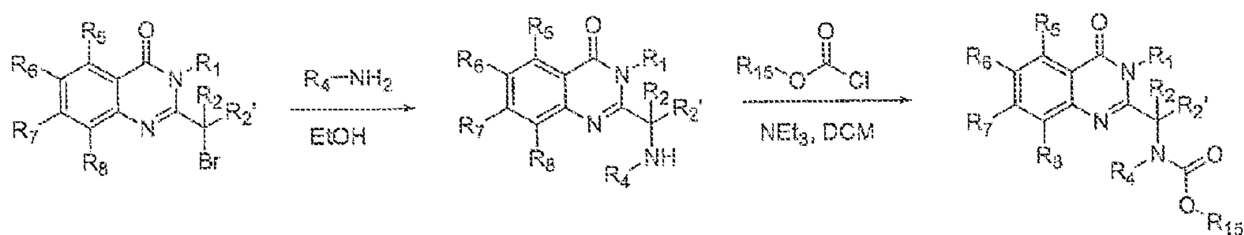
Figure 5c: Urea Synthesis
