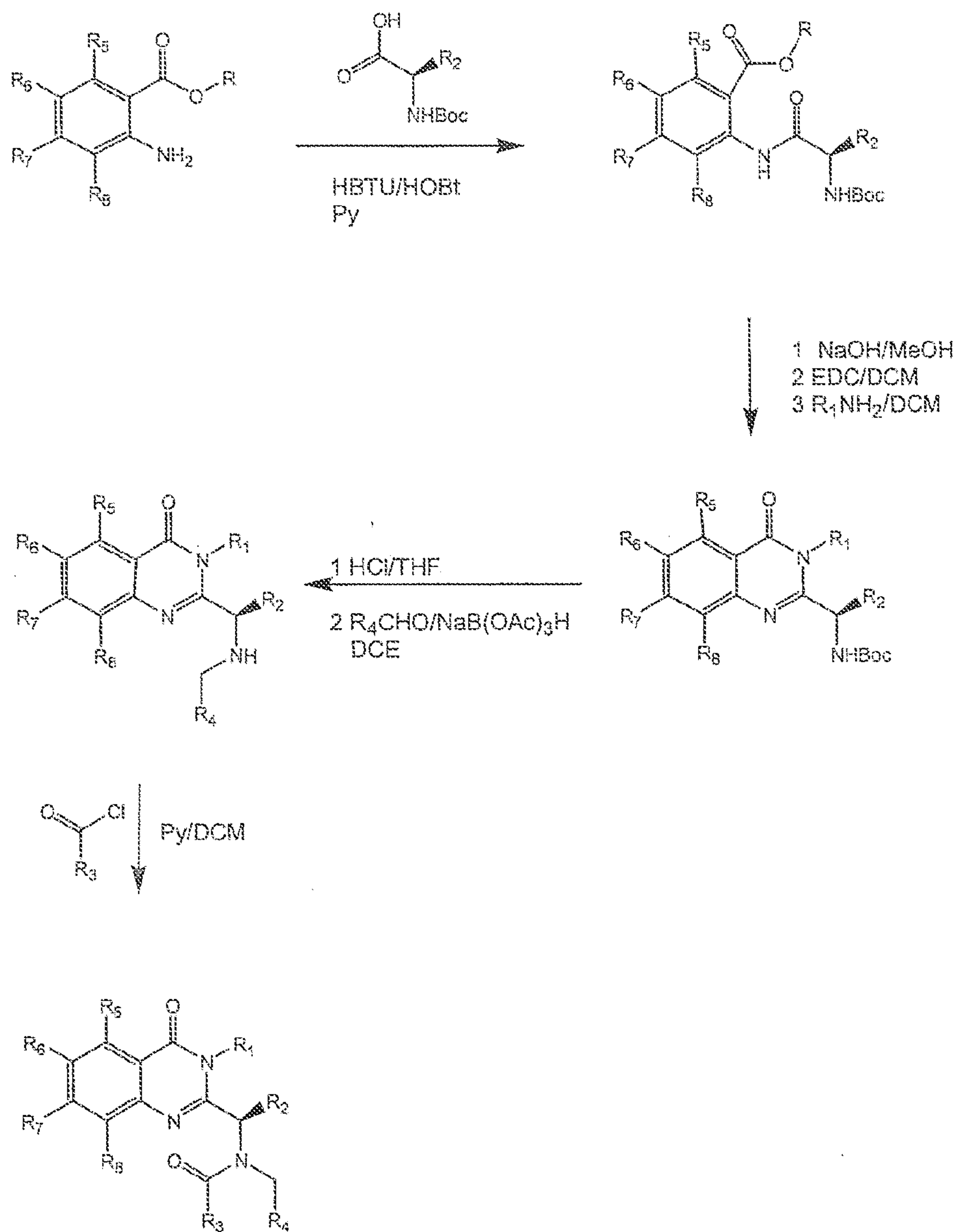
Figure 4: Asymmetric Synthesis
