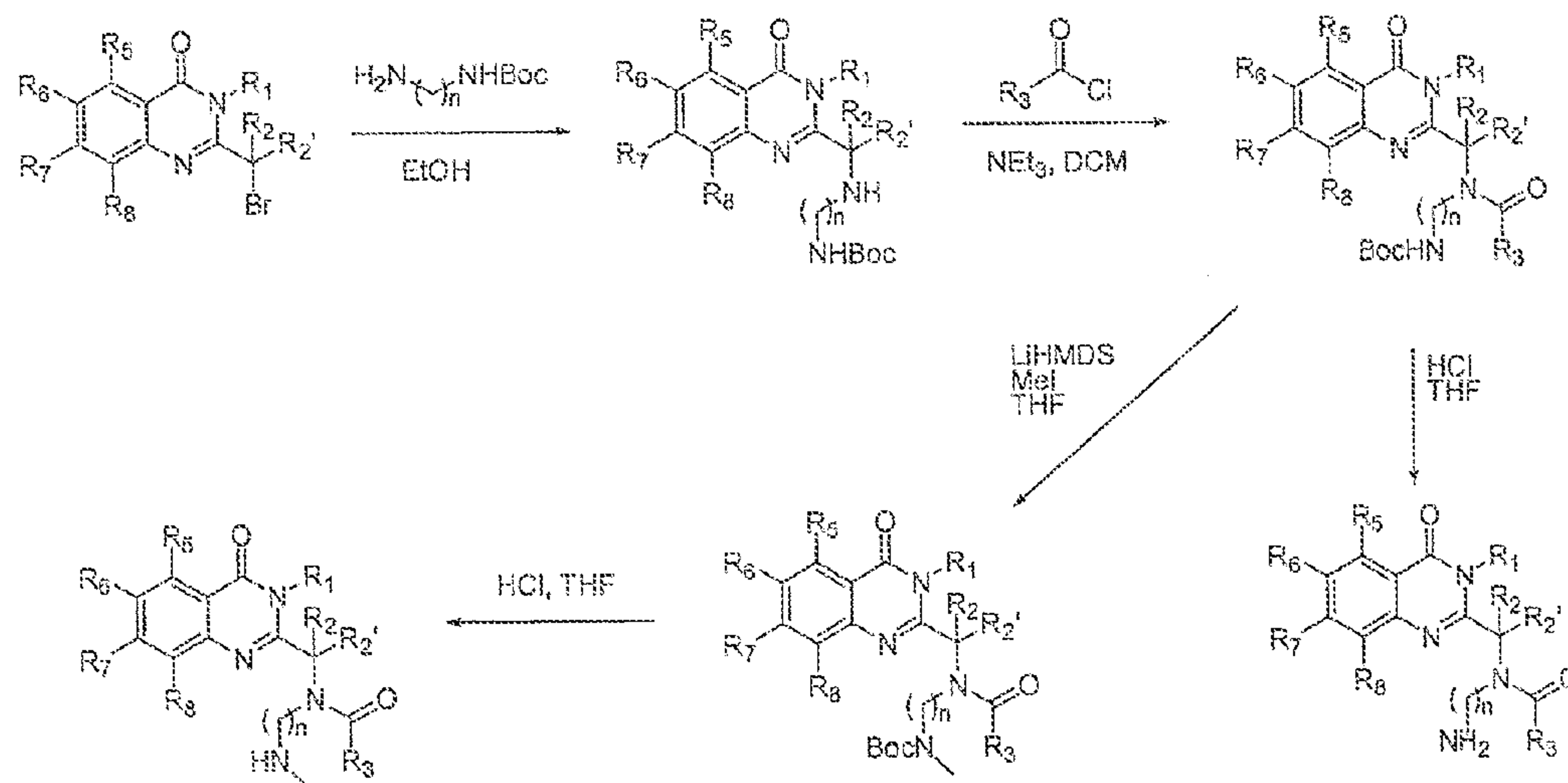
Figure 5d: Primary and Secondary Amine R4 Synthesis
