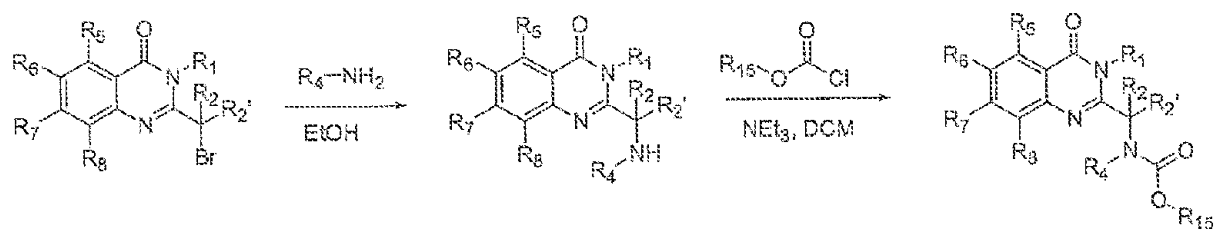
Figure 5c: Urea Synthesis
