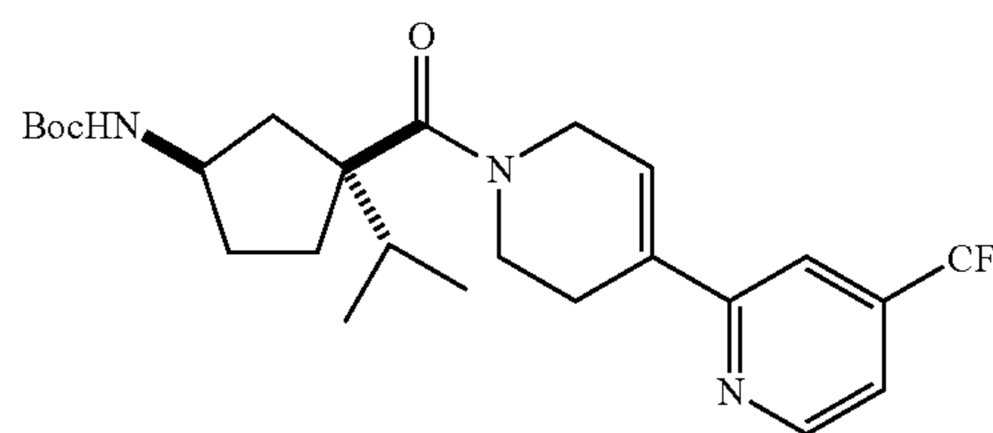
tert-Butyl ((1R,3S)-3-isopropyl-3-[[4-(trifluoromethyl)-3',6'-dihydro-2,4'-bipyridin-1'(2'H)-yl]carbonyl]cyclopentyl)carbamate
