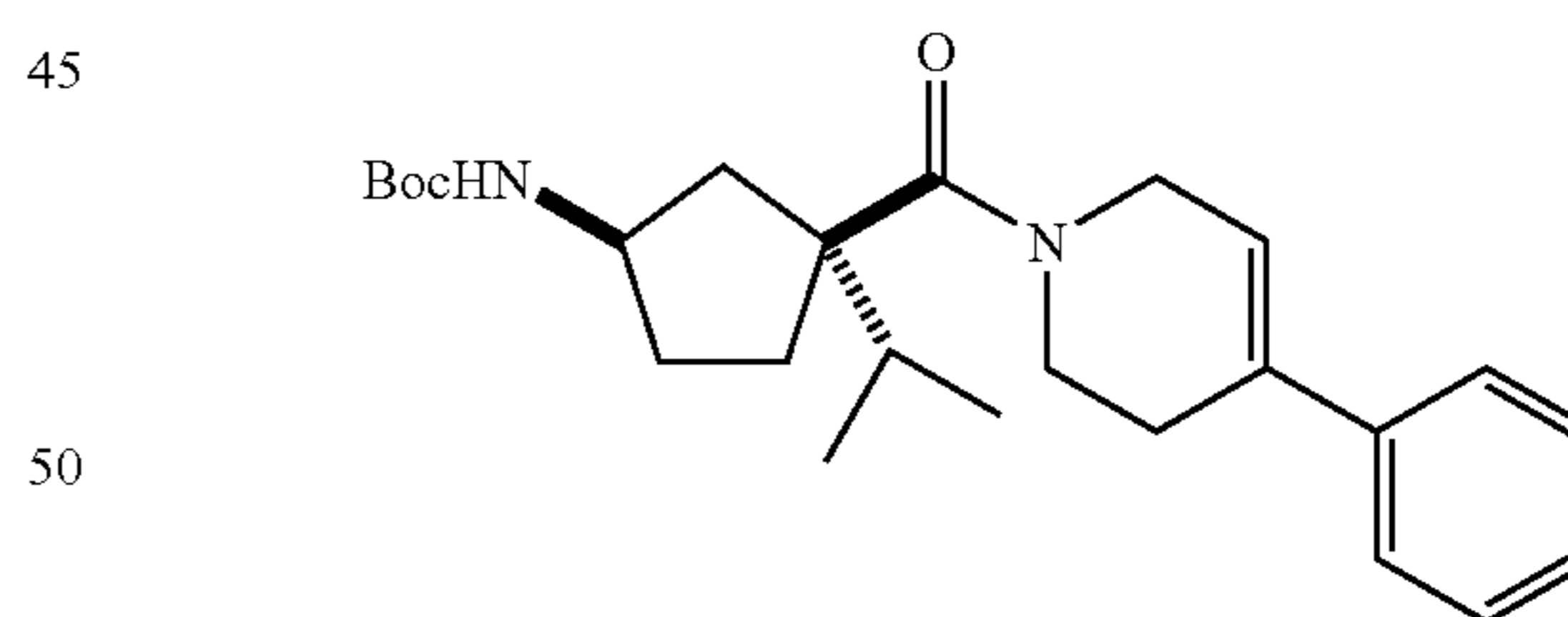
tert-Butyl {(1R,3S)-3-Isopropyl-3-[(4-phenyl-3,6-dihydropyridin-1(2H)-yl)carbonyl]cyclopentyl}carbamate
