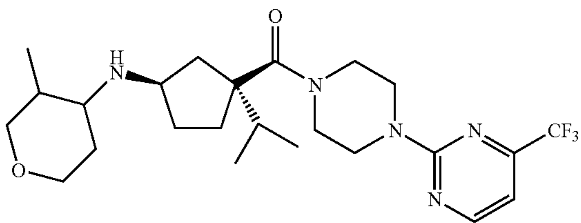
N-[(1R,3S)-3-Isopropyl-3-(4-[4-(trifluoromethyl)pyrimidin-2-yl]piperazin-1-yl)carbonyl]cyclopentyl]-3-methyltetrahydro-2H-pyran-4-amine
