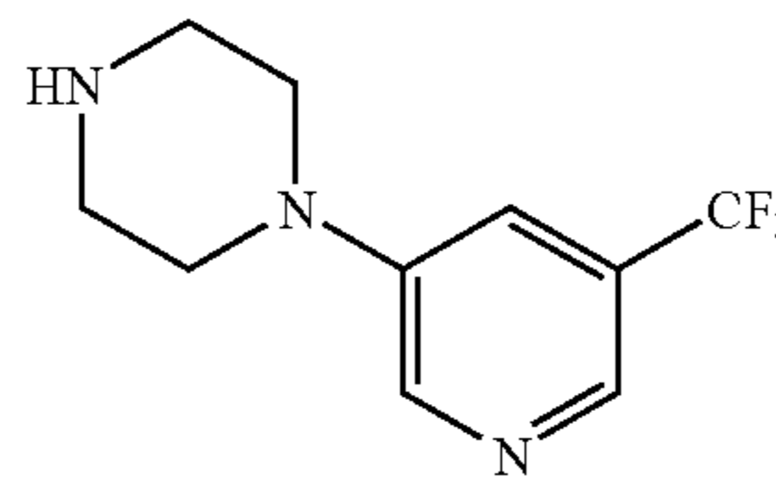
1-[5-(Trifluoromethyl)pyridin-3-yl]piperazine
