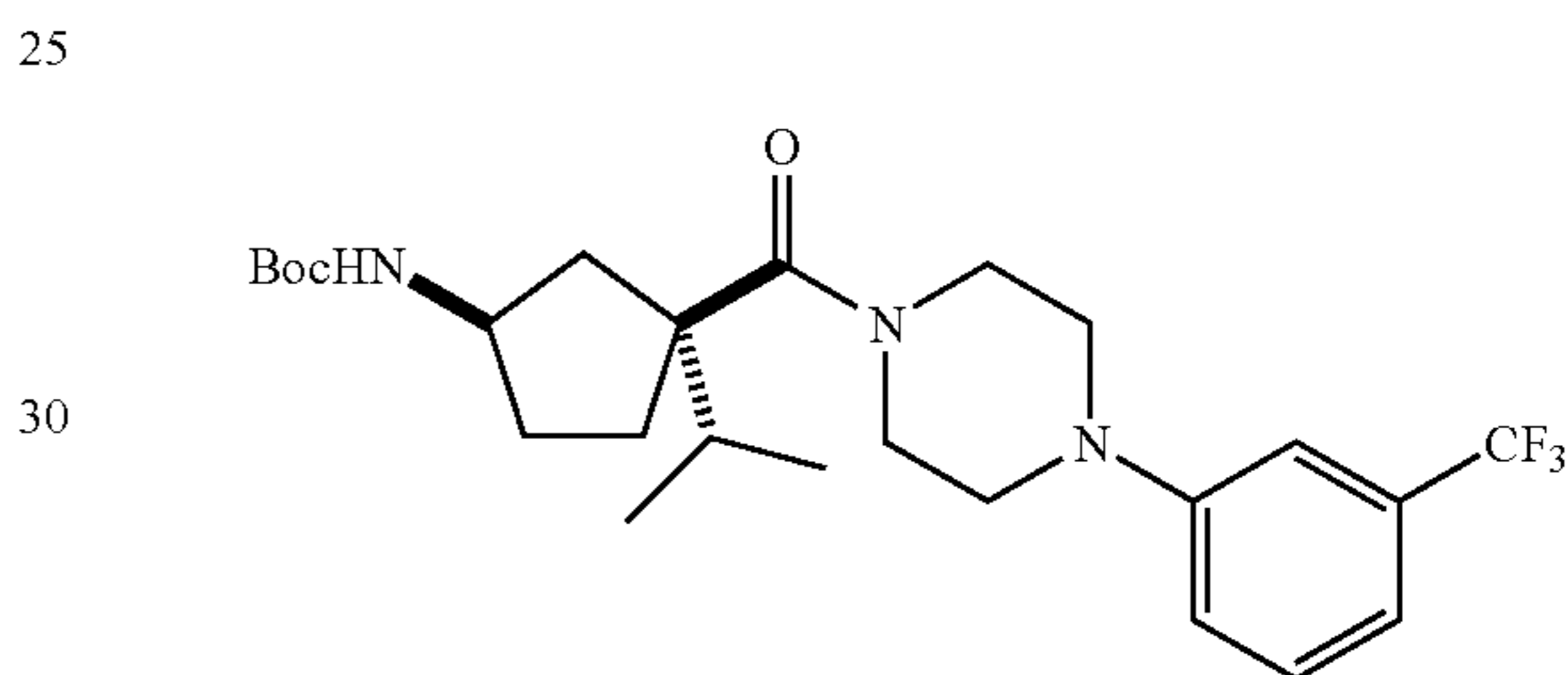
tert-Butyl [(1R,3S)-3-isopropyl-3-({4-[3-(trifluoromethyl)phenyl]piperazin-1-yl} carbonyl)cyclopentyl] carbamate
