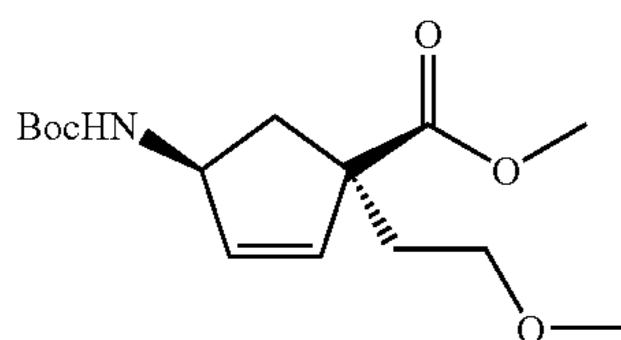
Methyl (1S,4S)-4-[(tert-Butoxycarbonyl)amino]-1-(2-methoxyethyl)cyclopent-2-ene-1-carboxylate
