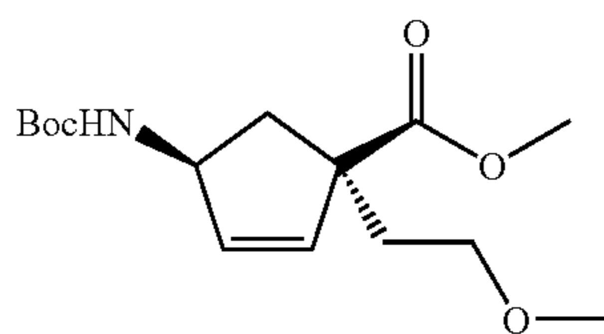
Methyl (1S,4S)-4-[(tert-Butoxycarbonyl)amino]-1-(2-methoxyethyl)cyclopent-2-ene-1-carboxylate
