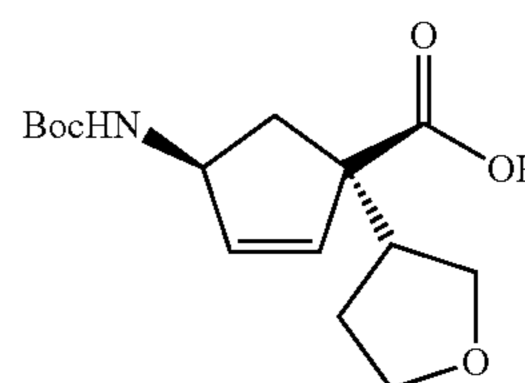
(1R,4S)-4-[(tert-Butoxycarbonyl)amino]-1-[(3R)-tetrahydrofuran-3-yl]cyclopent-2-ene-1-carboxylic acid
