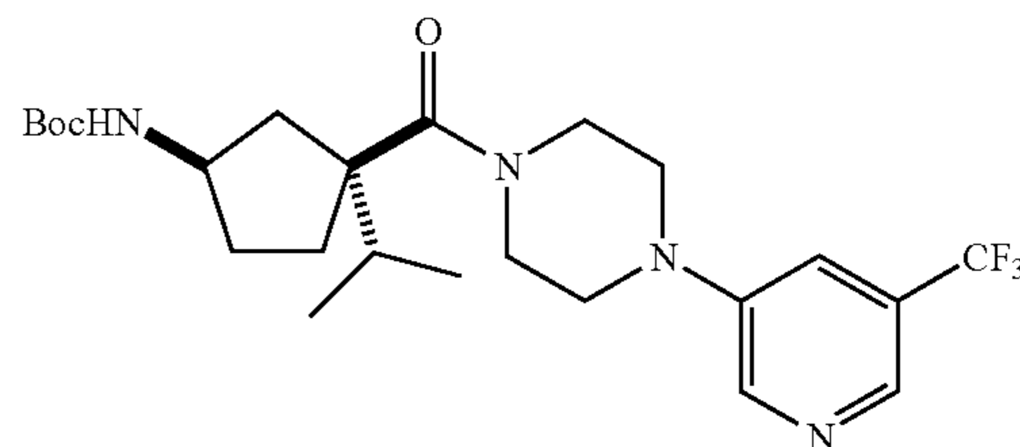
tert-Butyl [(1R,3S)-3-Isopropyl-3-({4-[5-(trifluoromethyl)pyridin-3-yl]piperazin-1-yl}carbonyl)cyclopentyl]carbamate
