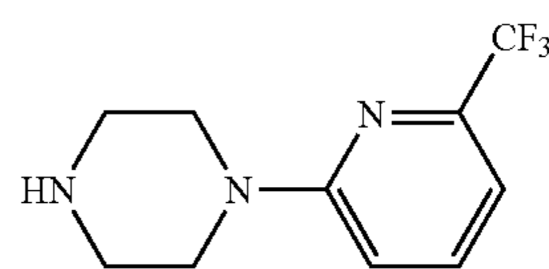
1-[6-(Trifluoromethyl)pyridin-2-yl]piperazine
