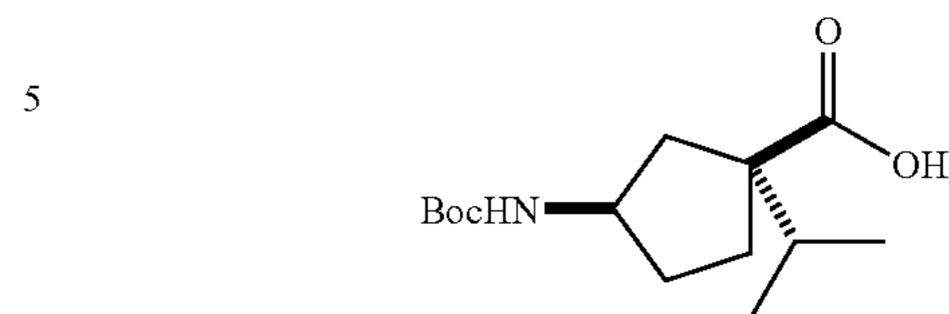
(1S,3R)-3-[(tert-Butoxycarbonyl)amino]-1-isopropylcyclopentanecarboxylic acid
