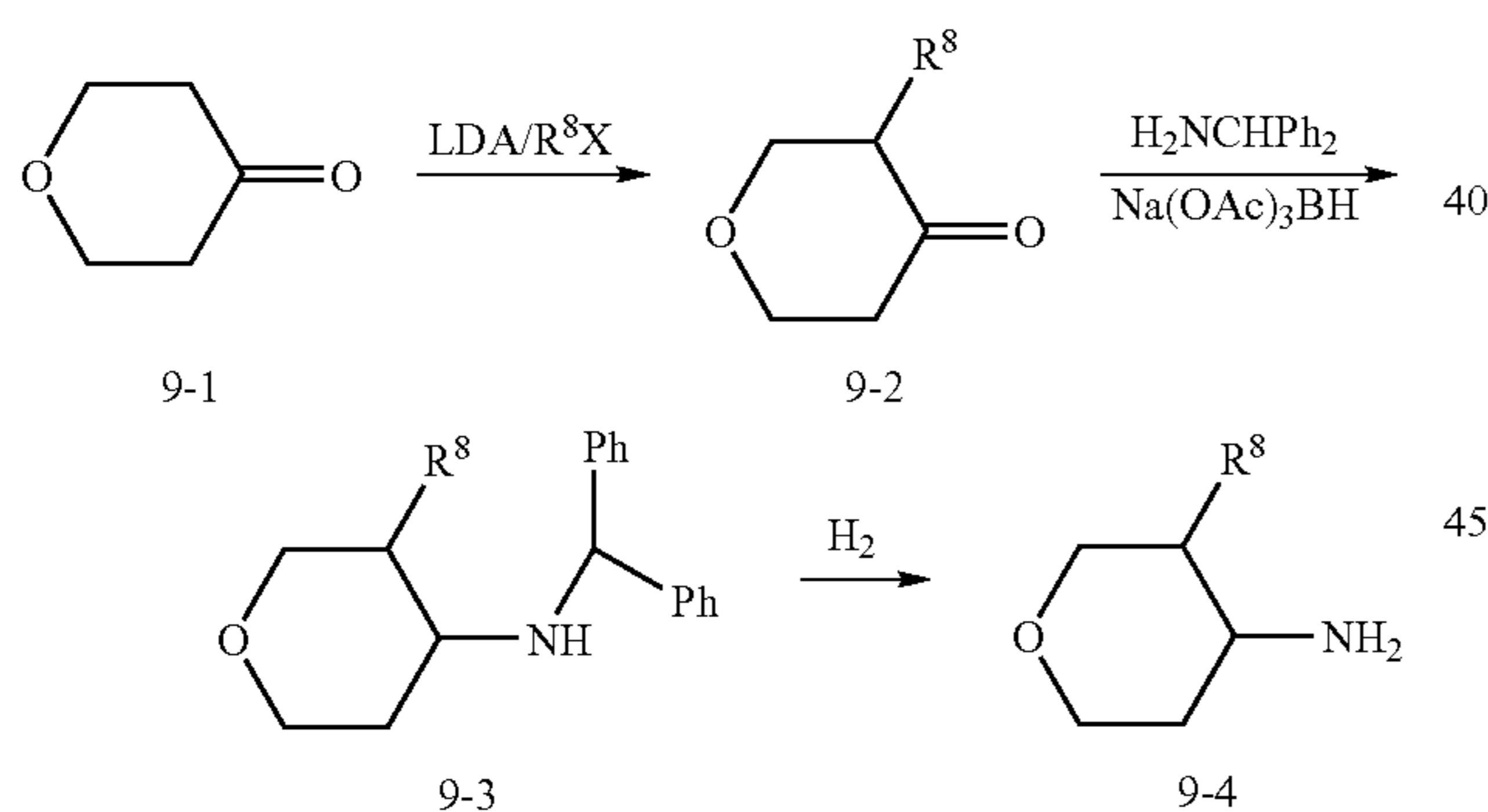
Scheme 9
