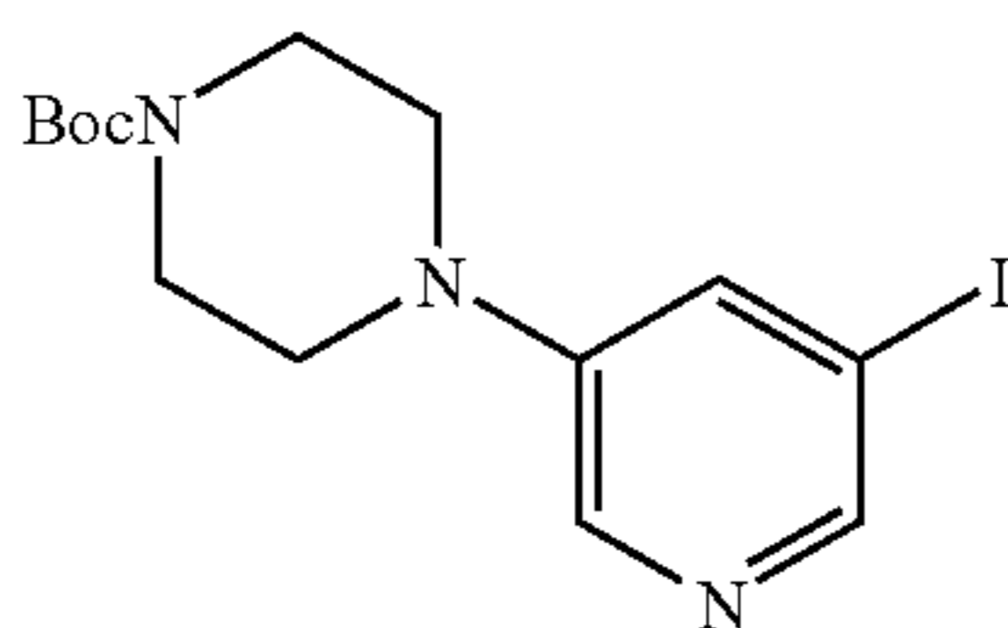
tert-Butyl 4-(5-Iodopyridin-3-yl)piperazine-1-carboxylate
