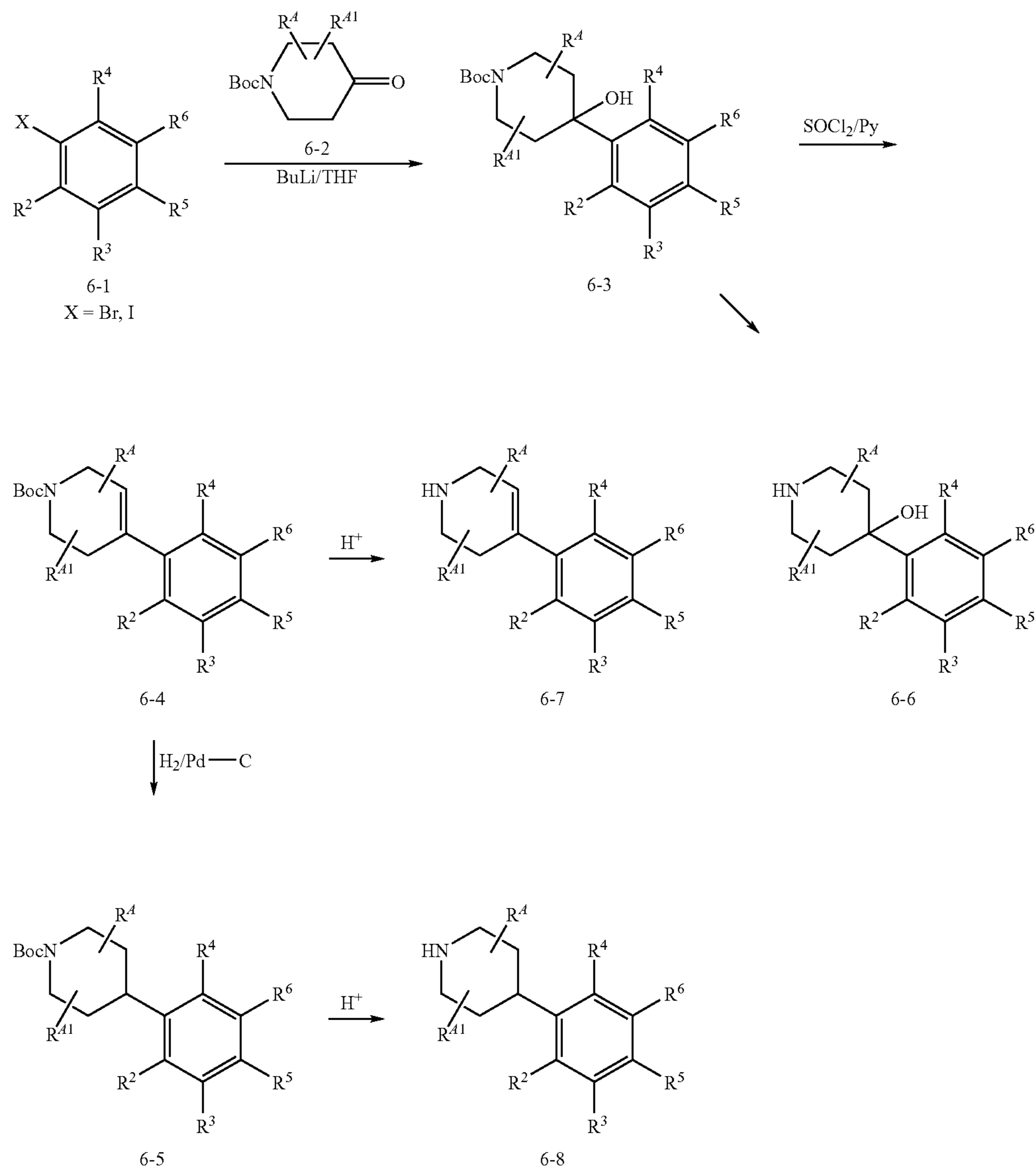
Scheme 6
