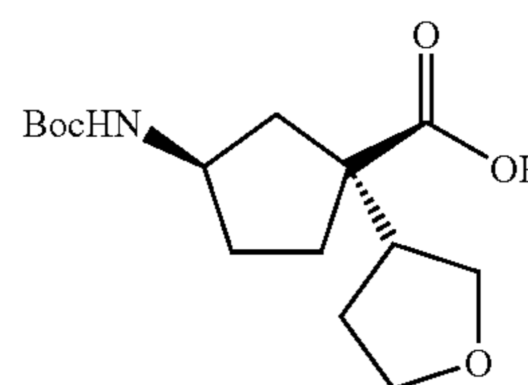
(1S,3R)-3-[(tert-Butoxycarbonyl)amino]-1-[(3R)-tetrahydrofuran-3-yl]cyclopentanecarboxylic acid
