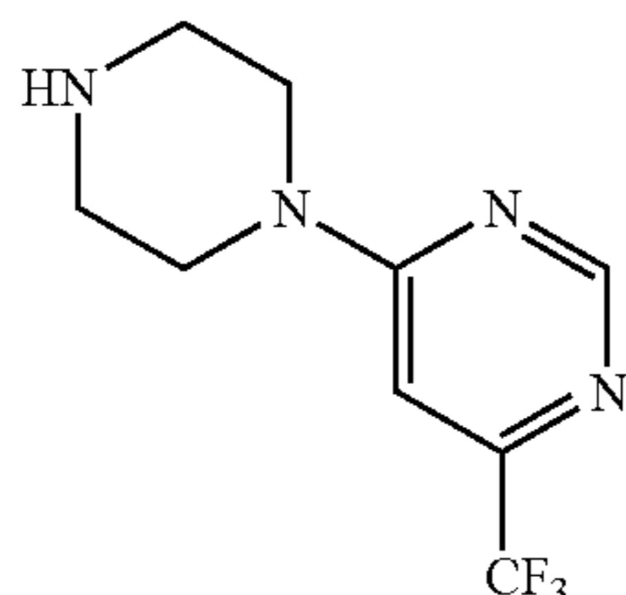
4-piperazin-1-yl-6-(trifluoromethyl)pyrimidine
