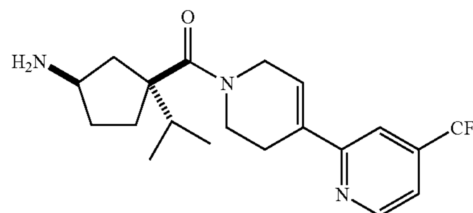
(1R,3S)-3-Isopropyl-3-[[4-(trifluoromethyl)-3',6'-dihydro-2,4'-bipyridin-1'(2'H)-yl]carbonyl]cyclopentanamine
