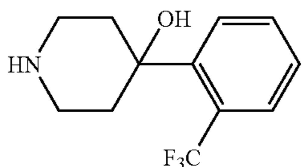
4-[2-(Trifluoromethyl)phenyl]piperidin-4-ol
