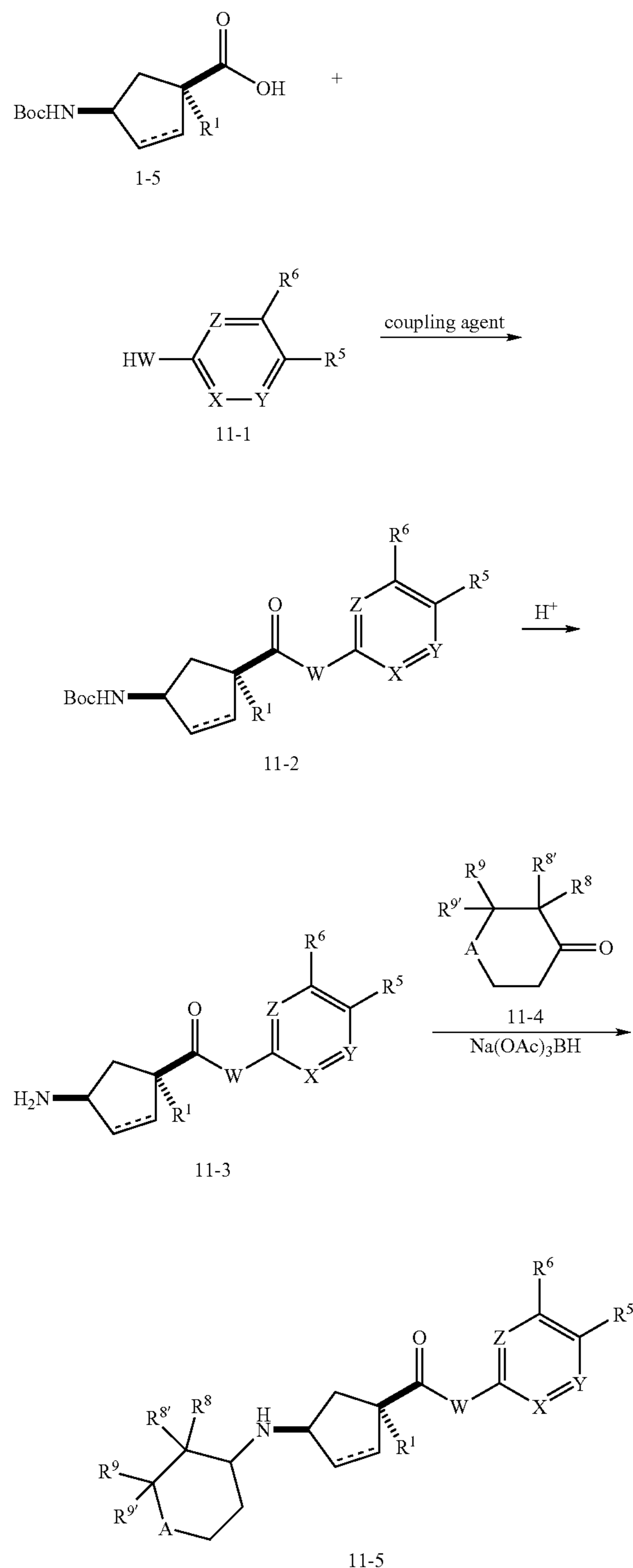
Scheme 11
