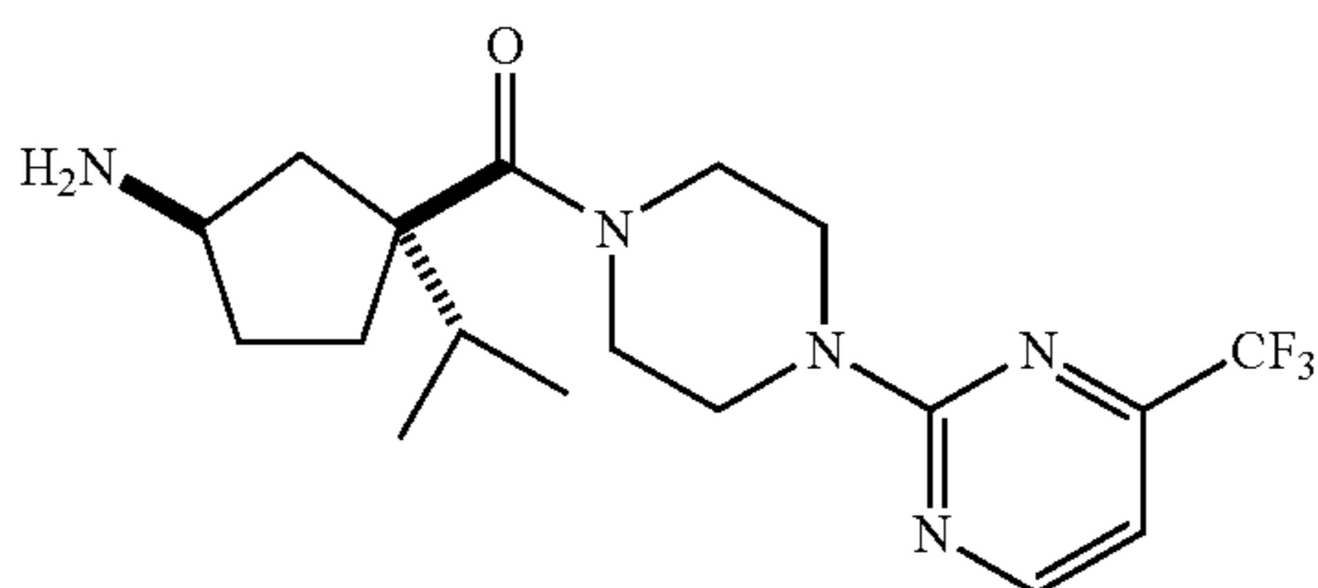
(1R,3S)-3-Isopropyl-3-(4-[4-(trifluoromethyl)pyrimidin-2-yl]piperazin-1-yl)carbonyl]cyclopentan-amine
