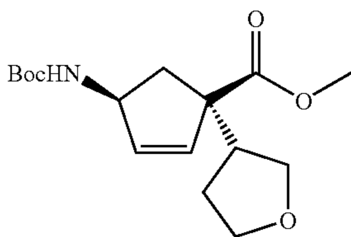
Methyl (1R,4S)-4-[(tert-Butoxycarbonyl)amino]-1-[(3R)-tetrahydrofuran-3-yl]cyclopent-2-ene-1-carboxylate
