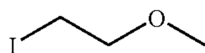
1-Iodo-2-methoxyethane
