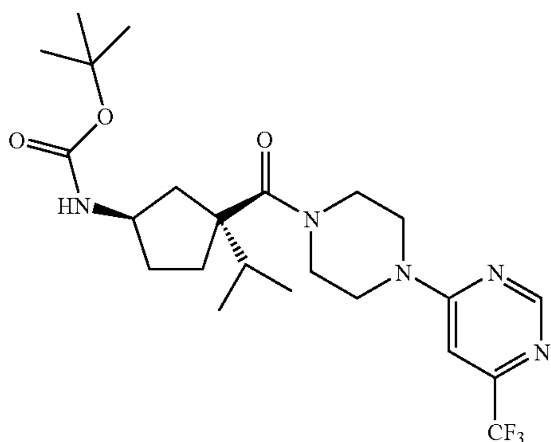
tert-Butyl [(1R,3S)-3-isopropyl-3-(4-[6-(trifluoromethyl)pyrimidin-4-yl]piperazin-1-ylcarbonyl)cyclopentyl]carbamate
