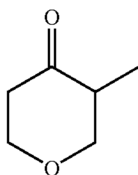
3-Methyltetrahydro-4H-pyran-4-one
