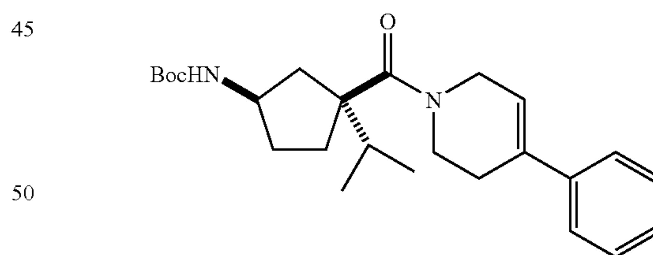
tert-Butyl {(1R,3S)-3-Isopropyl-3-[(4-phenyl-3,6-dihydropyridin-1(2H)-yl)carbonyl]cyclopentyl}carbamate
