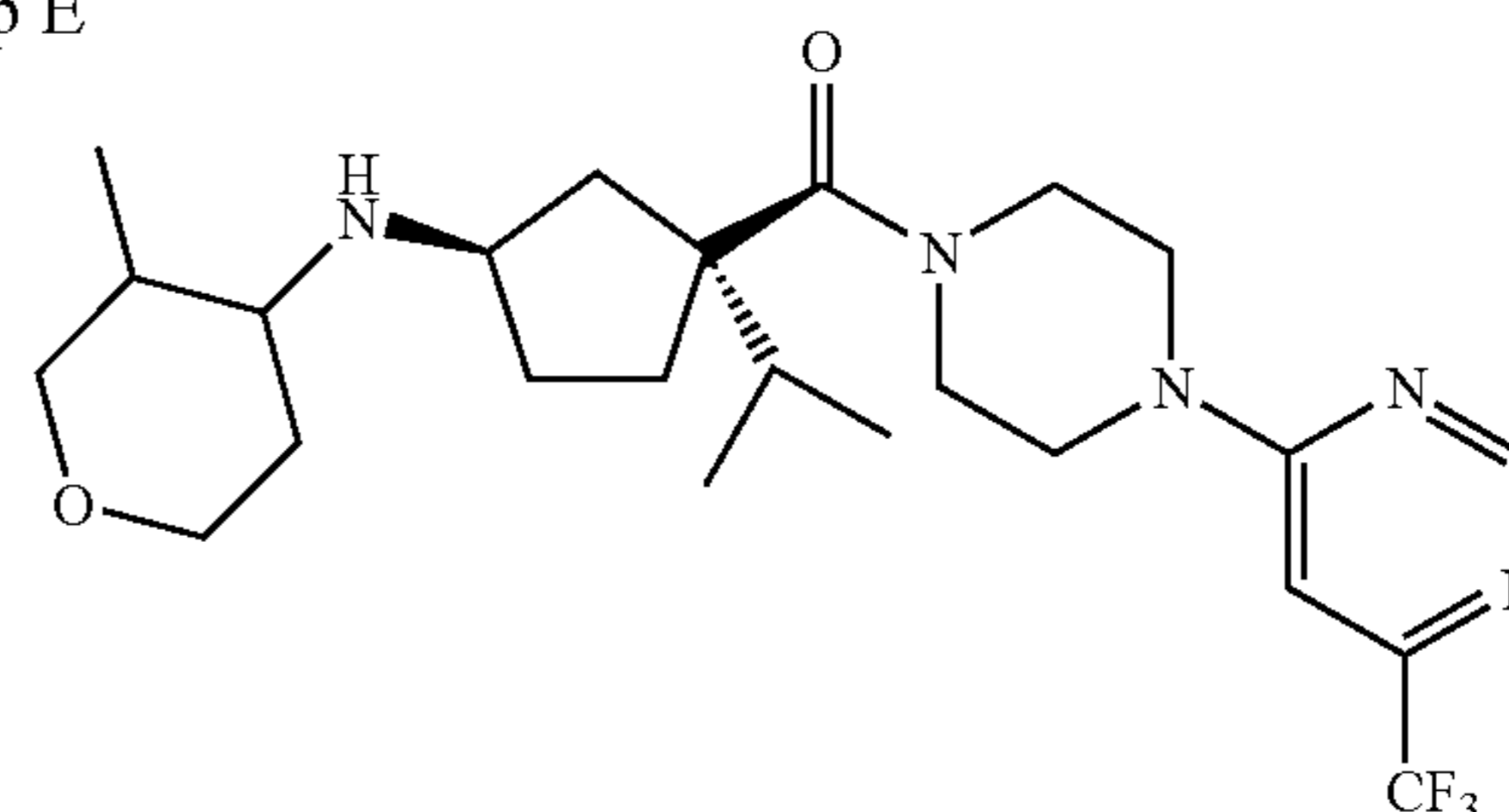
N-[(1R,3S)-3-isopropyl-3-(4-[6-(trifluoromethyl)pyrimidin-4-yl]piperazin-1-ylcarbonyl)cyclopentyl]-3-methyltetrahydro-2H-pyran-4-amine
