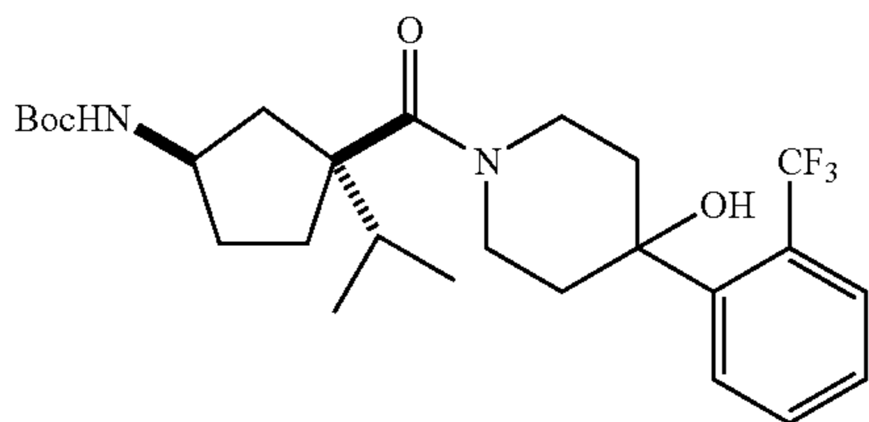
tert-Butyl [(1R,3S)-3-({4-hydroxy-4-[2-(trifluoromethyl)phenyl]piperidin-1-yl}-carbonyl)-3-isopropylcyclopentyl]carbamate
