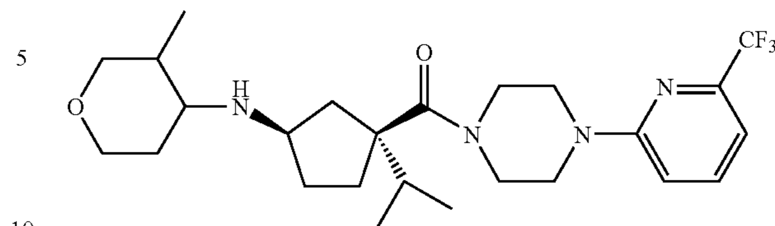
N-[(1R,3S)-3-isopropyl-3-(4-[6-(trifluoromethyl)pyridin-2-yl]piperazin-1-ylcarbonyl)cyclopentyl]-3-methyltetrahydro-2H-pyran-4-amine
