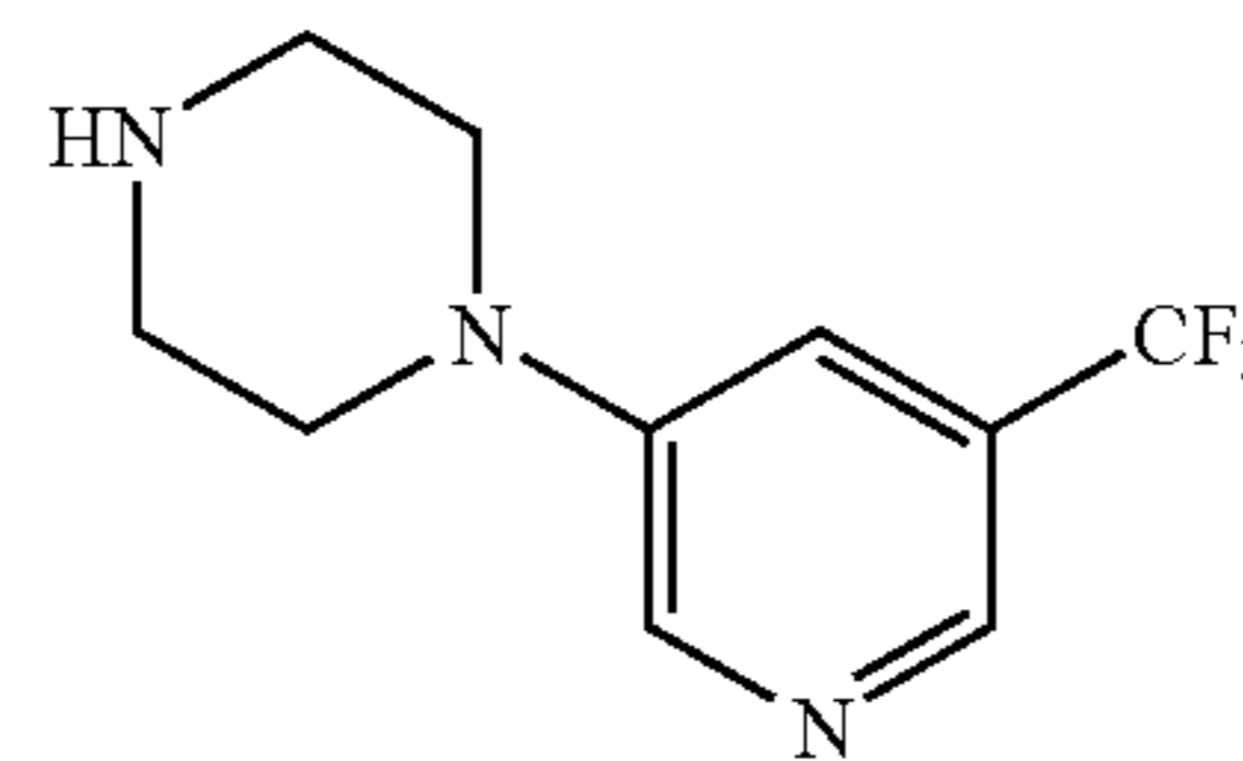
1-[5-(Trifluoromethyl)pyridin-3-yl]piperazine
