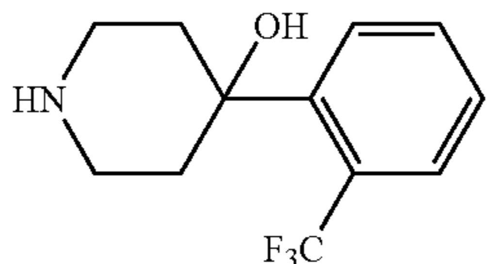
4-[2-(Trifluoromethyl)phenyl]piperidin-4-ol
