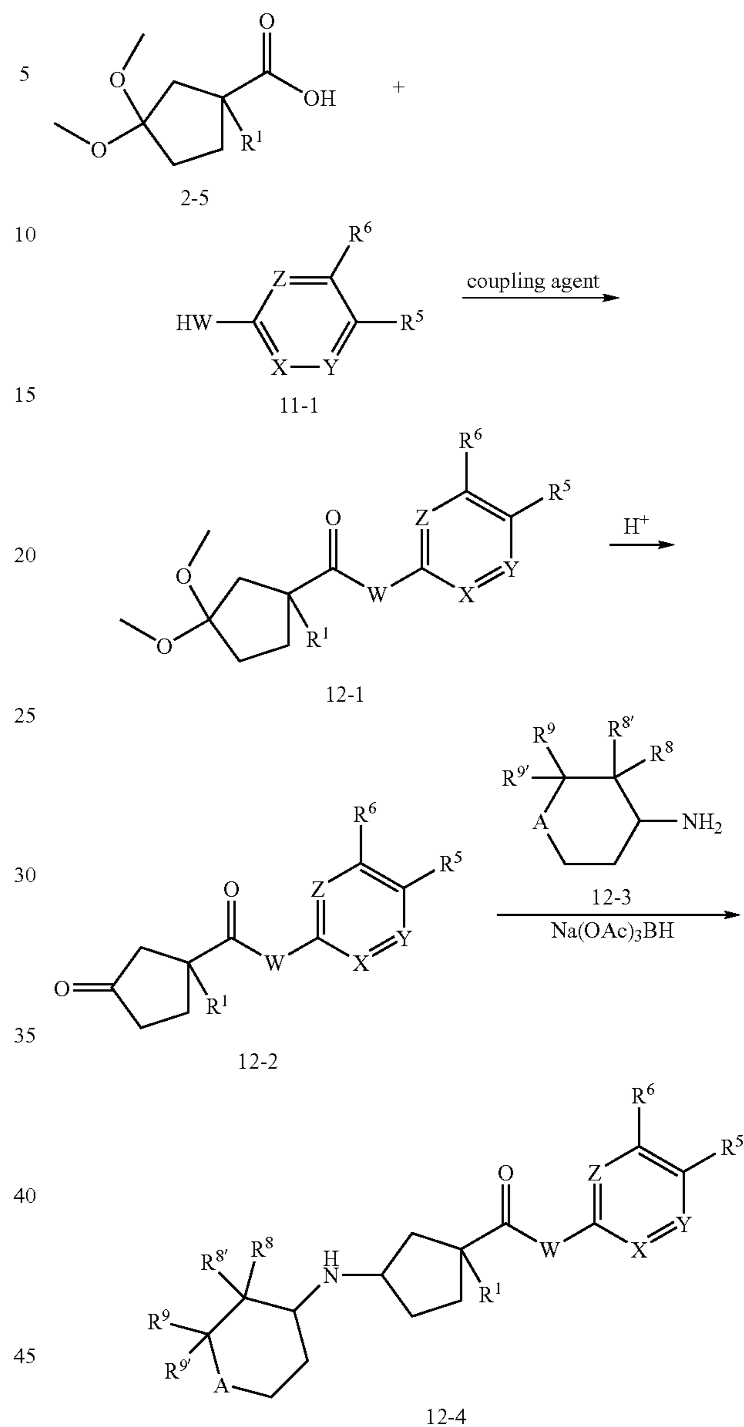
Scheme 12
