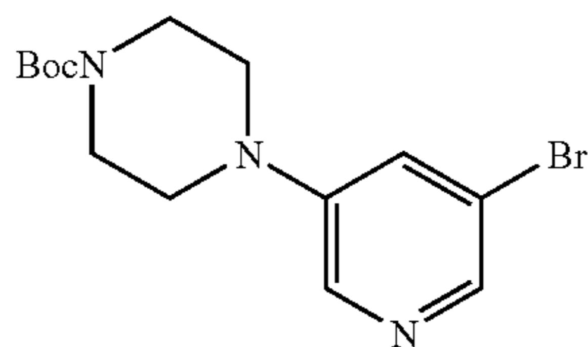
tert-Butyl 4-(5-Bromopyridin-3-yl)piperazine-1-carboxylate
