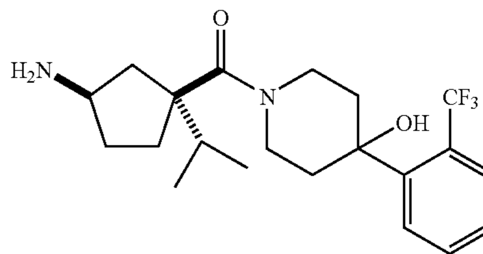
1-[(1S,3R)-3-Amino-1-isopropylcyclopentyl]carbonyl-4-[2-(trifluoromethyl)phenyl]piperidin-4-ol
