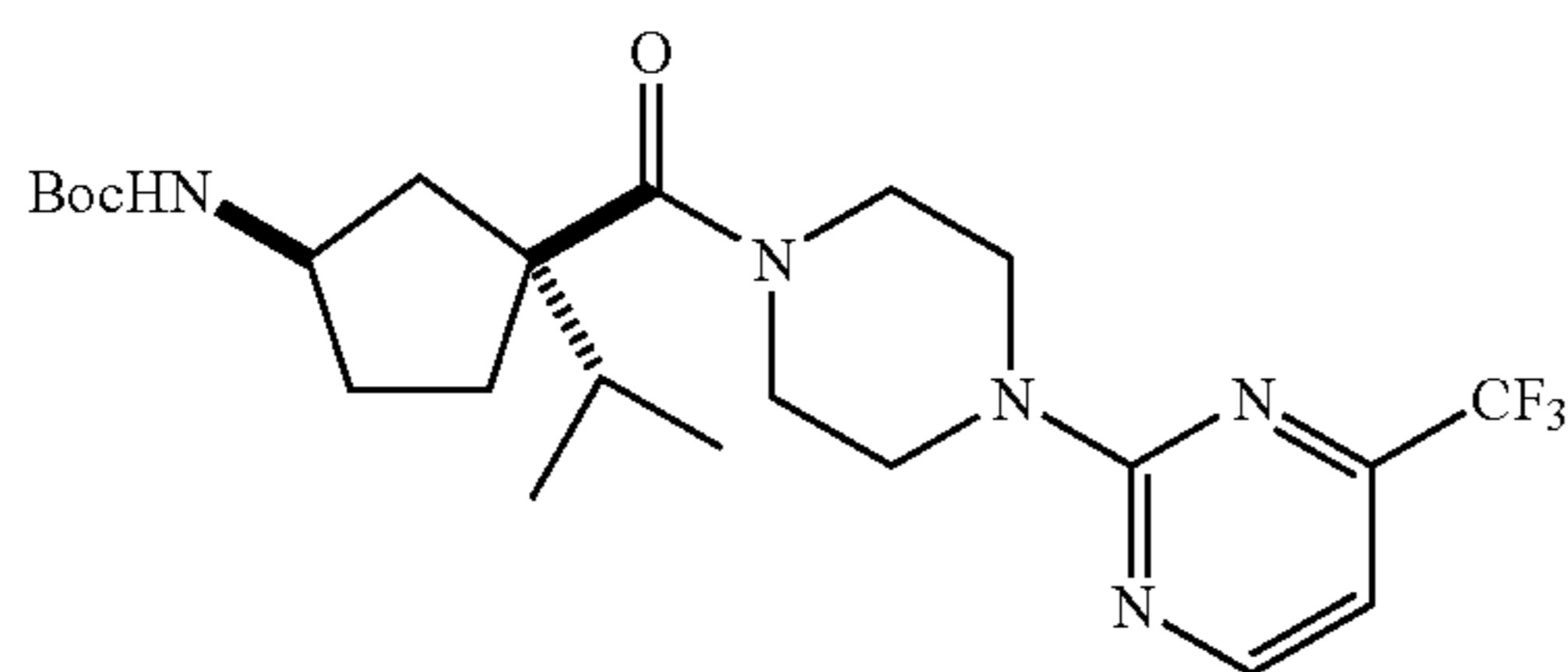
tert-Butyl [(1R,3S)-3-isopropyl-3-(4-[4-(trifluoromethyl)pyrimidin-2-yl]piperazin-1-yl)carbonyl]cyclopentyl]carbamate
