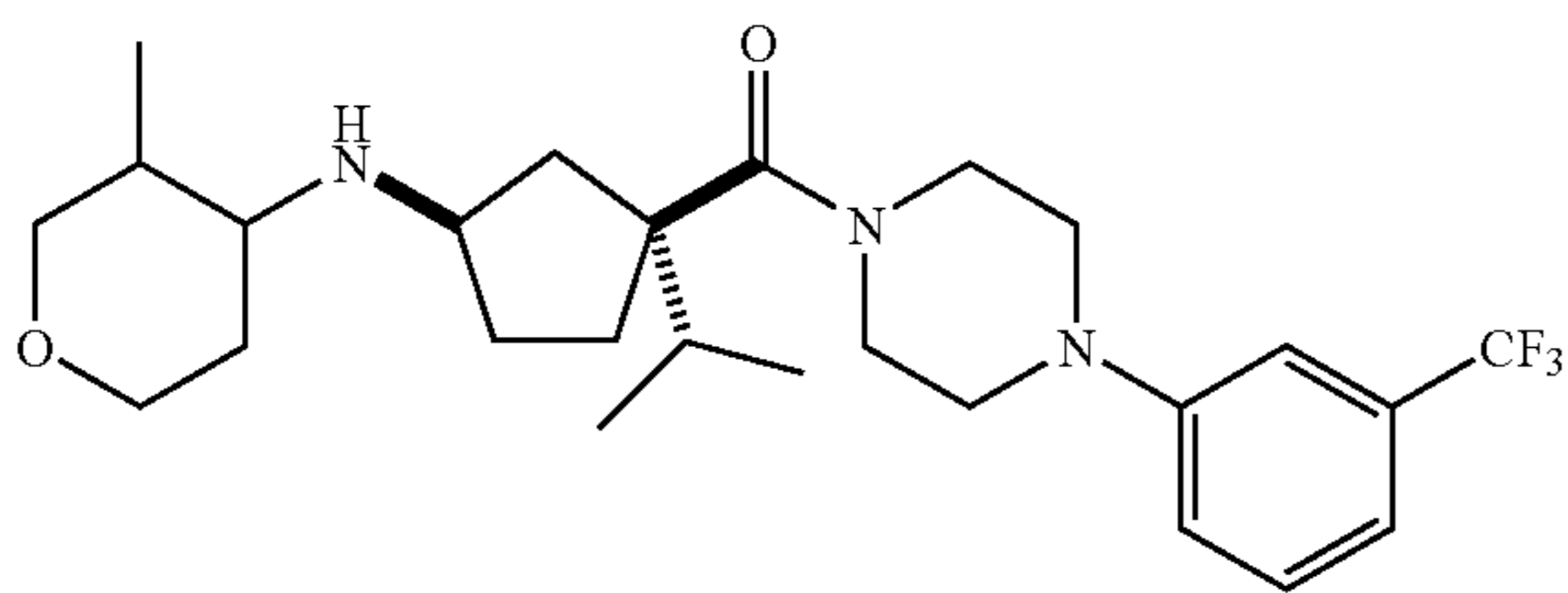
N -[(1 R ,3 S )-3-isopropyl-3-({4-[3-(trifluoromethyl)phenyl]piperazin-1-yl}carbonyl)cyclopentyl]-3-methyltetrahydro-2H-pyran-4-amine
