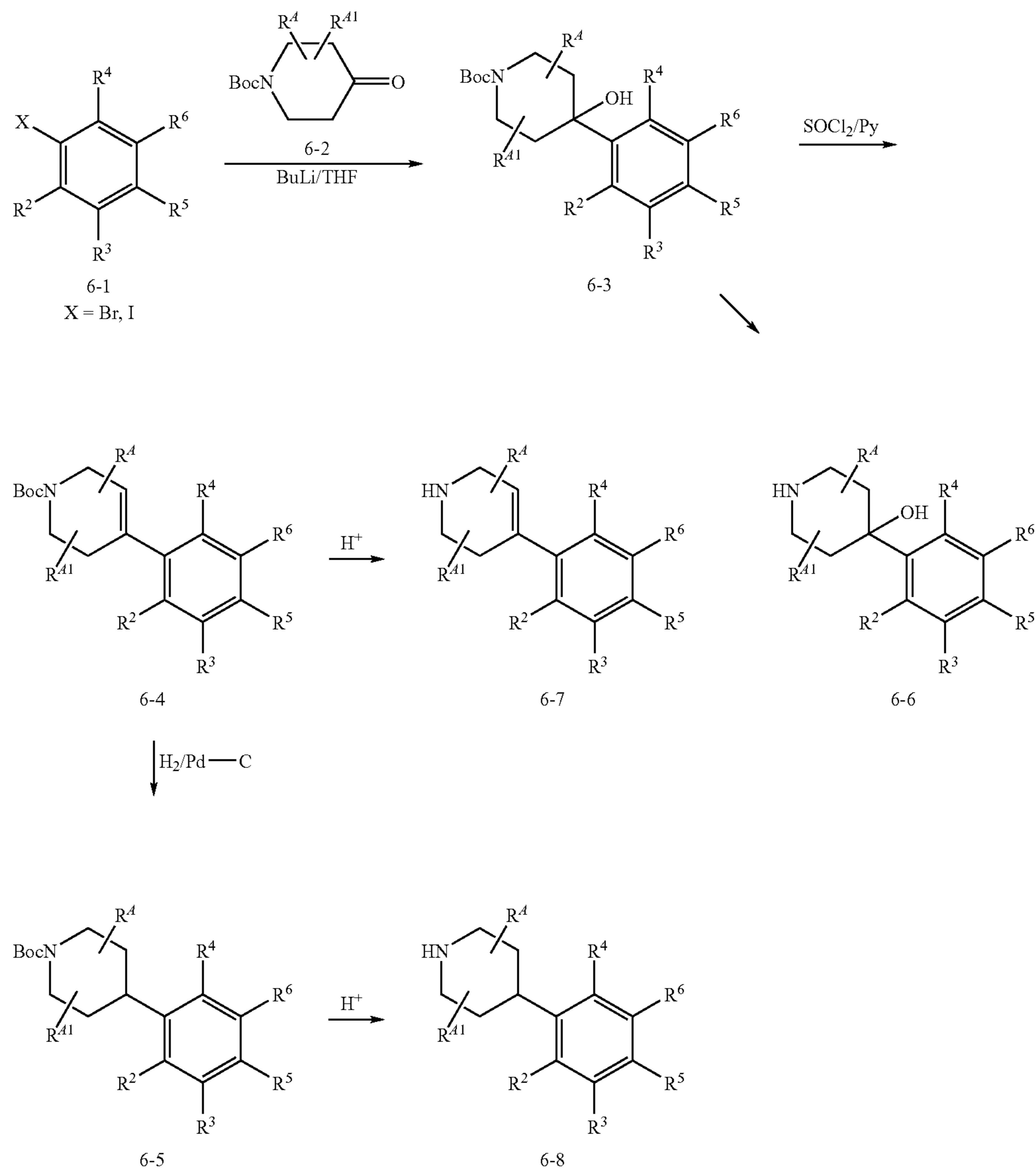
Scheme 6
