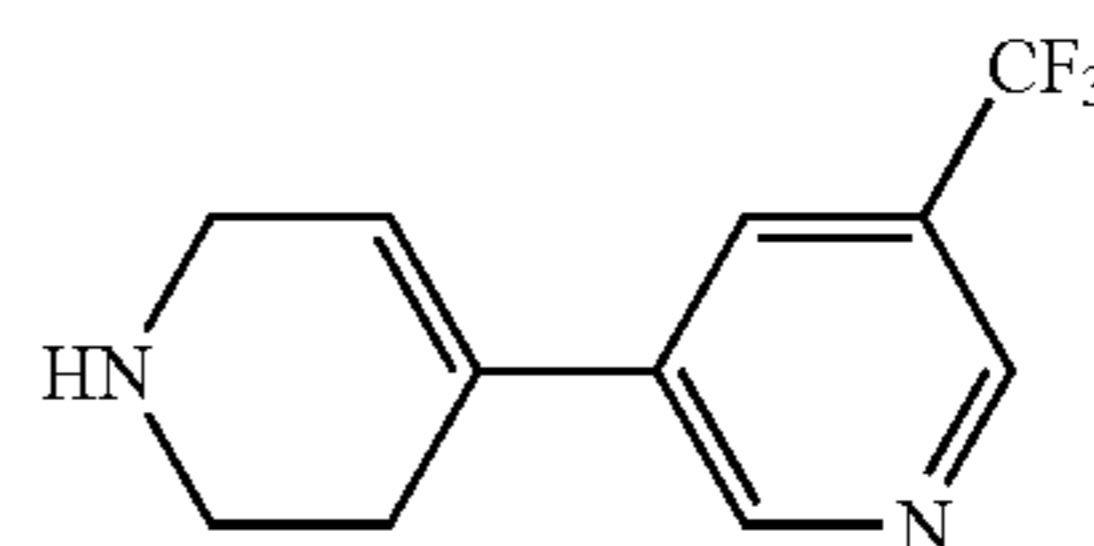
5-(Trifluoromethyl)-1',2',3',6'-tetrahydro-3,4'-bipyridine
