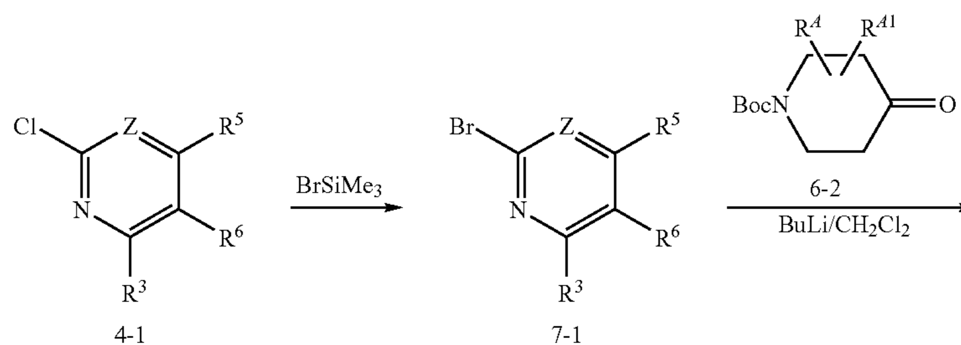
Scheme 7
