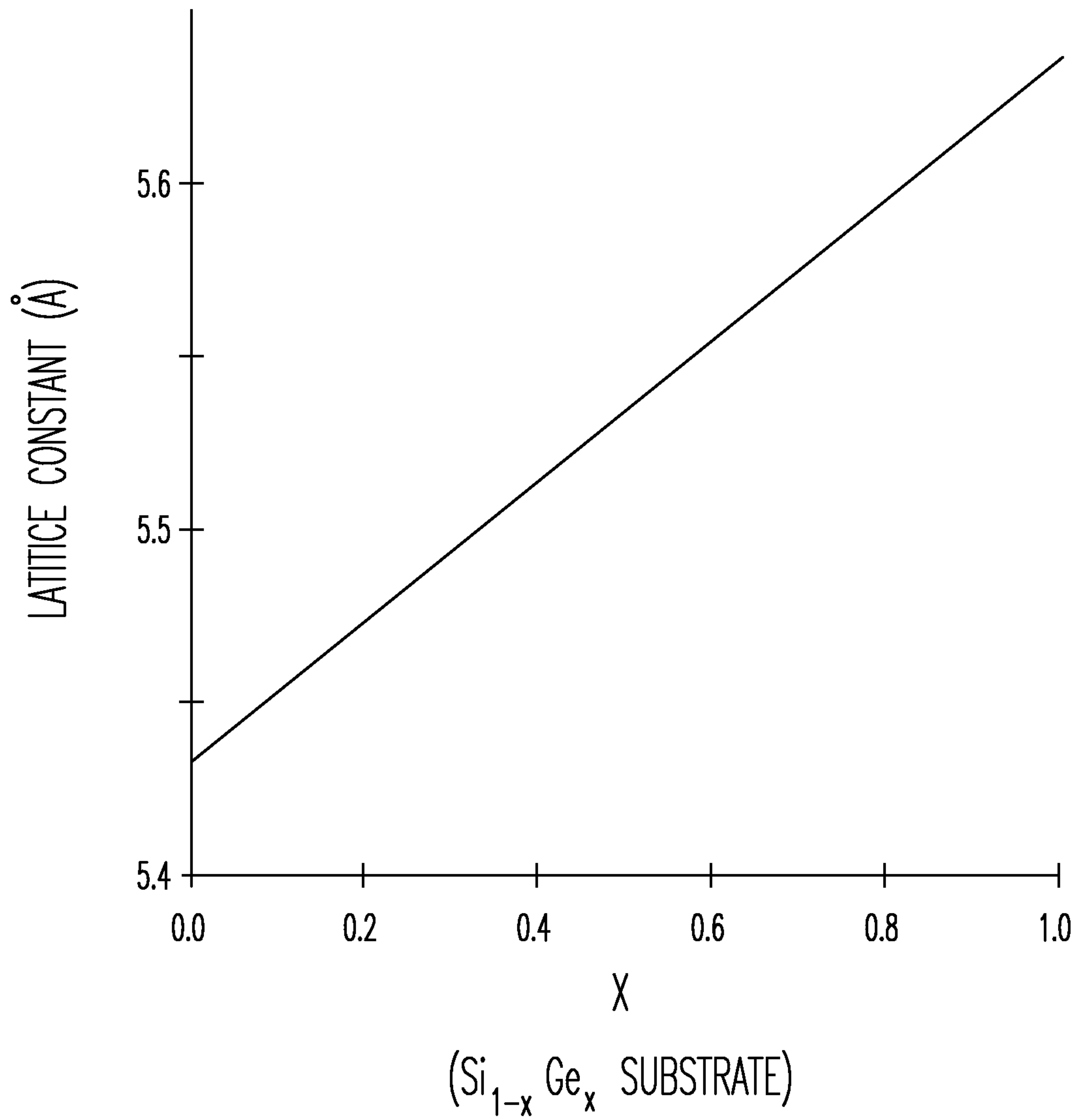
FIG. 1 (PRIOR ART)
