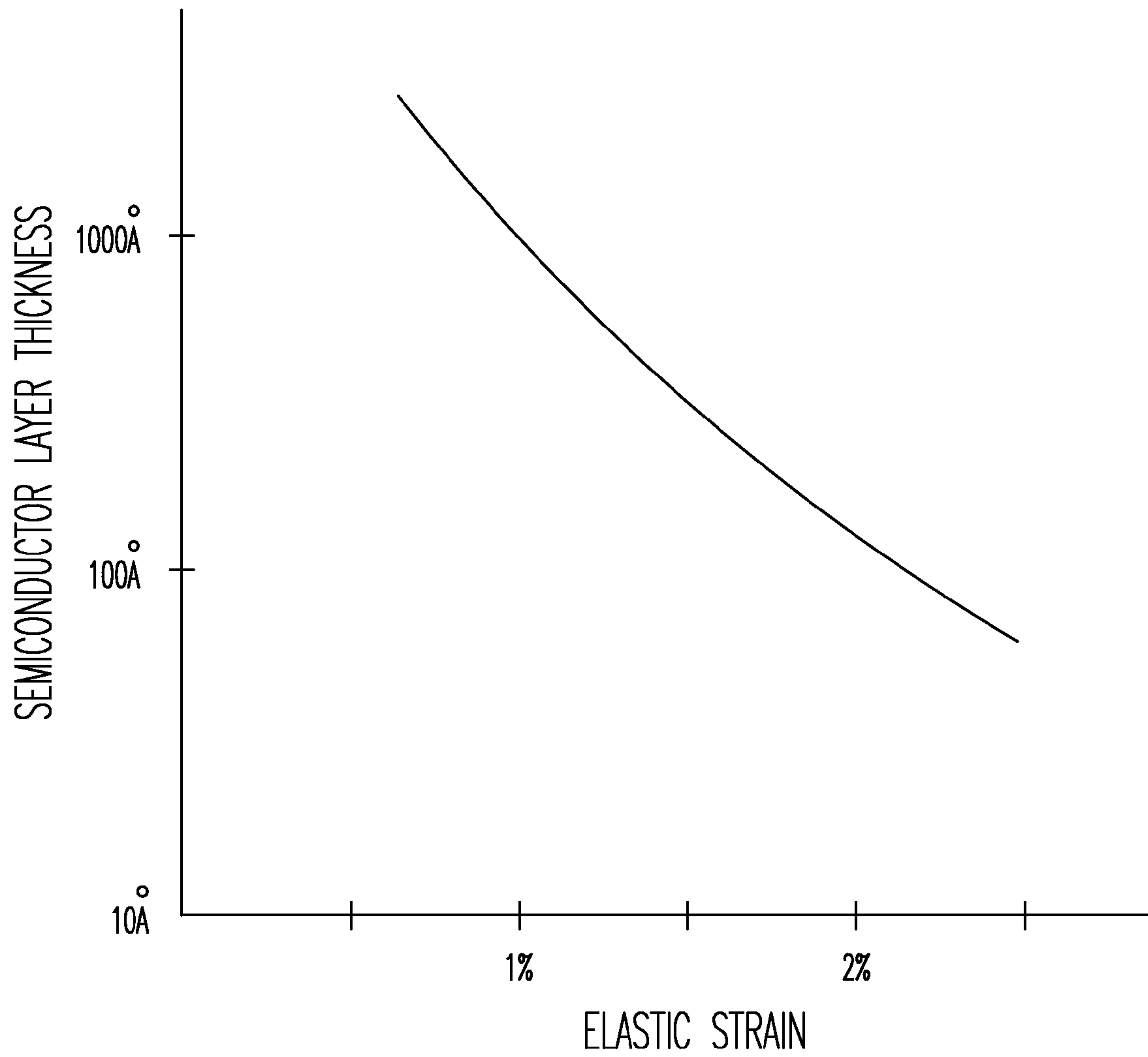
FIG. 3 (PRIOR ART)
