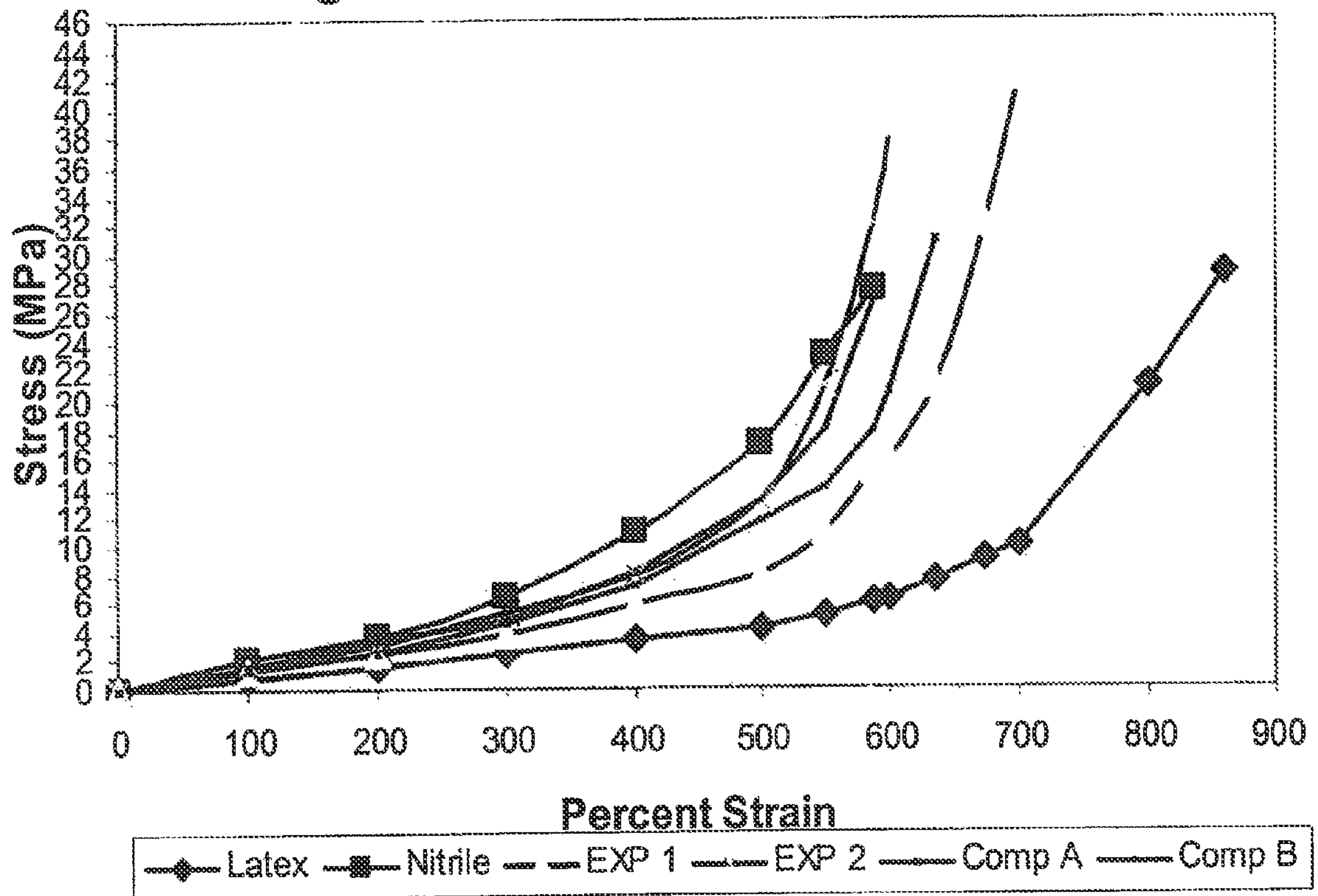
Figure 1 - Stress -Strain Curves
