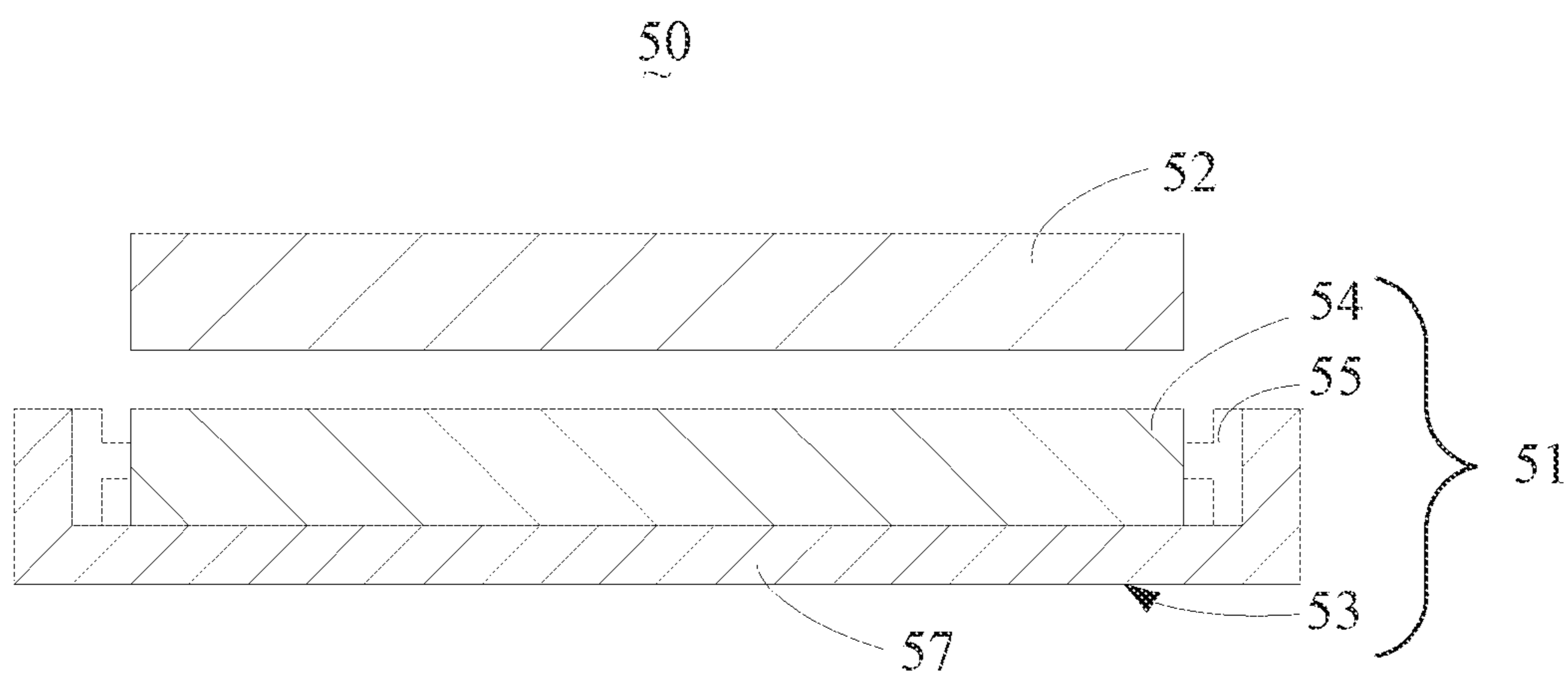
FIG. 20 (Prior Art)
