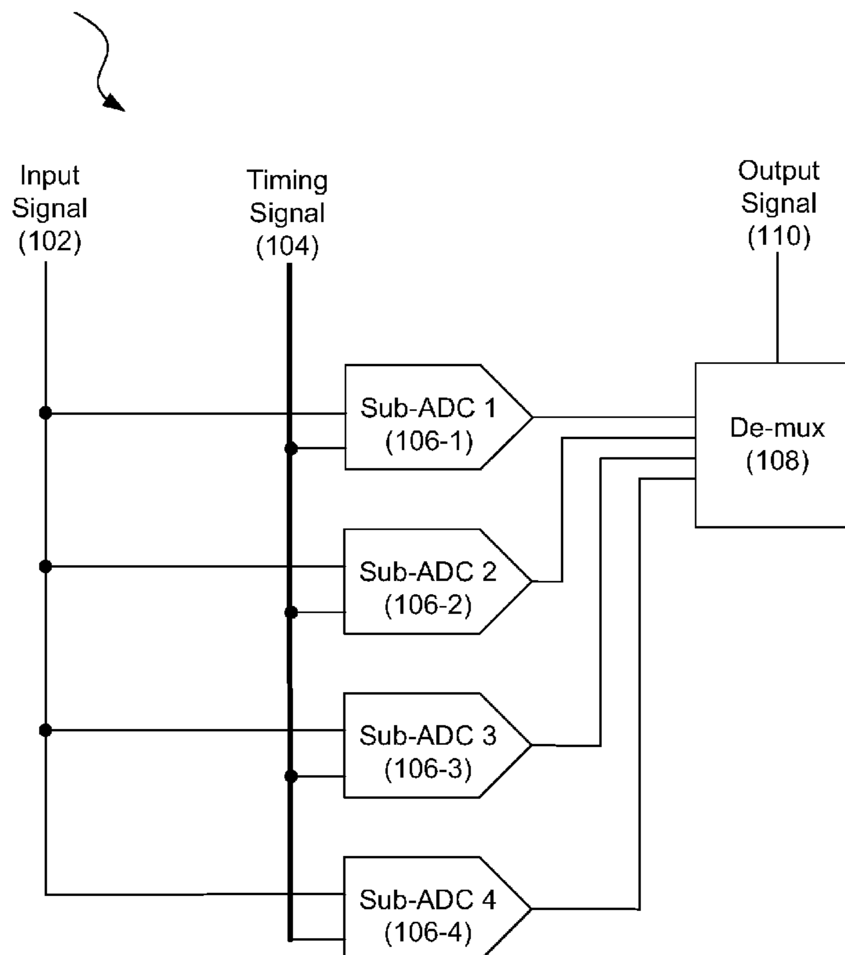
Time-interleaved ADC (100)
