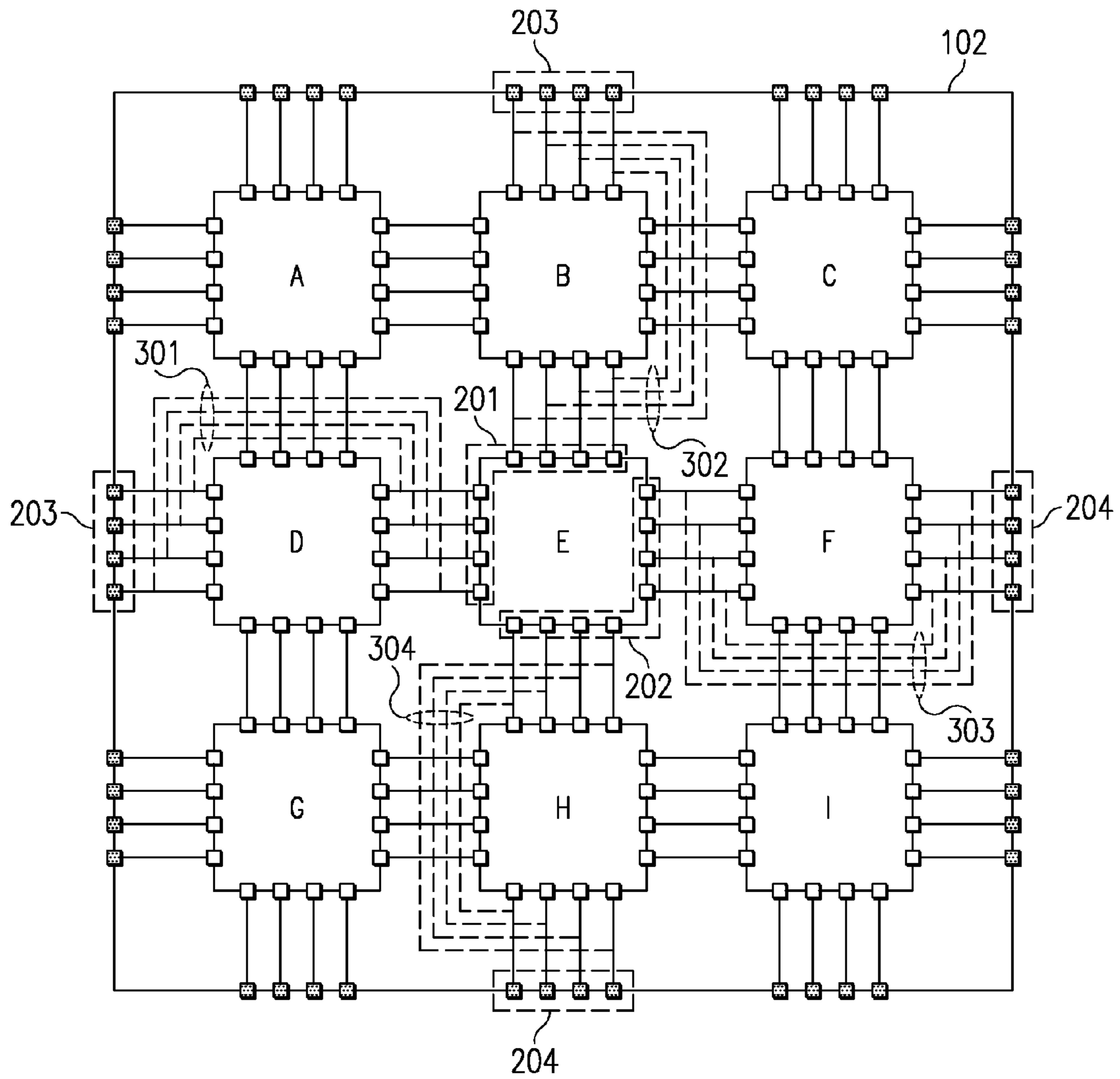
FIG. 3 (PRIOR ART)
