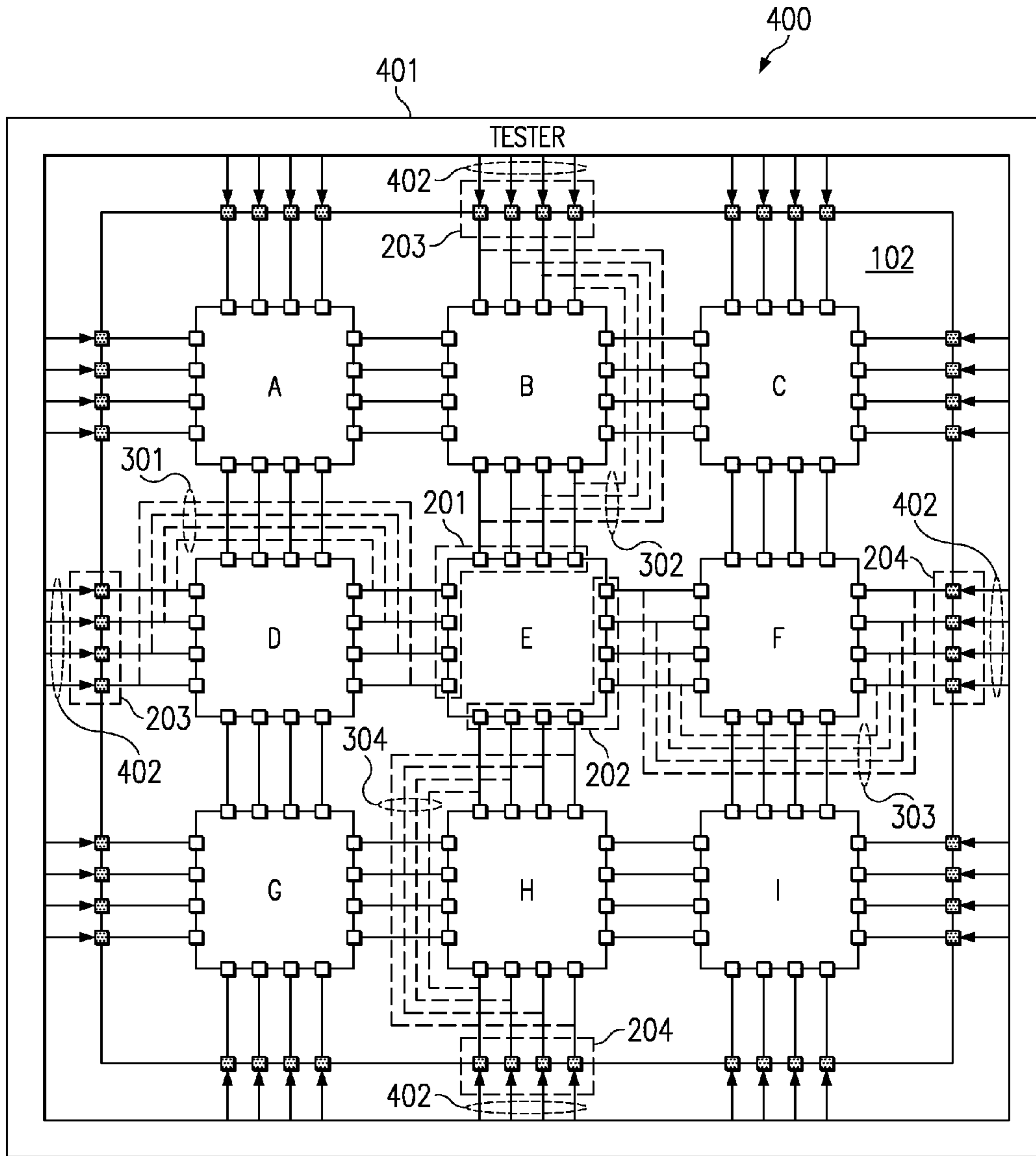
FIG. 4 (PRIOR ART)
