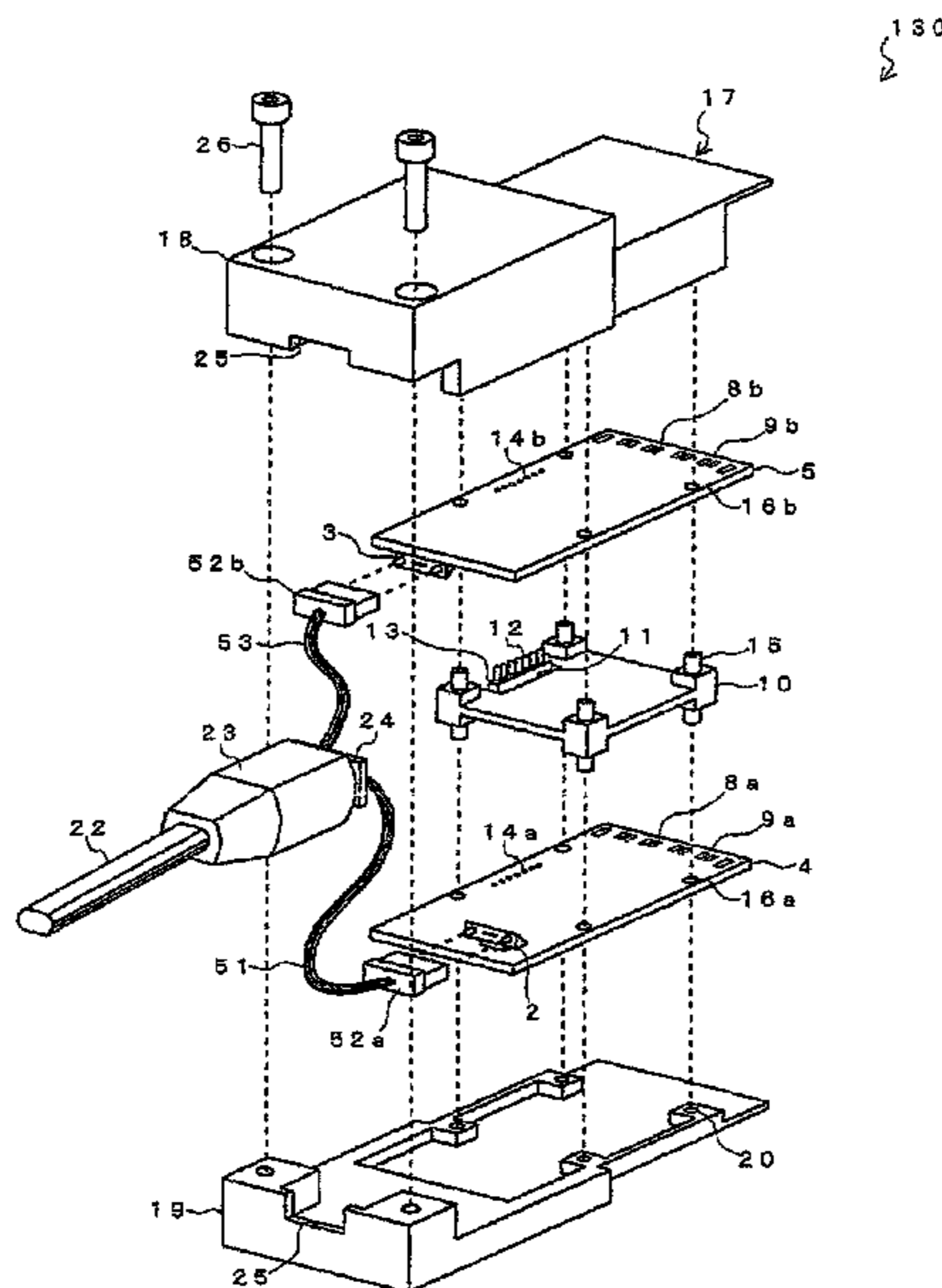
2 TRANSMISSION SIDE PHOTOELECTRIC CONVERSION PART 3 RECEPTION SIDE PHOTOELECTRIC CONVERSION PART 4 TRANSMISSION SIDE CIRCUIT BOARD 5 RECEPTION SIDE CIRCUIT BOARD
