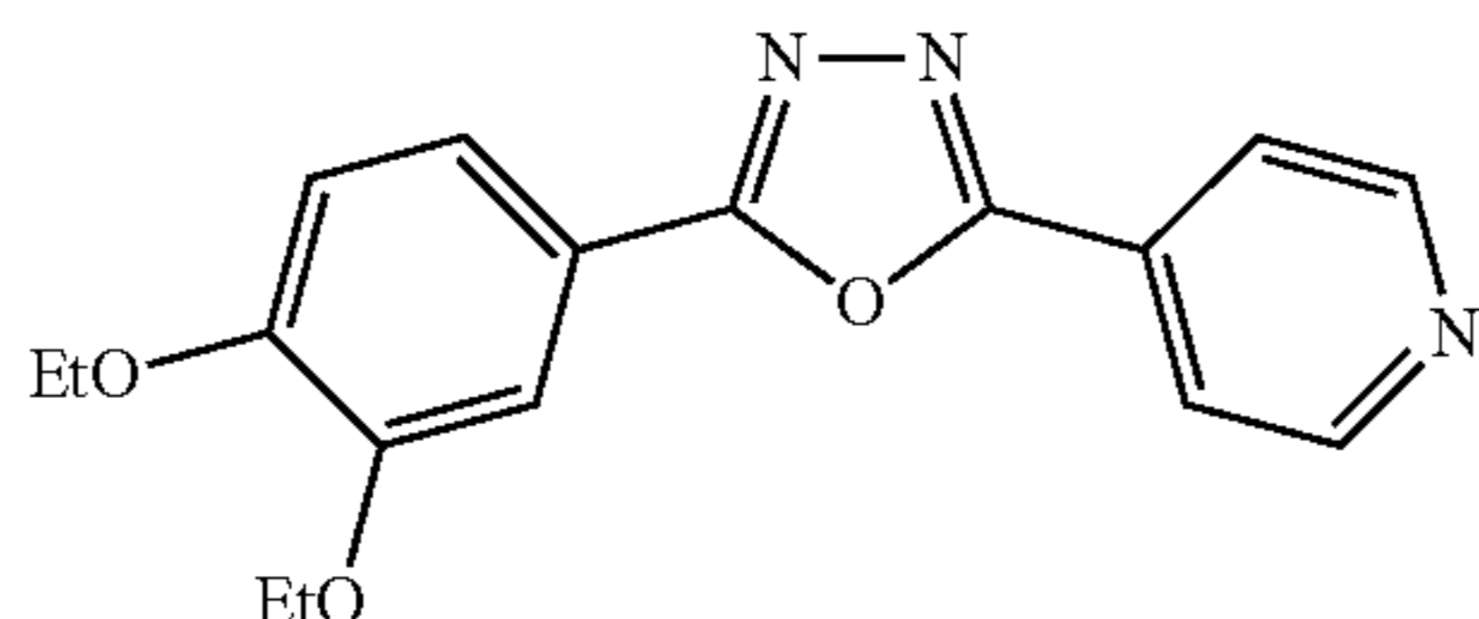
2-(3,4-diethoxyphenyl)-5-(pyridin-4-yl)-1,3,4-oxadiazole
