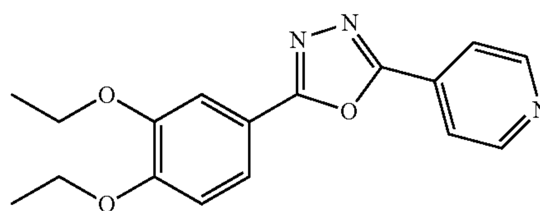
2-(3,4-diethoxyphenyl)-5-(pyridin-4-yl)-1,3,4-oxadiazole (25)
