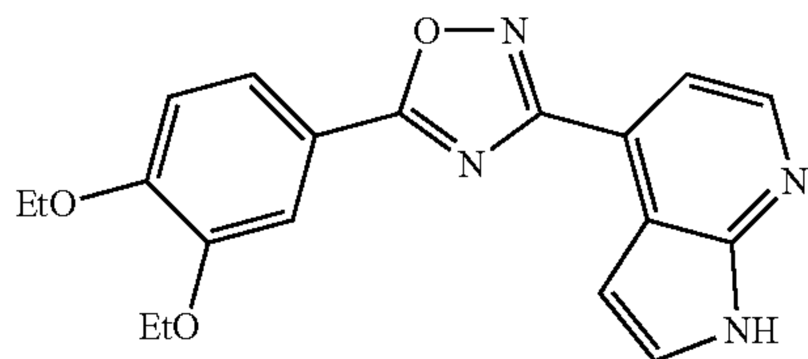
5-(3,4-diethoxyphenyl)-3-(1H-pyrrolo[2,3-b]pyridin-4-yl)-1,2,4-oxadiazole
