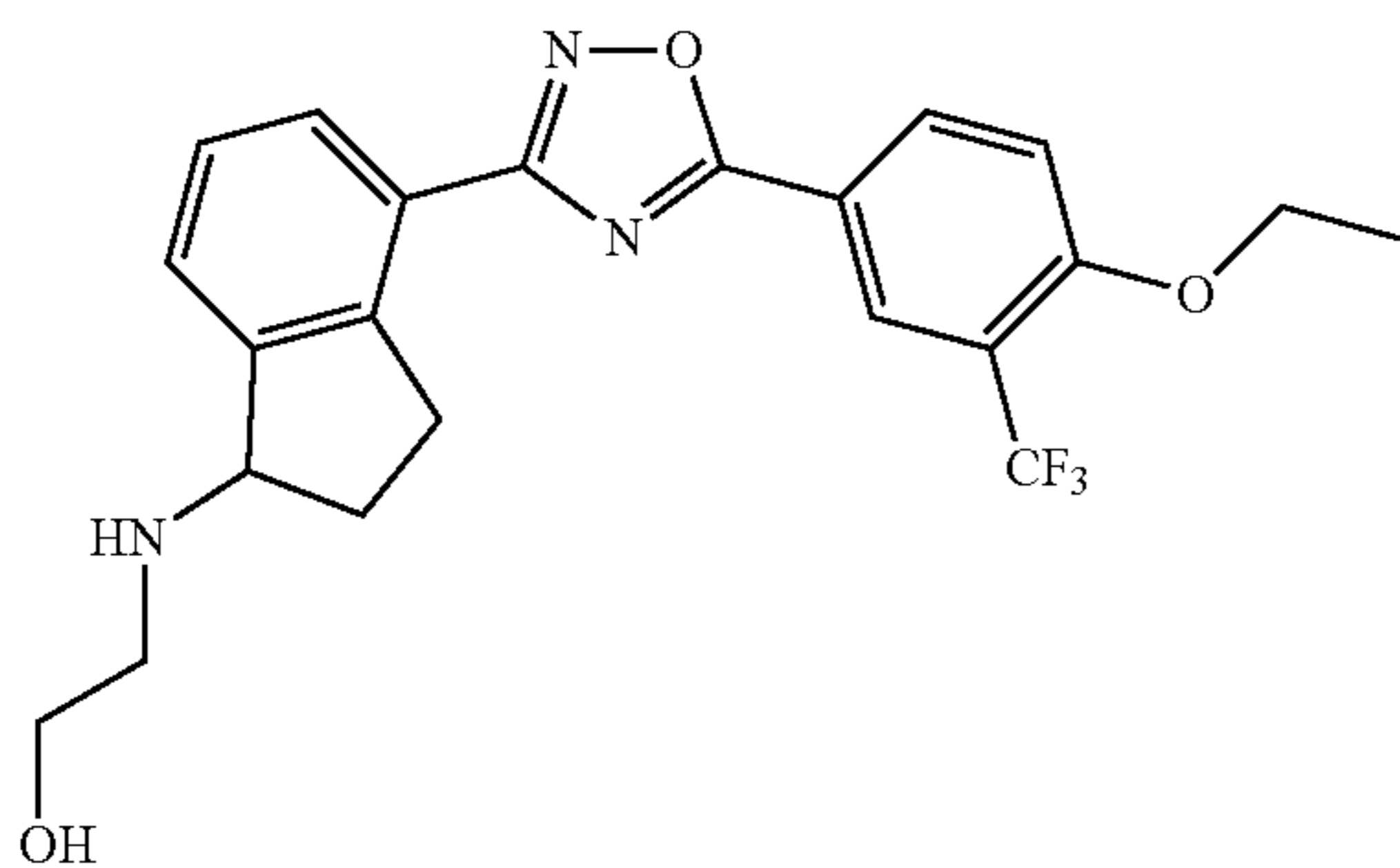
2-(4-(5-(4-ethoxy-3-(trifluoromethyl)phenyl)-1,2,4-oxadiazol-3-yl)-2,3-dihydro-1H-inden-1-ylamino)ethanol
