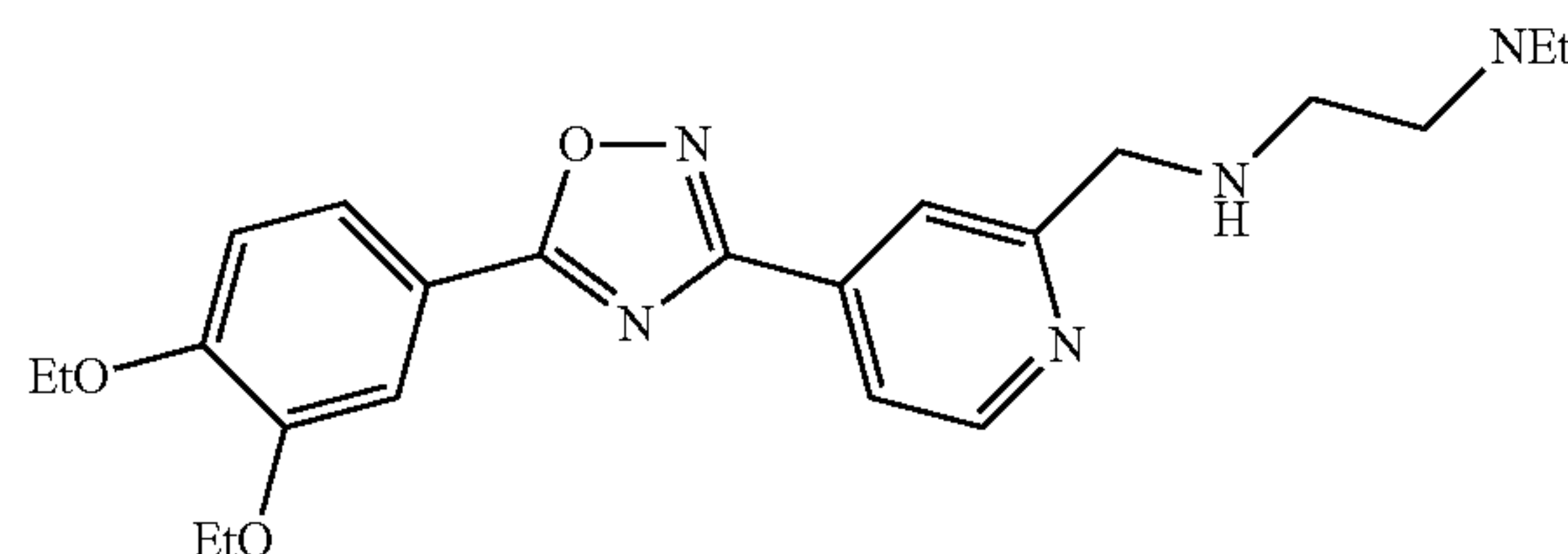
N1-((4-(5-(3,4-diethoxyphenyl)-1,2,4-oxadiazol-3-yl)pyridin-2-yl)methyl)-N2,N2-diethylethane-1,2-diamine
