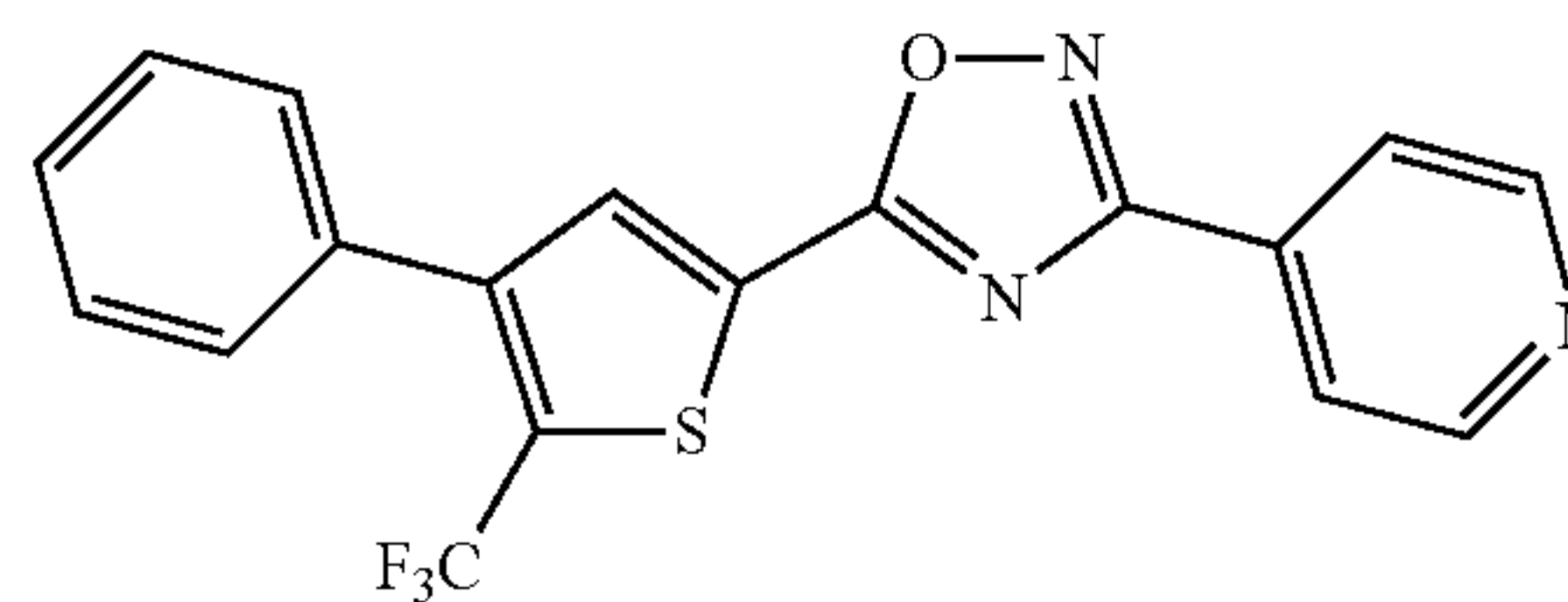
4-[5-(4-Phenyl-5-trifluoromethyl-thiophen-2-yl)-[1,2,4]oxadiazol-3-yl]-pyridine
