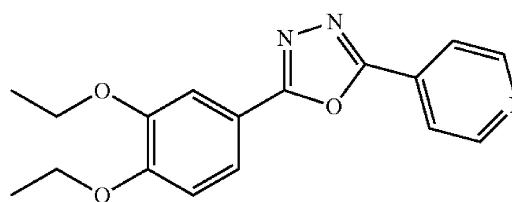
2-(3,4-diethoxyphenyl)-5-(pyridin-4-yl)-1,3,4-oxadiazole (25)
