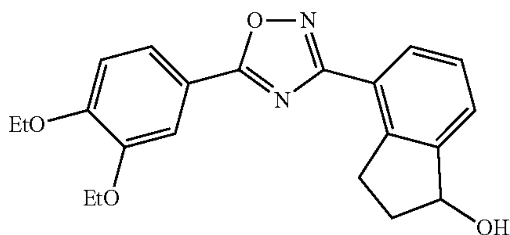
4-(5-(3,4-diethoxyphenyl)-1,2,4-oxadiazol-3-yl)-2,3-dihydro-1H-inden-1-ol
