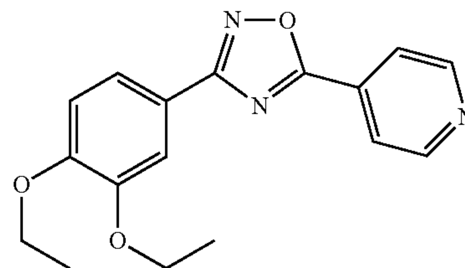
3-(3,4-diethoxyphenyl)-5-(pyridin-4-yl)-1,2,4-oxadiazole
