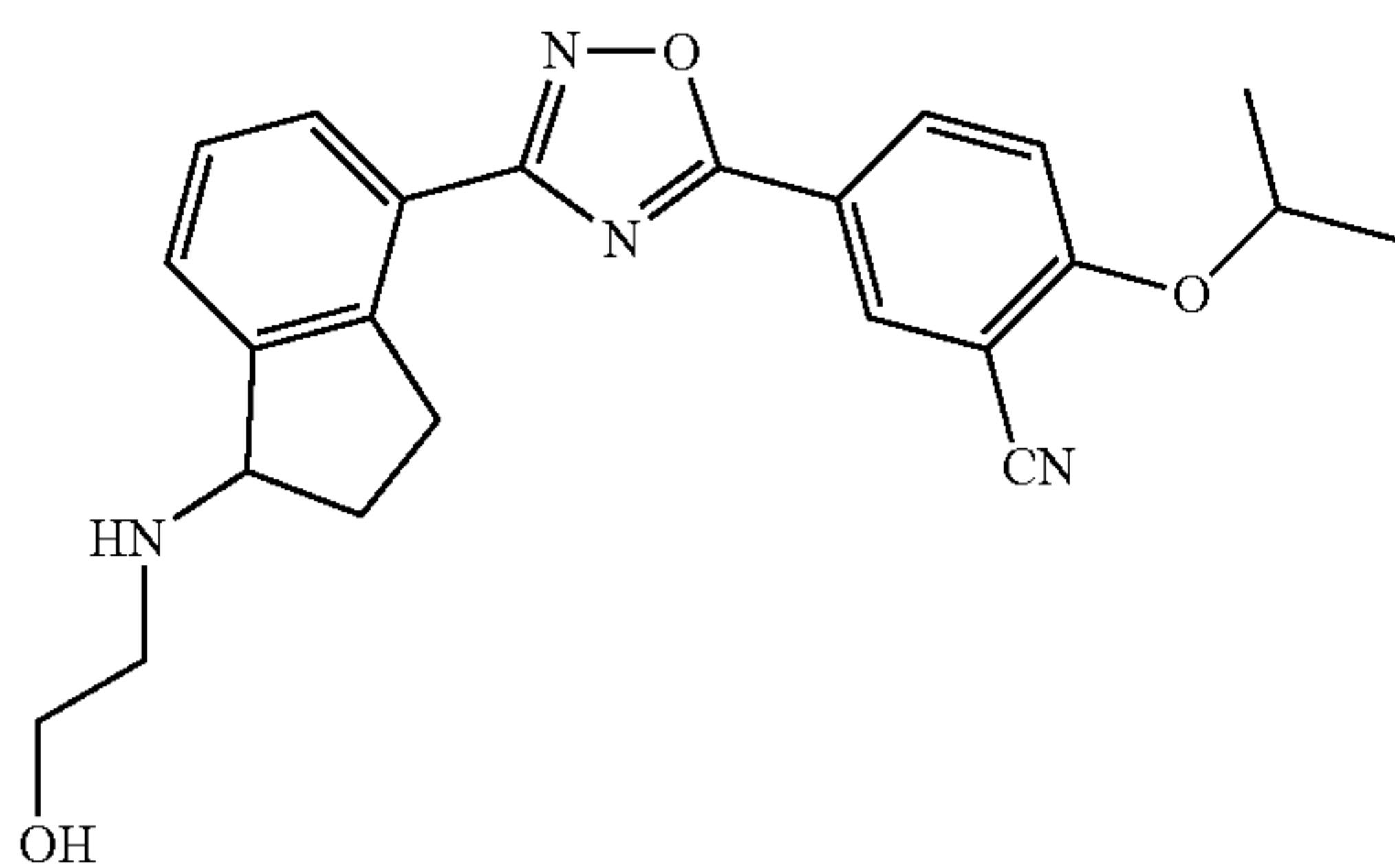
5-(3-(1-(2-hydroxyethylamino)-2,3-dihydro-1H-inden-4-yl)-1,2,4-oxadiazol-5-yl)-2-isopropoxybenzonitrile
