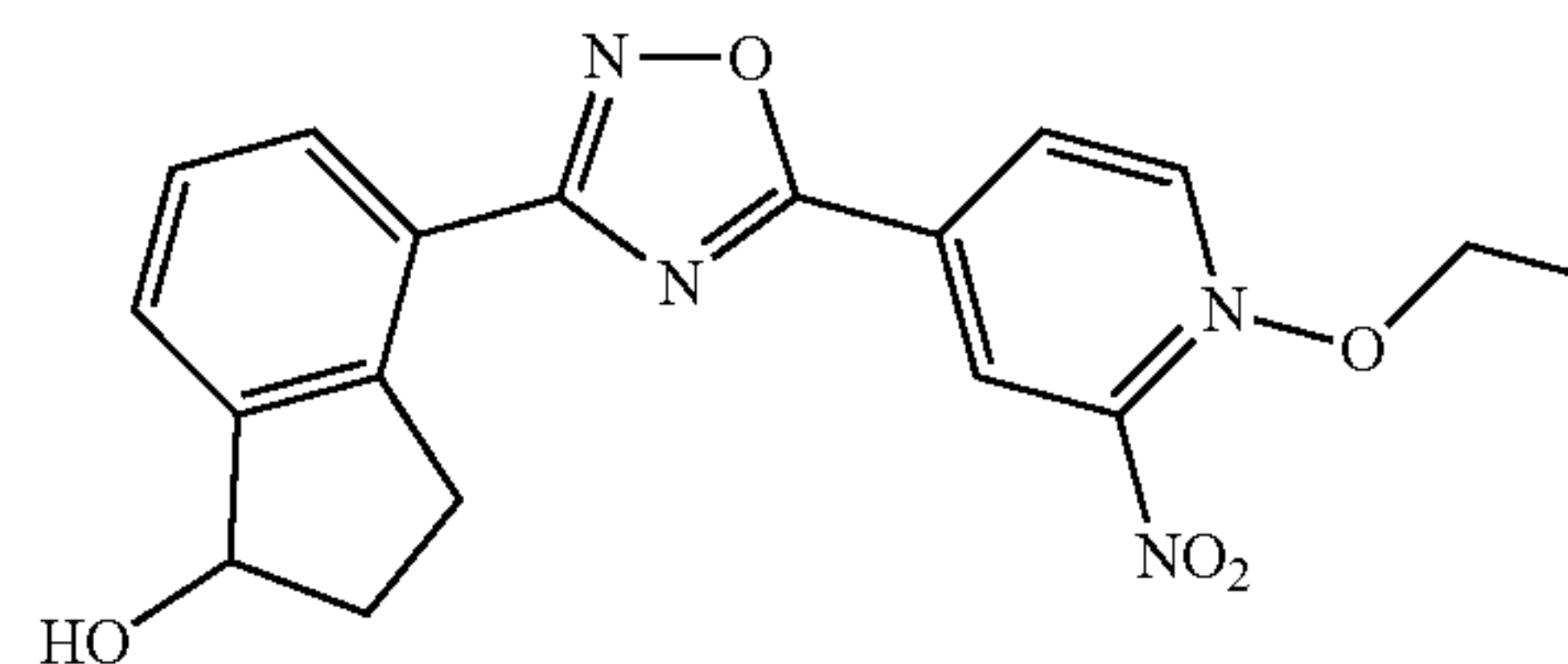
4-(5-(4-ethoxy-3-nitrophenyl)-1,2,4-oxadiazol-3-yl)-2,3-dihydro-1H-inden-1-ol
