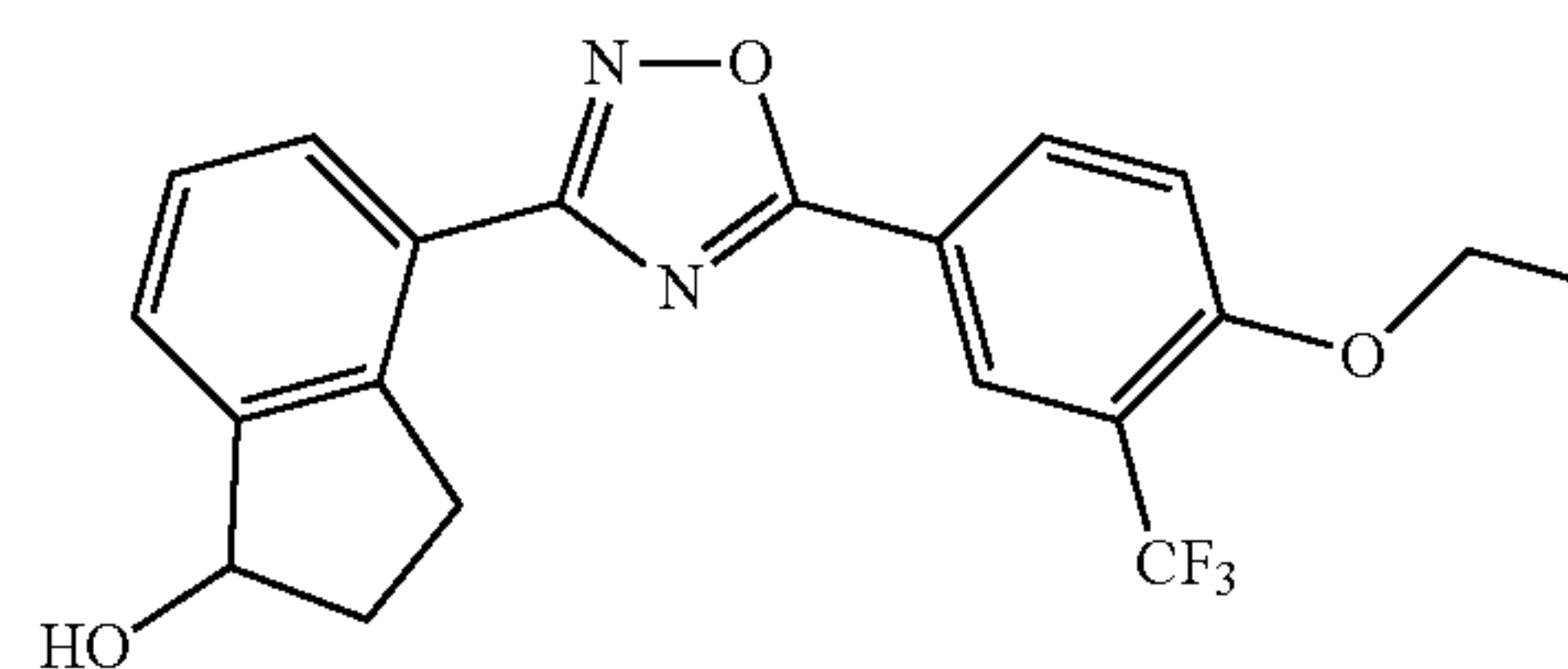
4-(5-(4-ethoxy-3-(trifluoromethyl)phenyl)-1,2,4-oxadiazol-3-yl)-2,3-dihydro-1H-inden-1-ol
