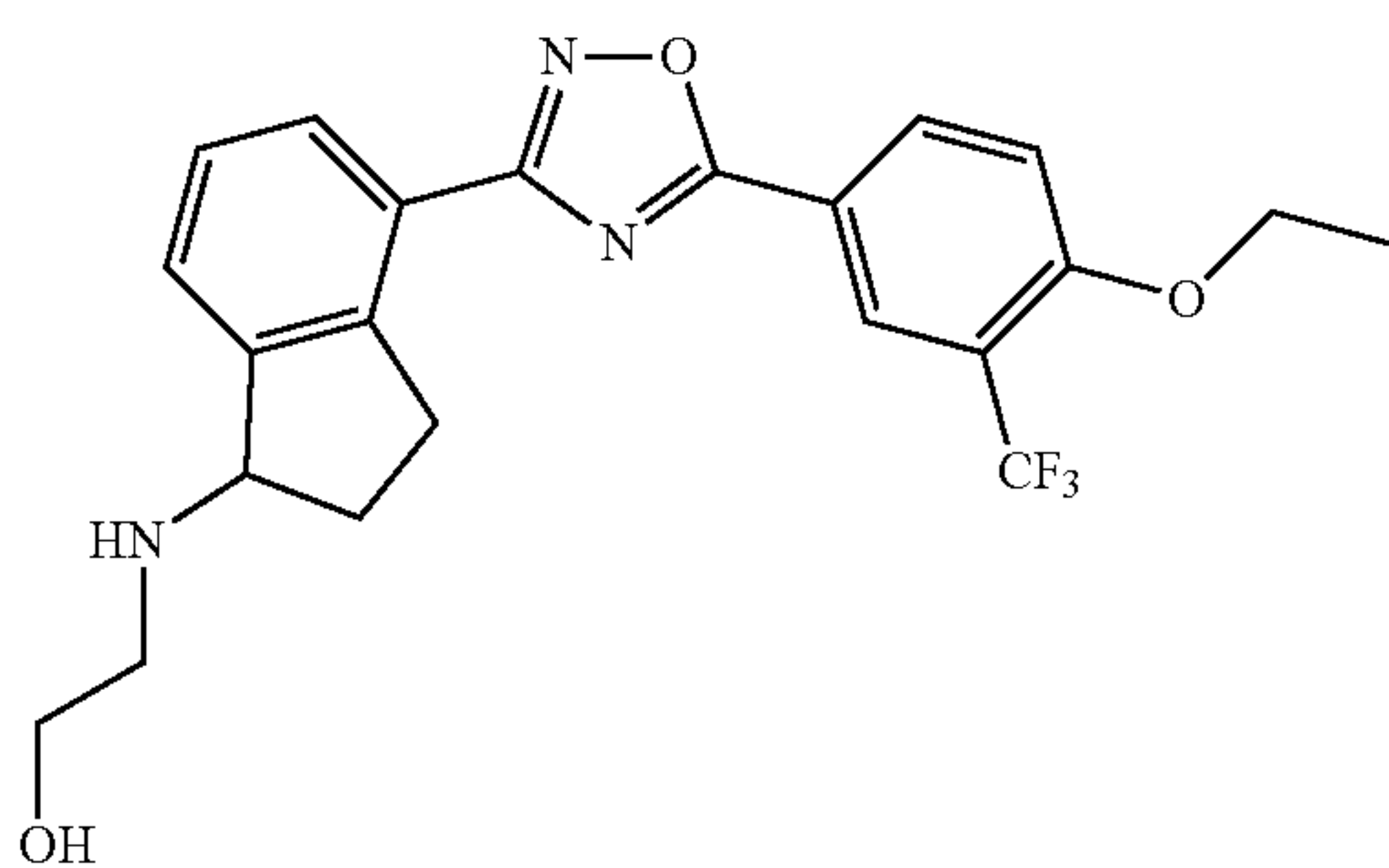
2-(4-(5-(4-ethoxy-3-(trifluoromethyl)phenyl)-1,2,4-oxadiazol-3-yl)-2,3-dihydro-1H-inden-1-ylamino)ethanol
