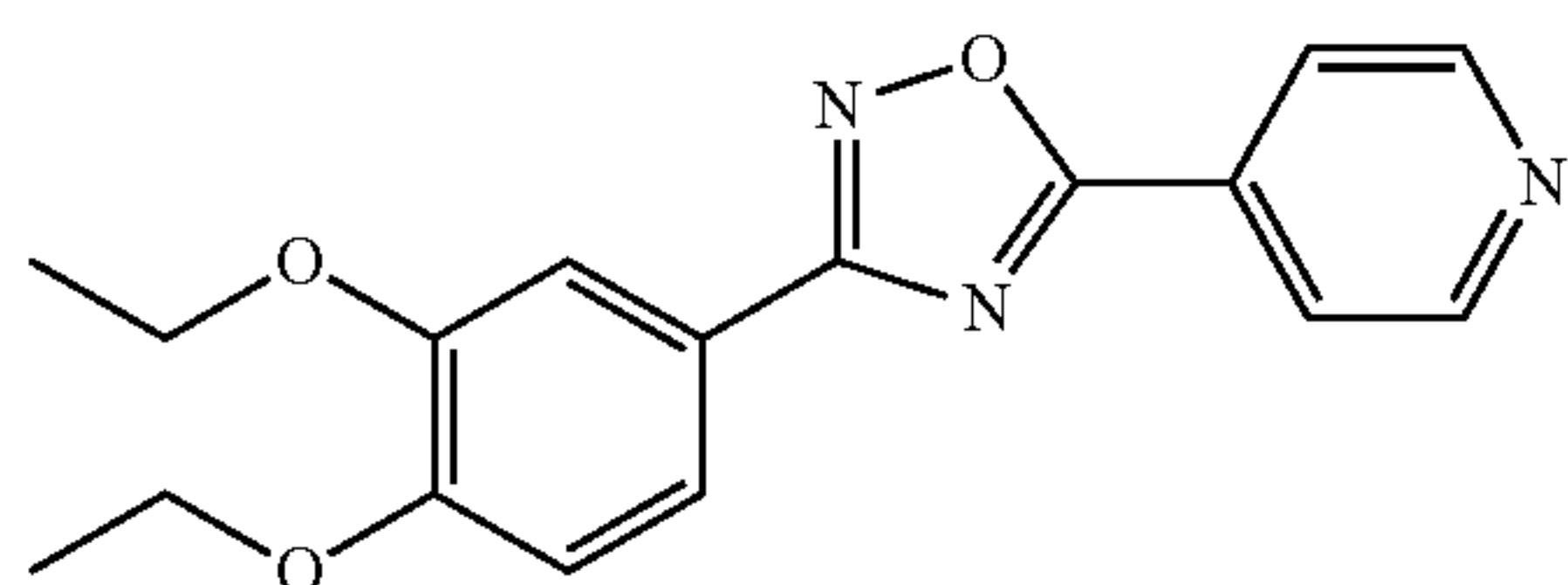
3-(3,4-diethoxyphenyl)-5-(pyridin-4-yl)-1,2,4-oxadiazole
