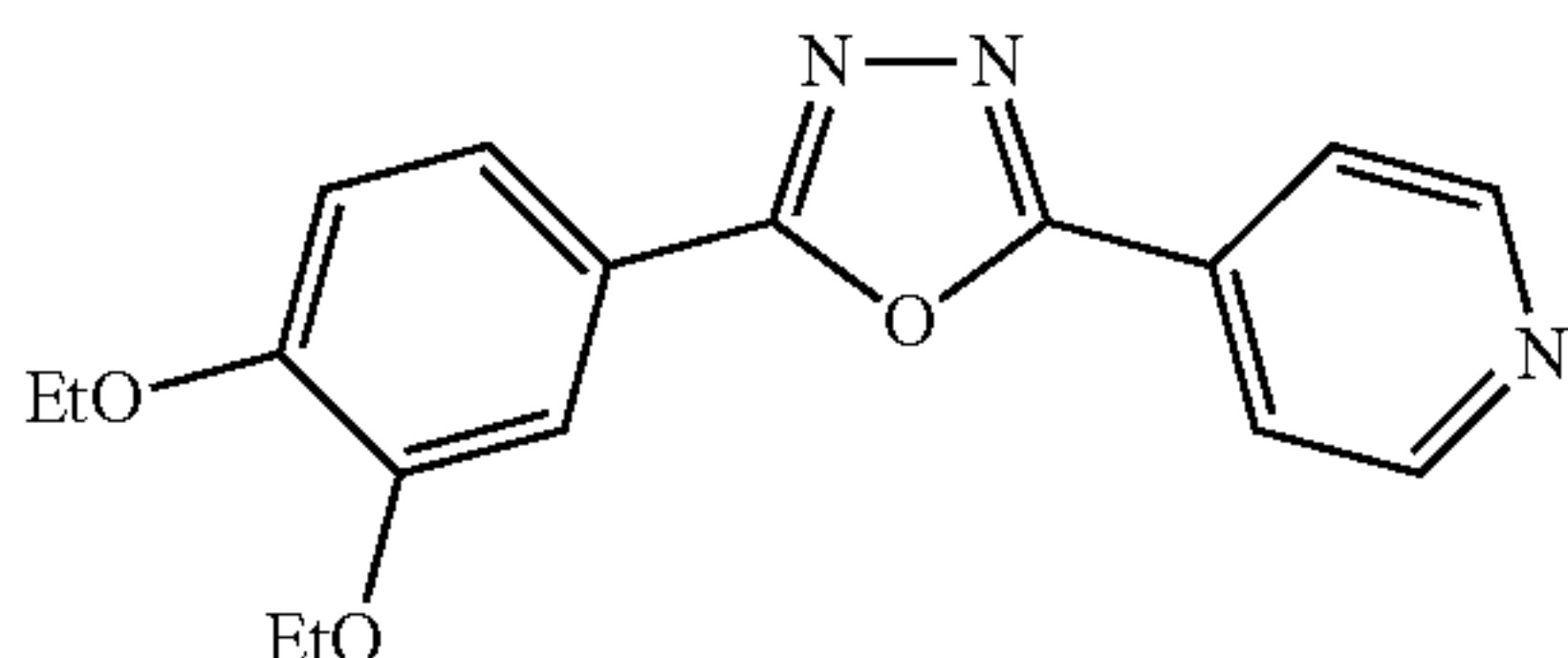
2-(3,4-diethoxyphenyl)-5-(pyridin-4-yl)-1,3,4-oxadiazole
