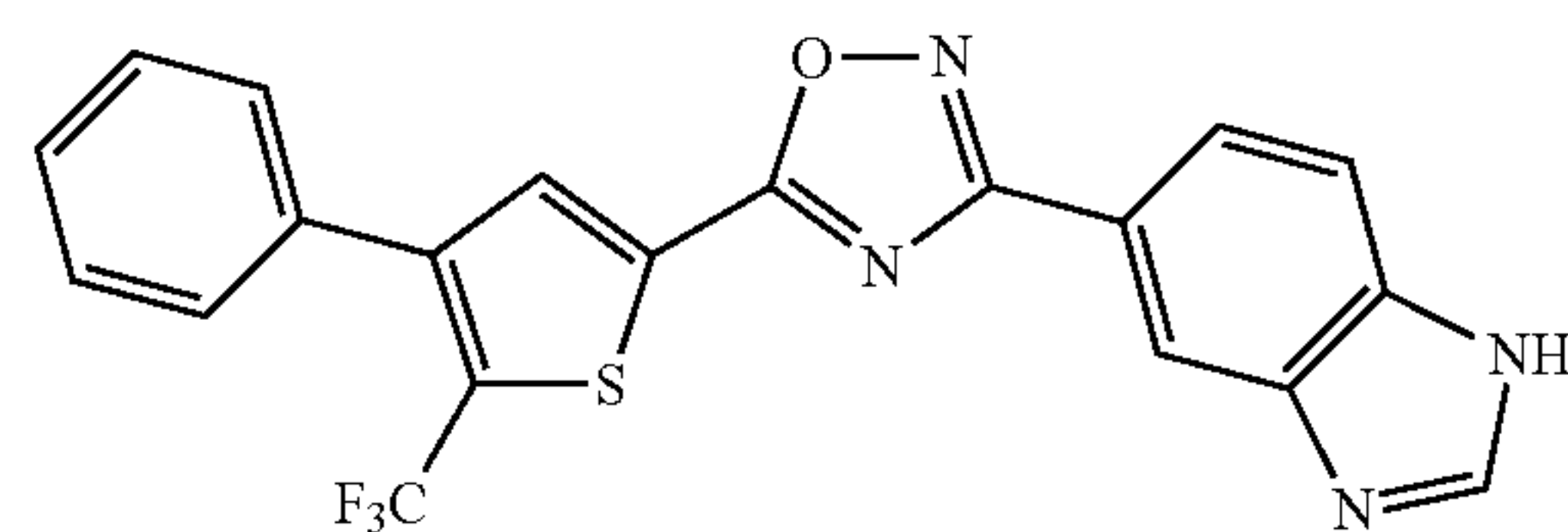
3-(1H-benzo[d]imidazol-5-yl)-5-(4-phenyl-5-(trifluoromethyl)thiophen-2-yl)-1,2,4-oxadiazole
