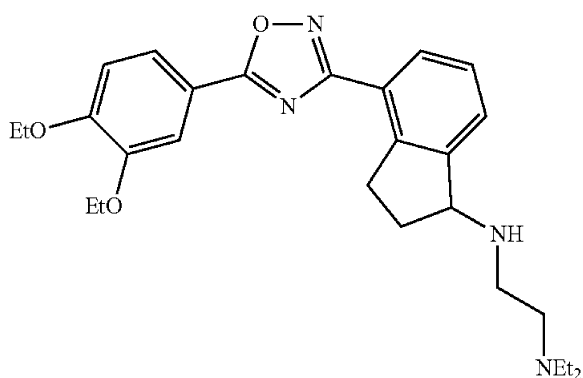
N1-(4-(5-(3,4-diethoxyphenyl)-1,2,4-oxadiazol-3-yl)- 2,3-dihydro-1H-inden-1-yl)-N2,N2-diethyl- ethane-1,2-diamine
