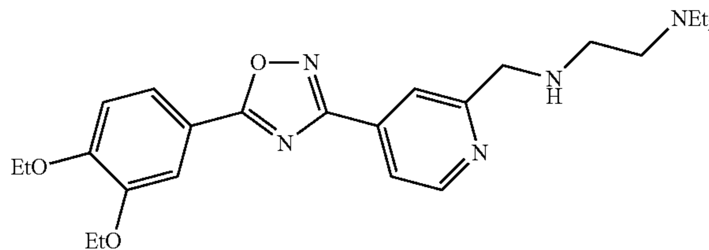
N1-((4-(5-(3,4-diethoxyphenyl)-1,2,4-oxadiazol-3-yl)pyridin-2-yl)methyl)-N2,N2-diethylethane-1,2-diamine
