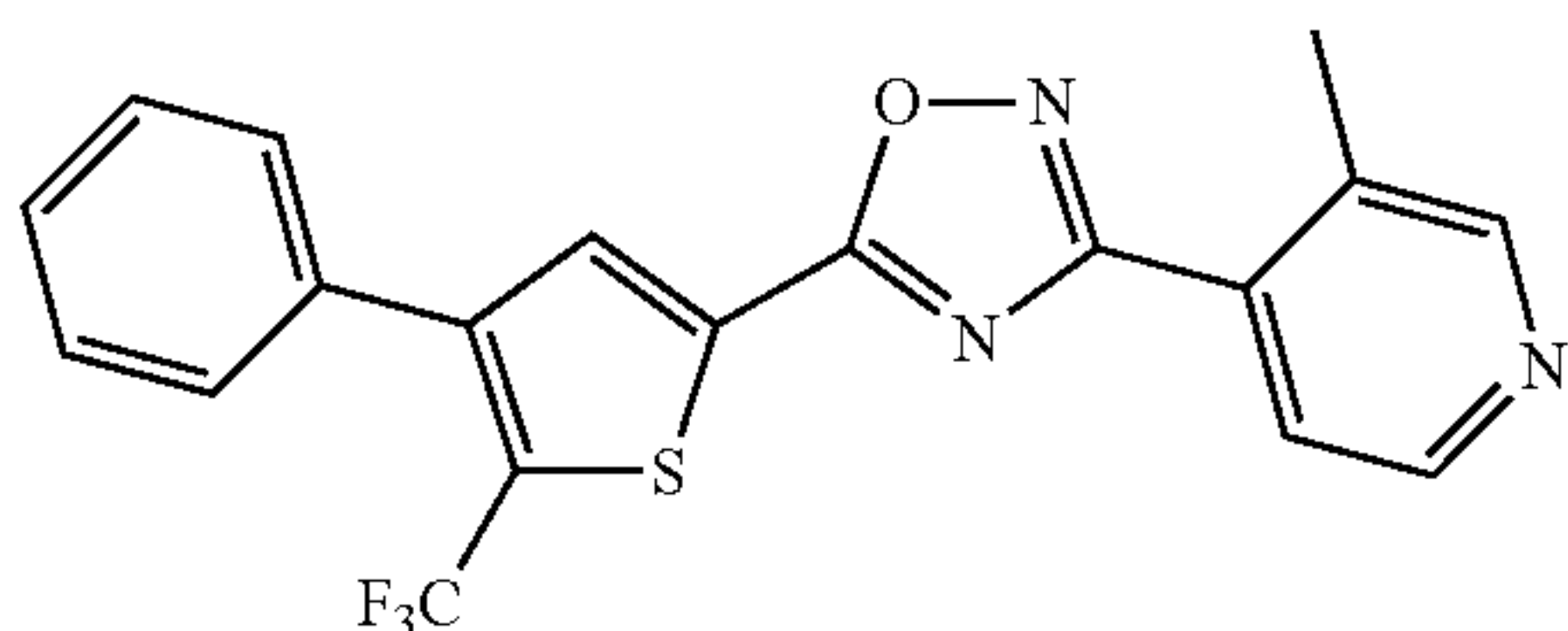
3-(3-methylpyridin-4-yl)-5-(4-phenyl-5-(trifluoromethyl)thiophen-2-yl)-1,2,4-oxadiazole
