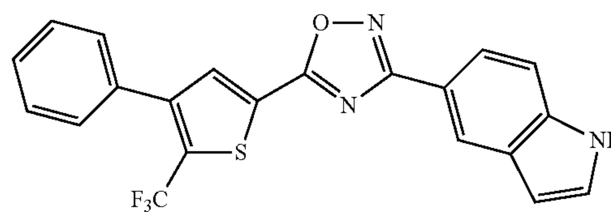
3-(1H-indol-5-yl)-5-(4-phenyl-5-(trifluoromethyl)thiophen-2-yl)-1,2,4-oxadiazole
