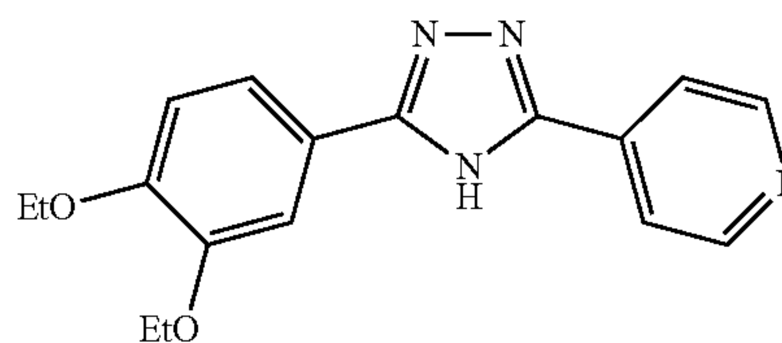
4-(5-(3,4-diethoxyphenyl)-4H-1,2,4-triazol-3-yl)pyridine
