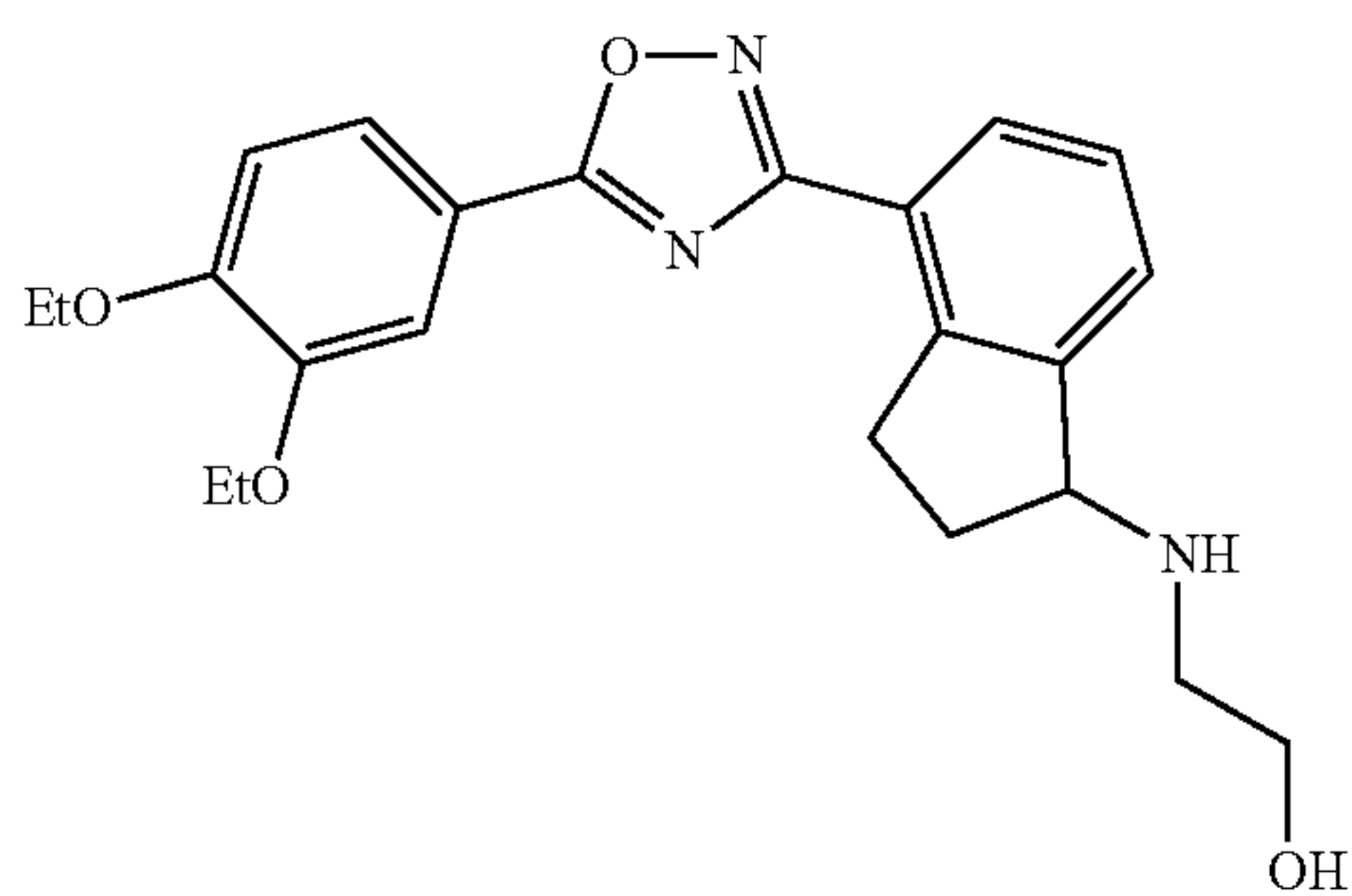
2-(4-(5-(3,4-diethoxyphenyl)-1,2,4-oxadiazol-3-yl)- 2,3-dihydro-1H-inden-1-ylamino)ethanol
