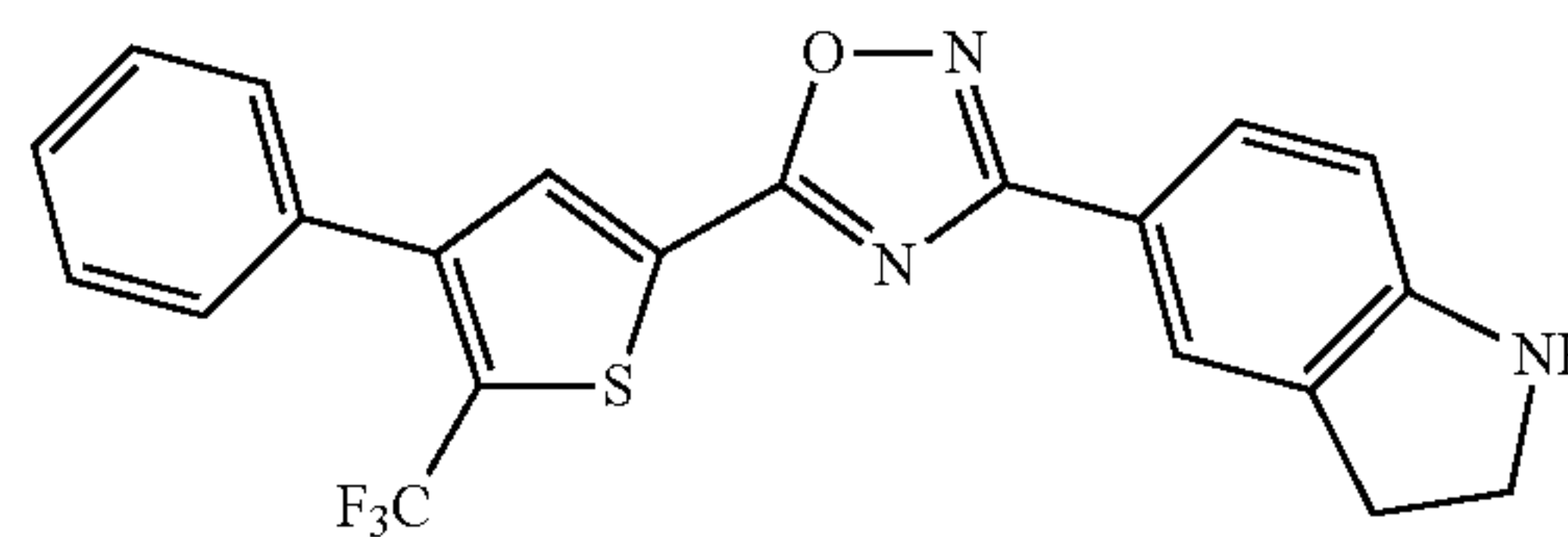
3-(indolin-5-yl)-5-(4-phenyl-5-(trifluoromethyl)thiophen-2-yl)-1,2,4-oxadiazole
