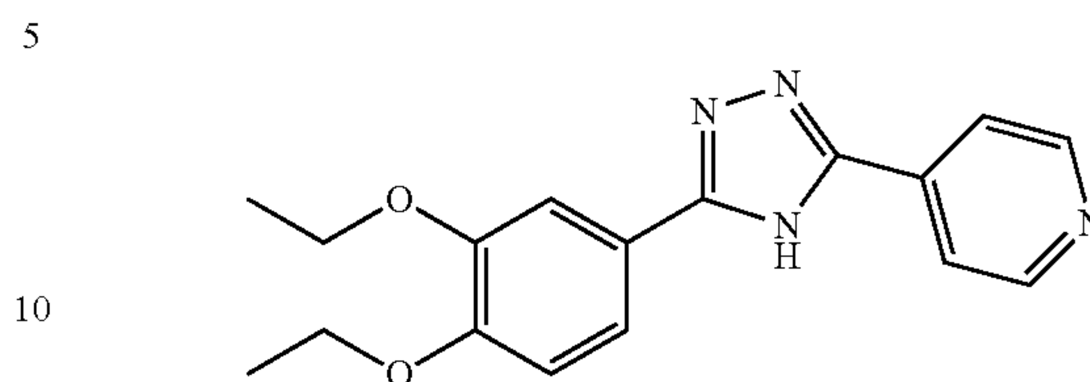
4-(5-(3,4-diethoxyphenyl)-4H-1,2,4-triazol-3-yl)pyridine
