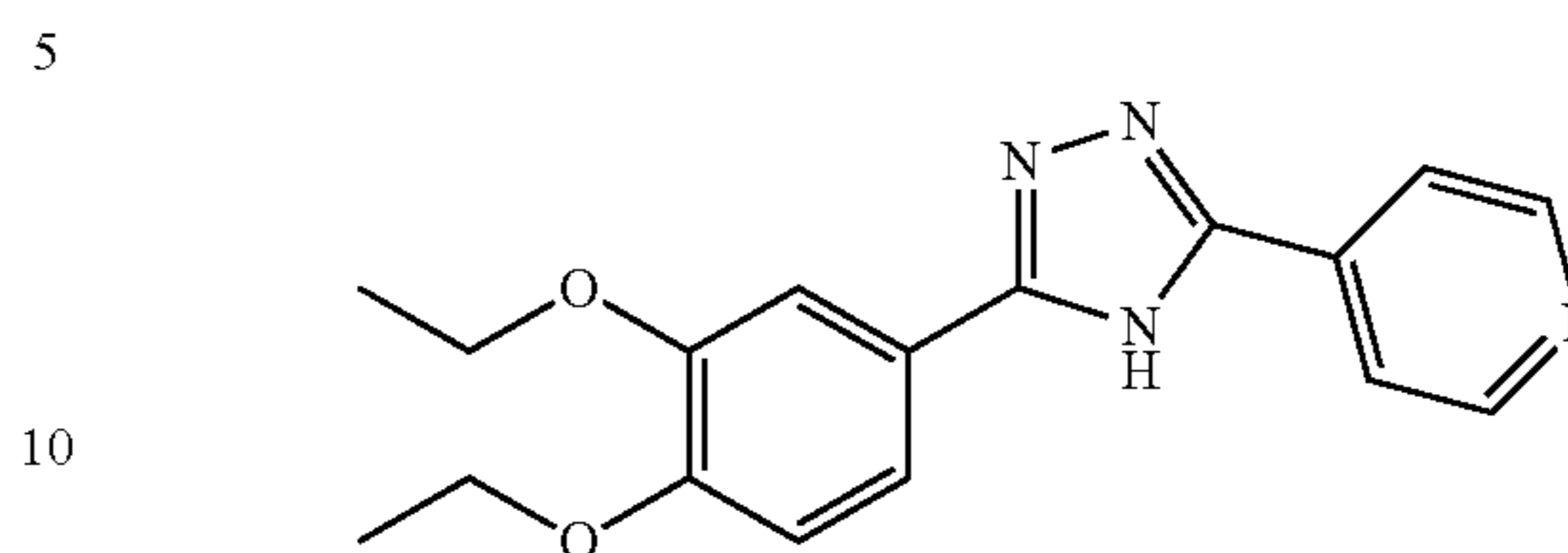
4-(5-(3,4-diethoxyphenyl)-4H-1,2,4-triazol-3-yl)pyridine
