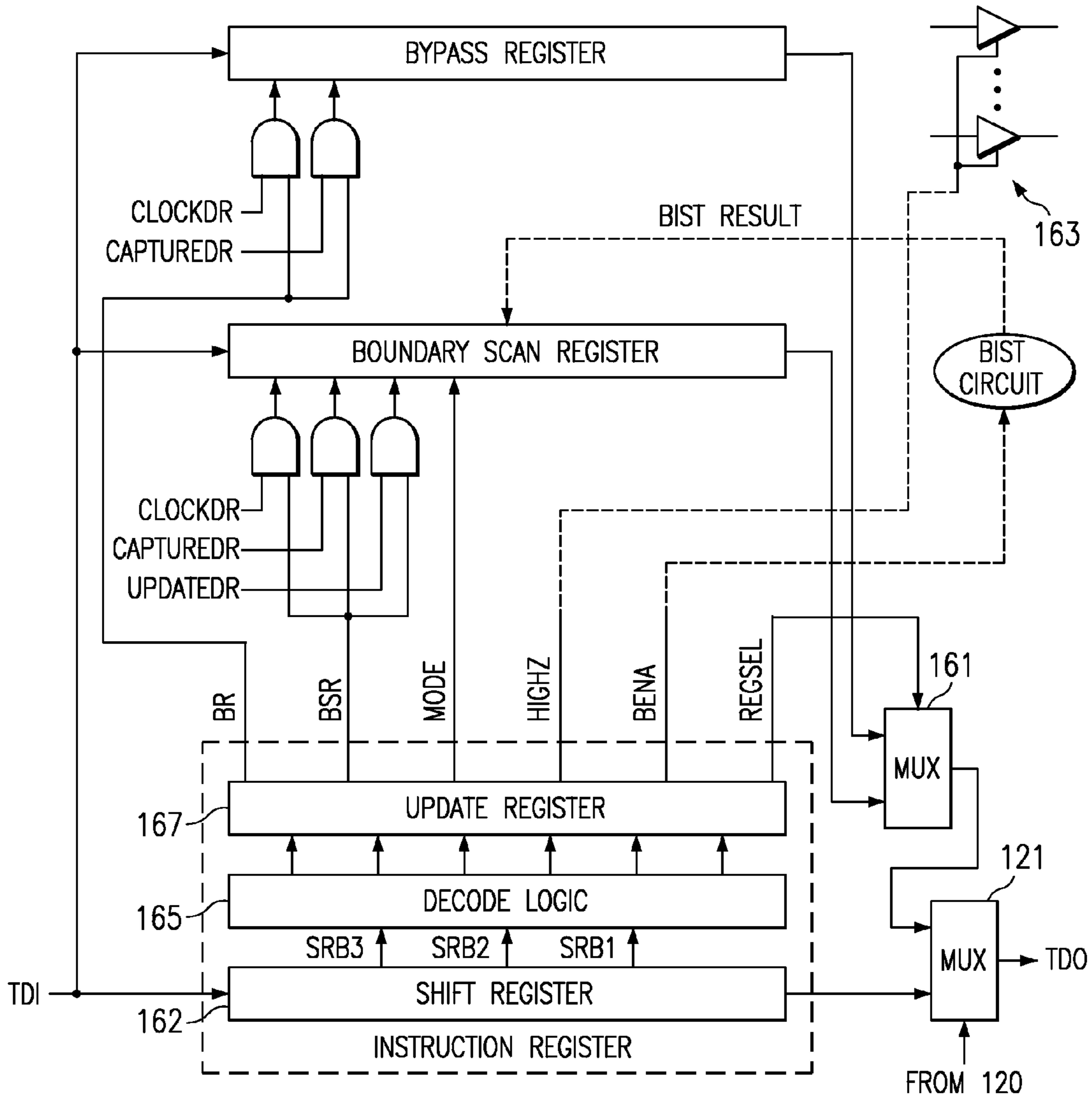
FIG. 16 (PRIOR ART)
