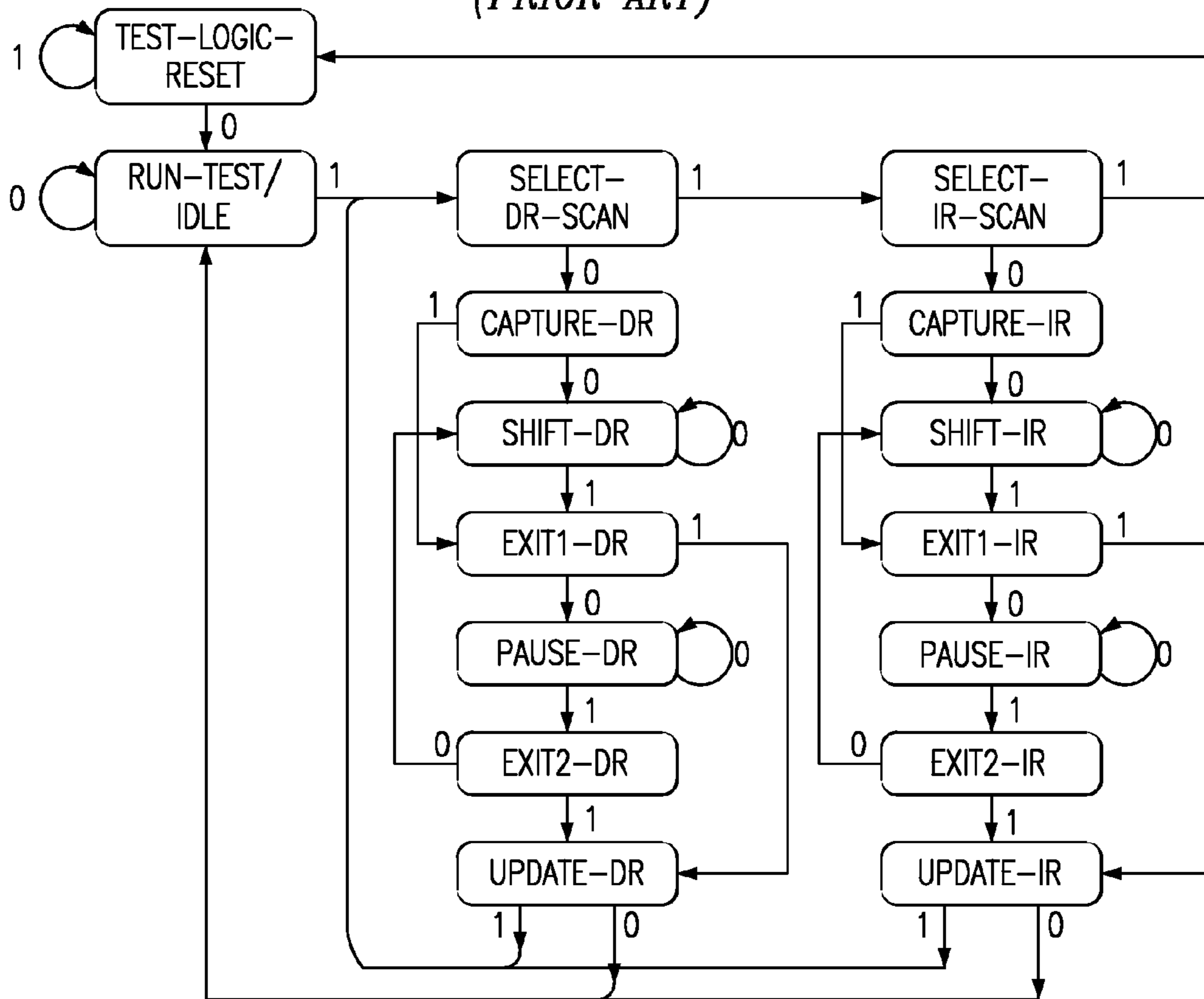
FIG. 14 (PRIOR ART)
