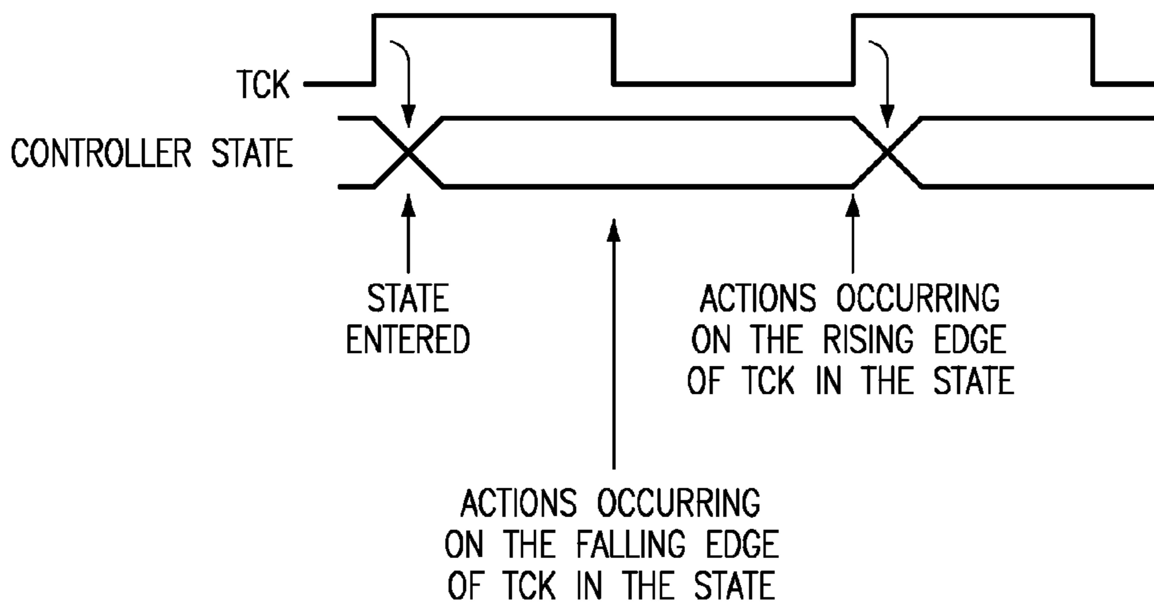
FIG. 15 (PRIOR ART)
