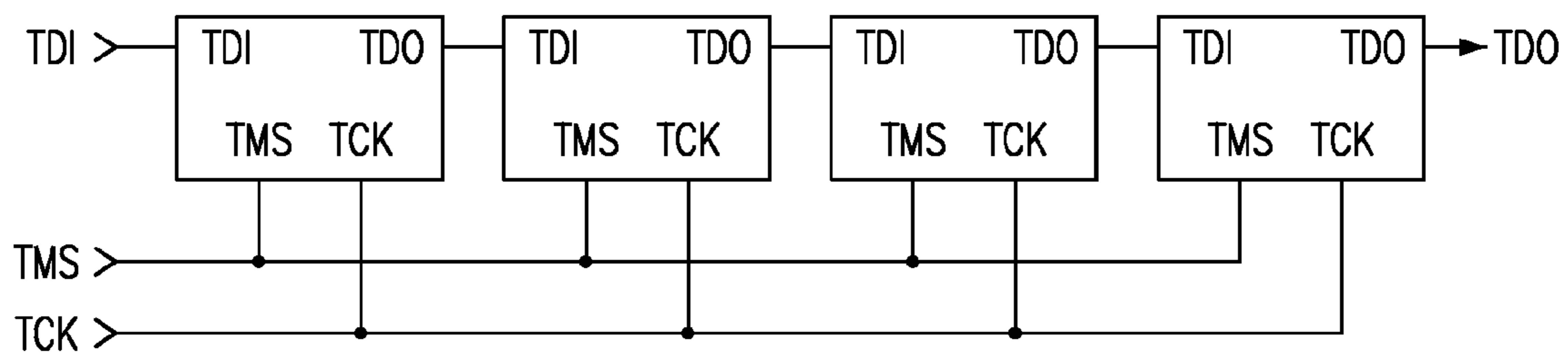
FIG. 13 (PRIOR ART)
