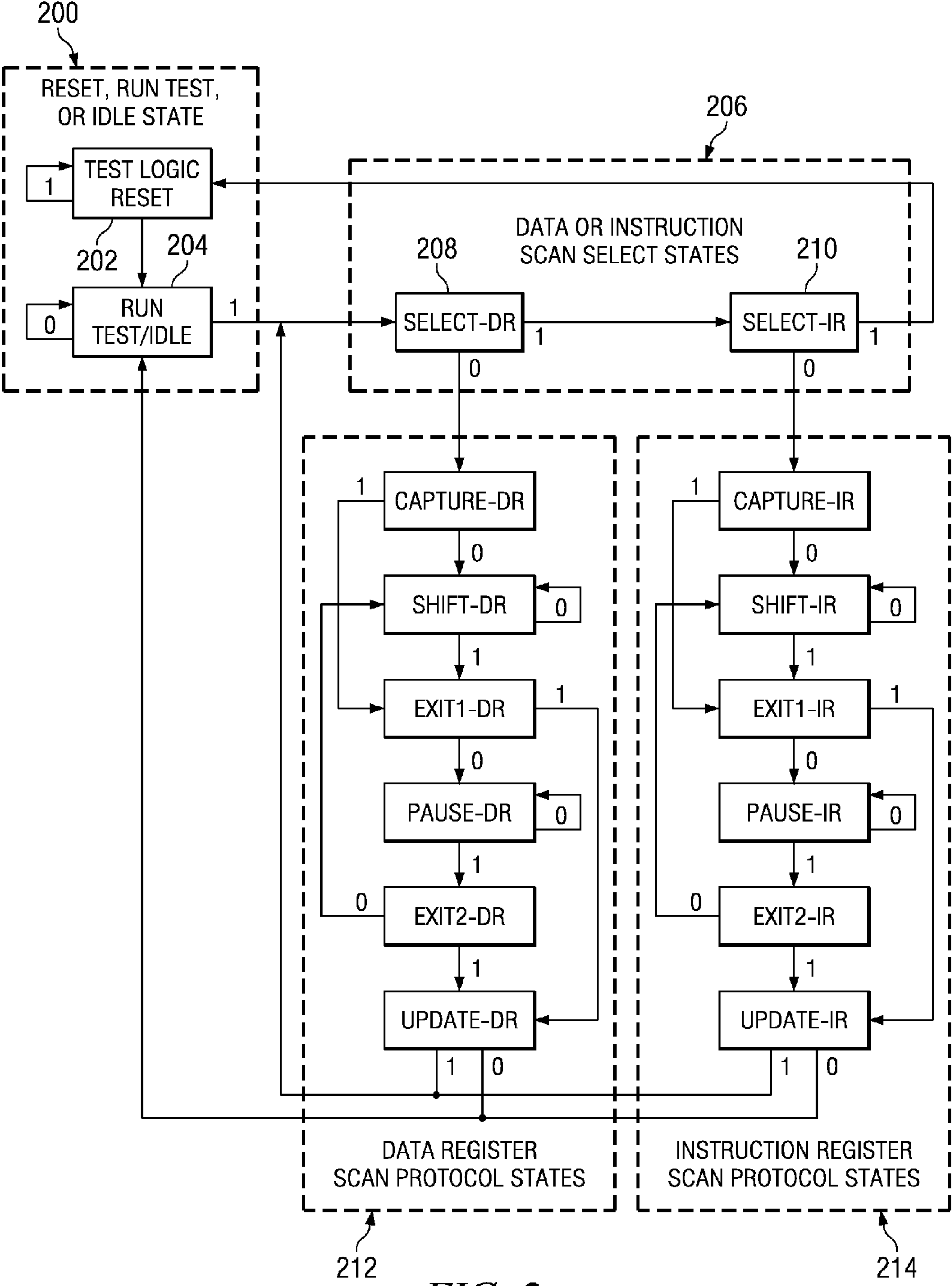
FIG. 2 (PRIOR ART)
