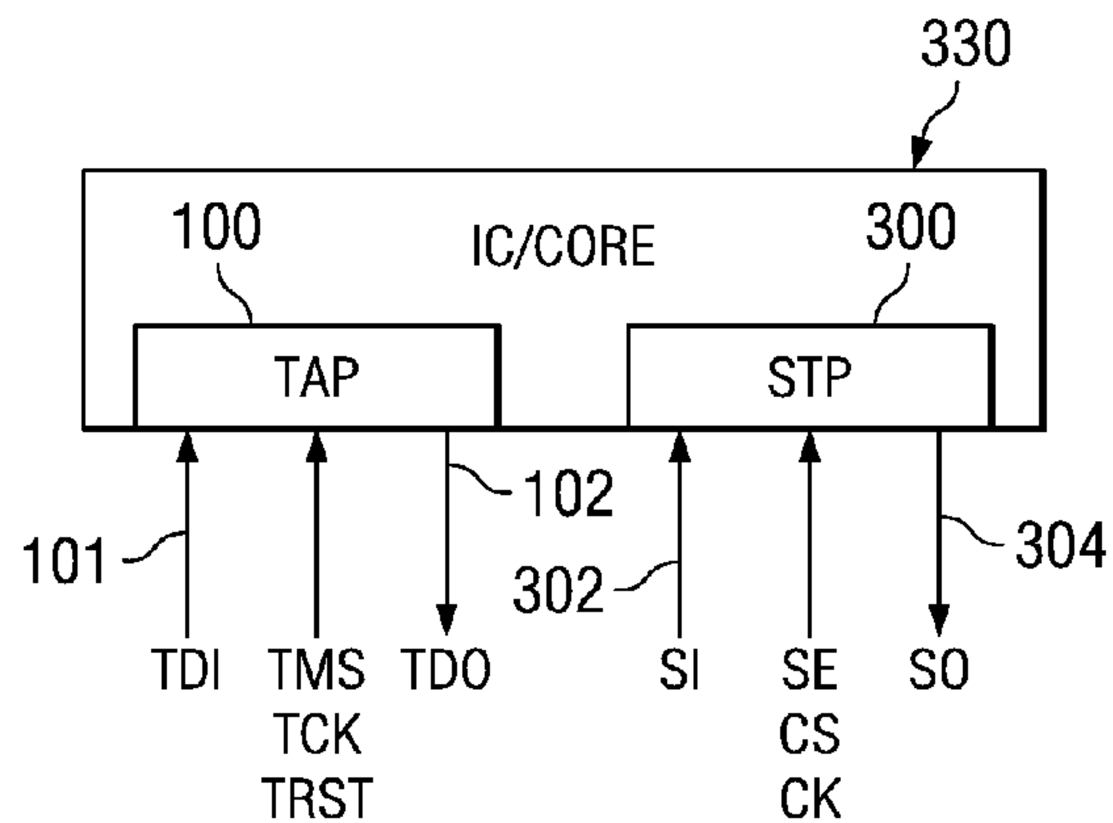
FIG. 3C (PRIOR ART)
