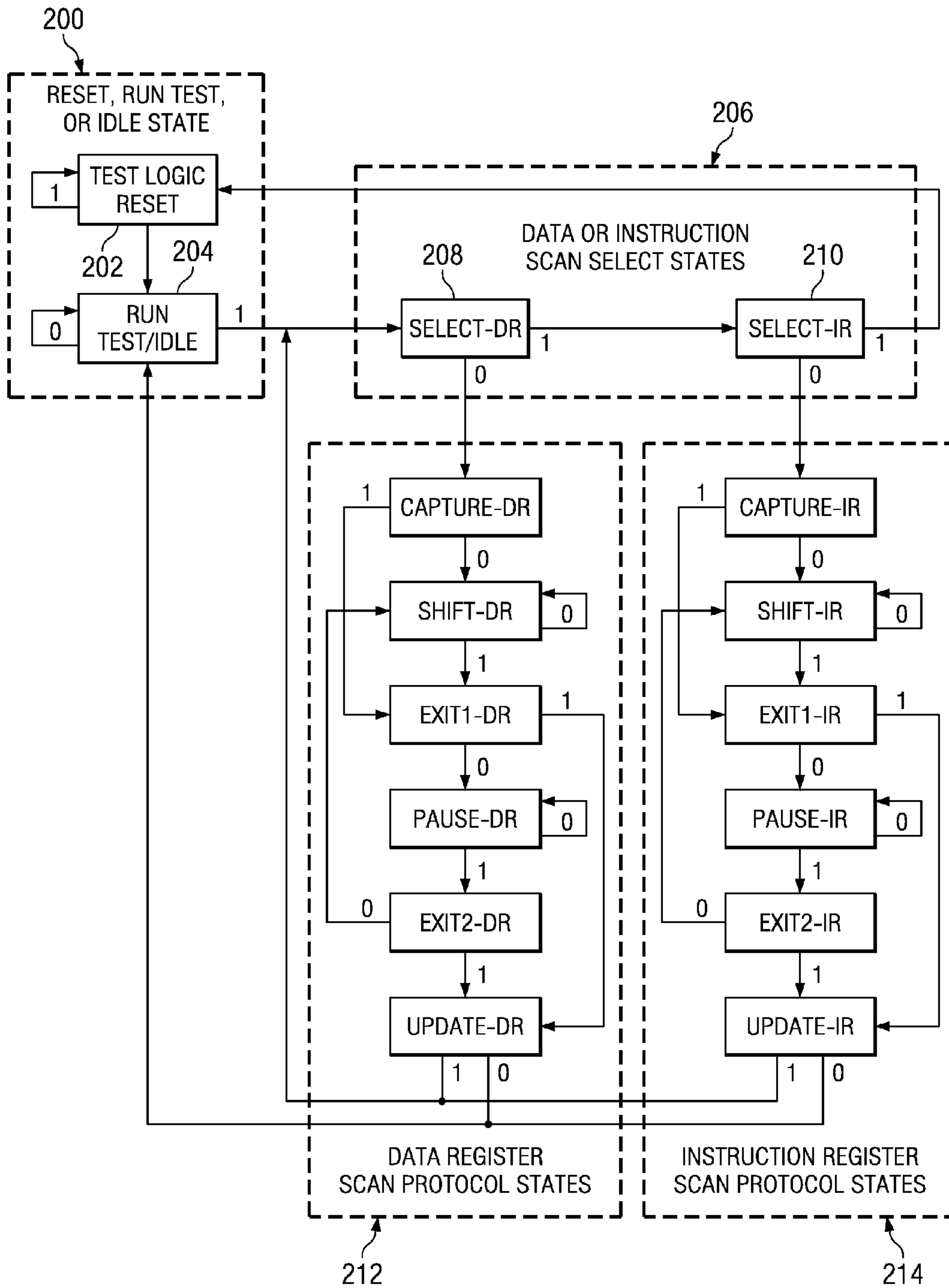
FIG. 2 (PRIOR ART)
