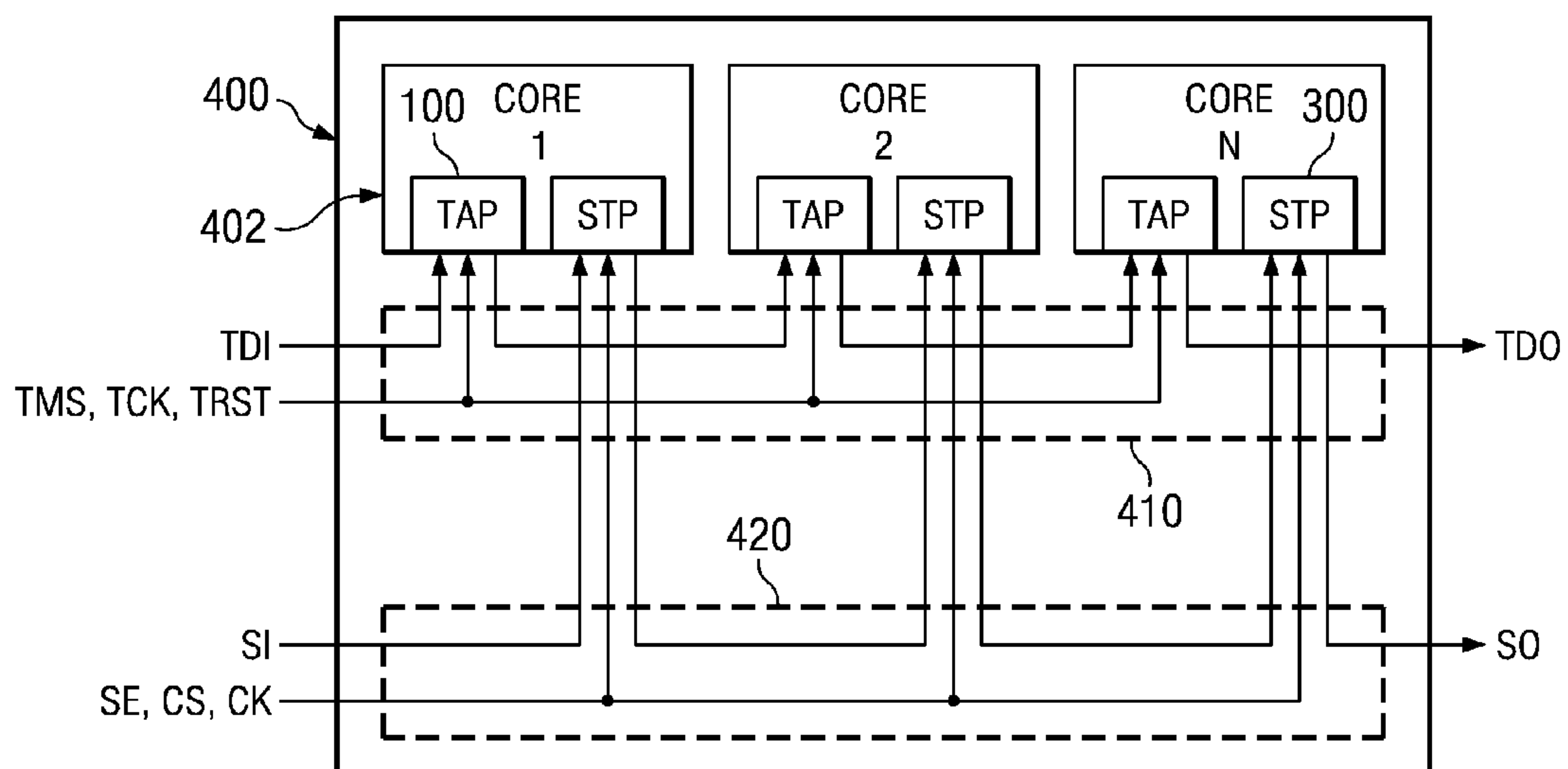
FIG. 4 (PRIOR ART)
