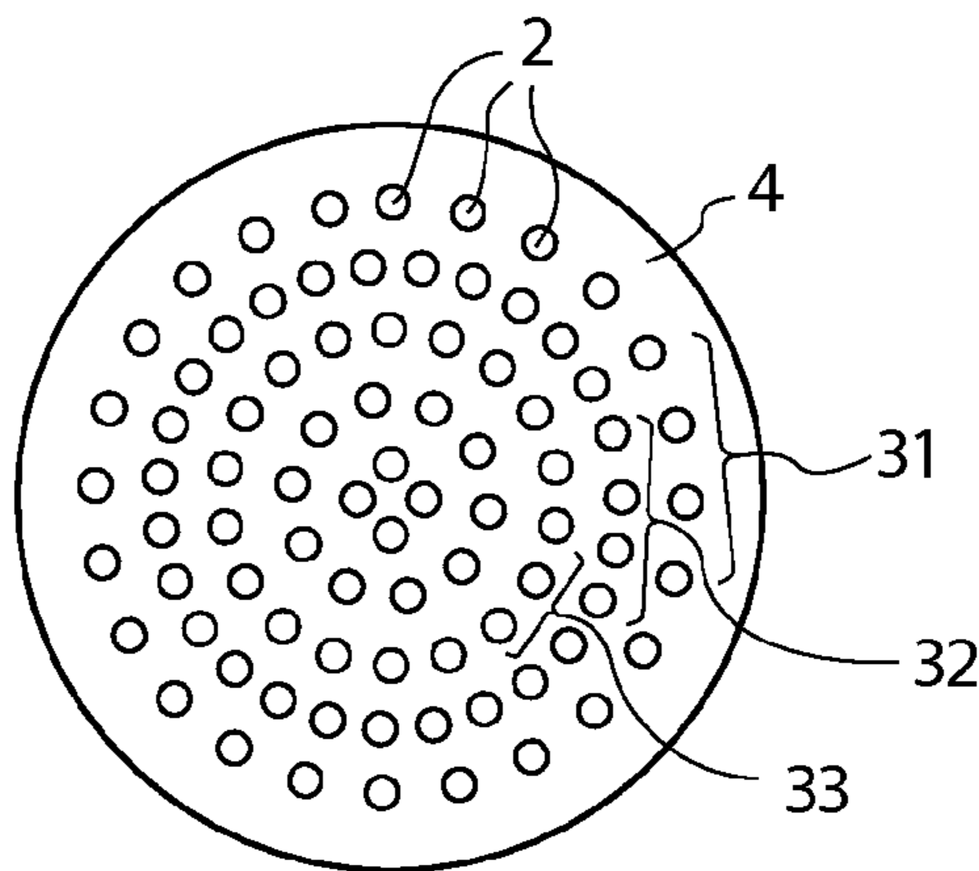
FIG. 2 Prior Art
