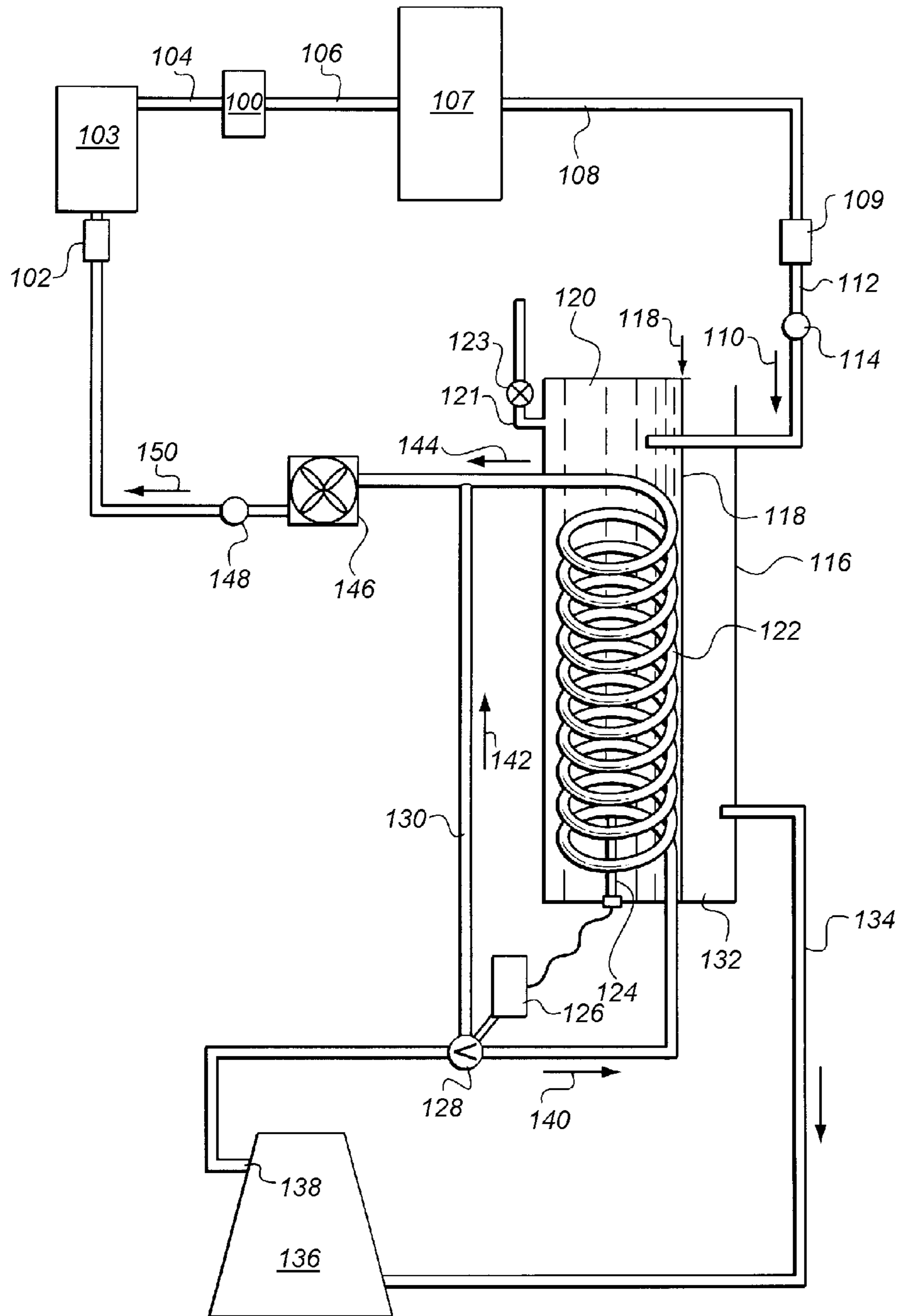
FIG. 3 Prior Art
