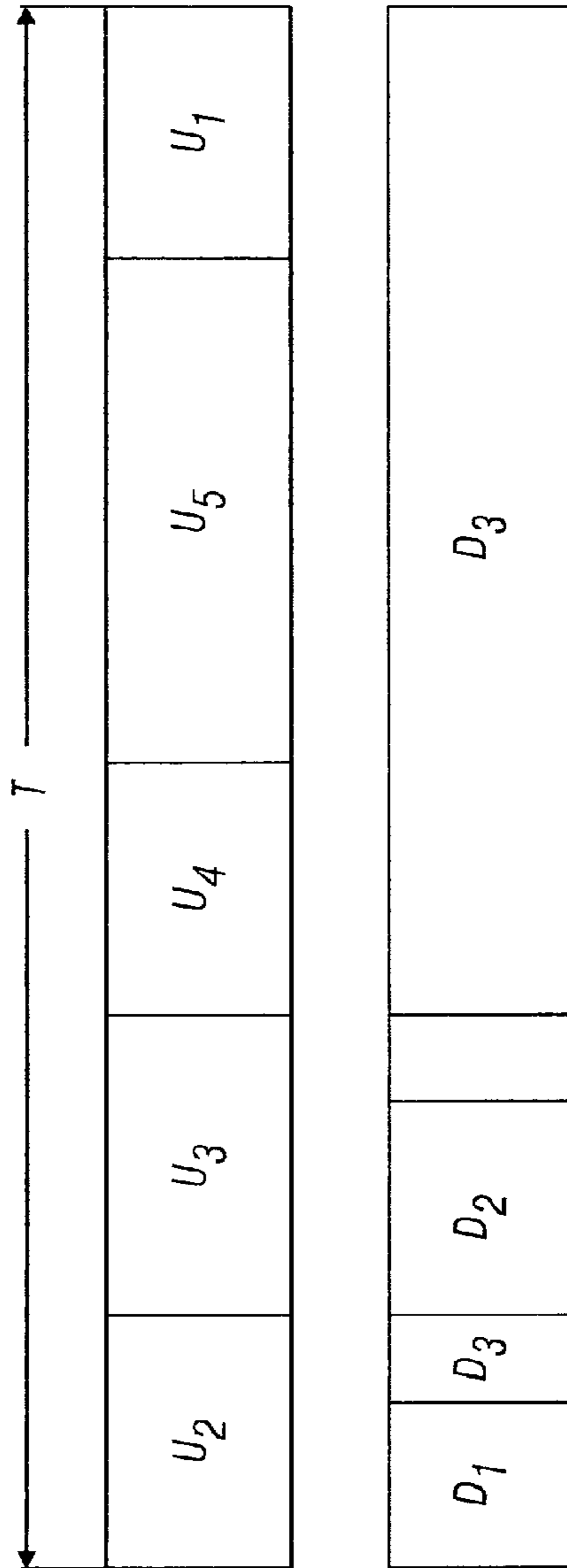
FIG. 18: D_3 > U_4 + U_5 + U_1
