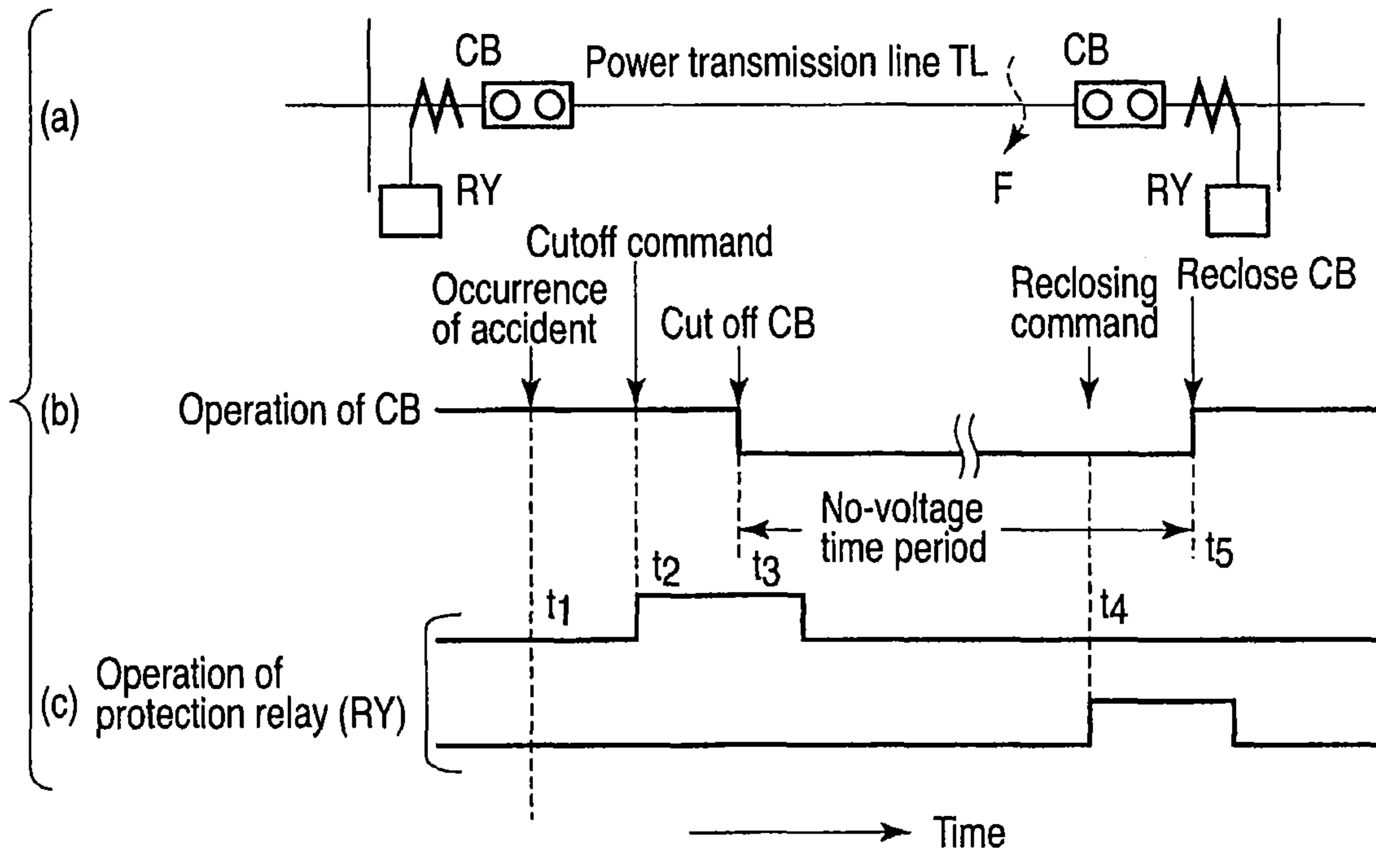
PRIOR ART FIG. 19
