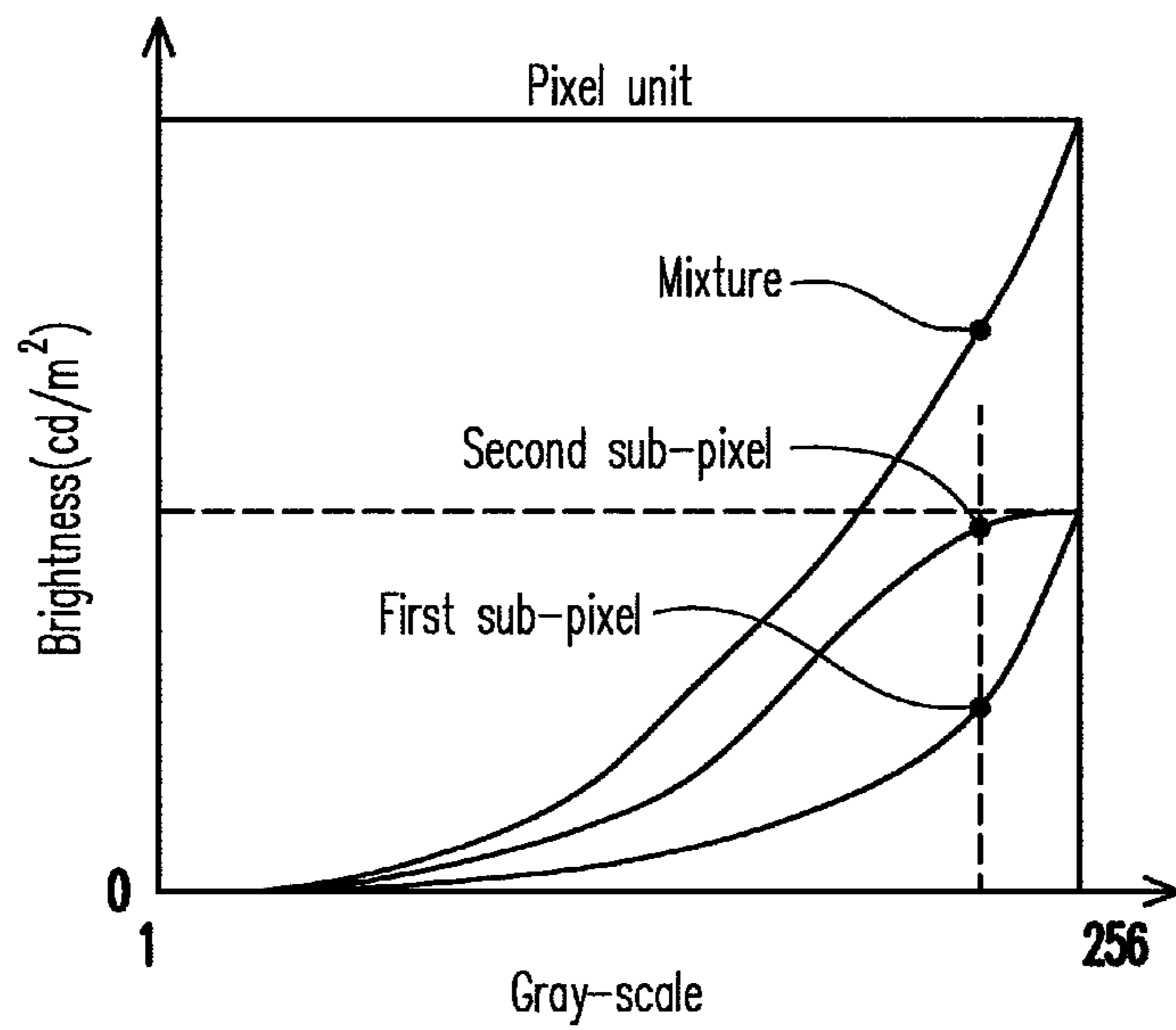
FIG. 2D(PRIOR ART)
