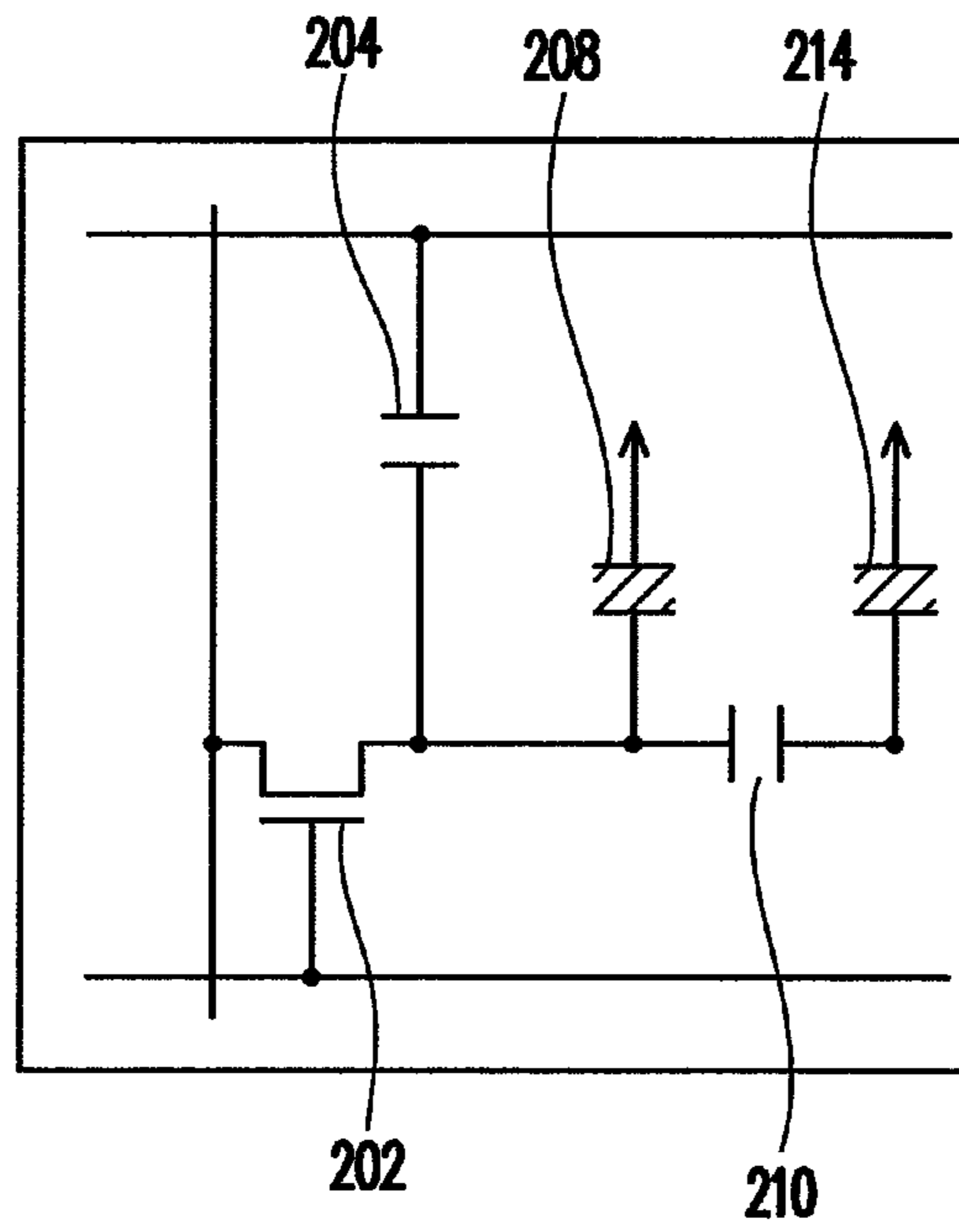
FIG. 2A(PRIOR ART)
