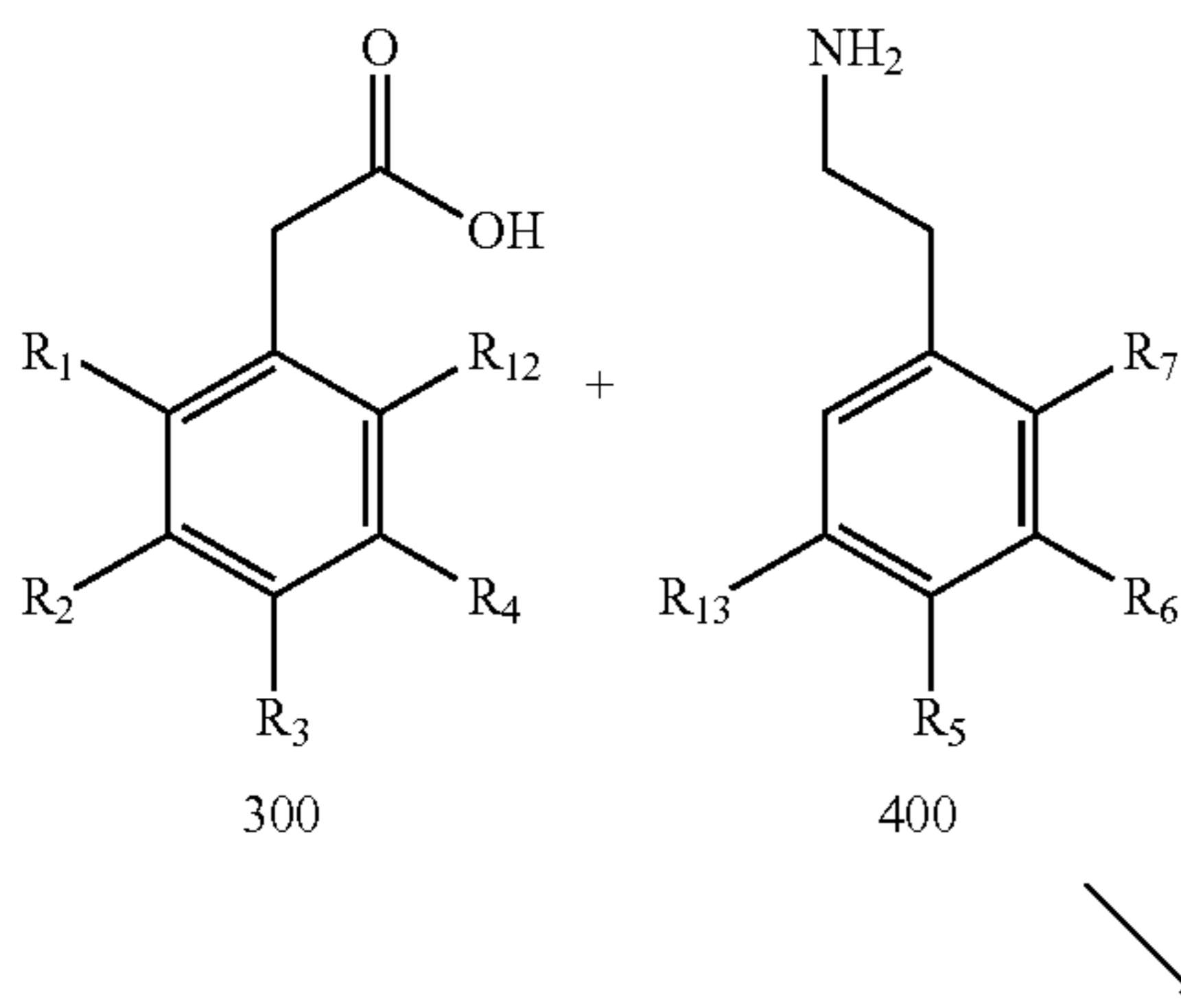
Reaction Scheme 1
