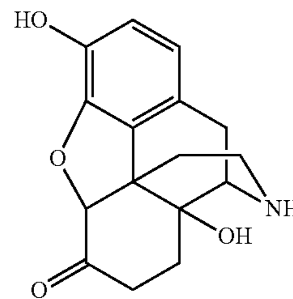
noroxymorphone
