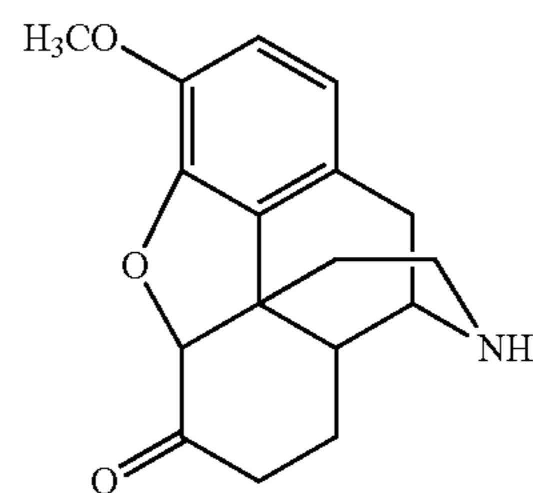
nordihydrocodeinone
