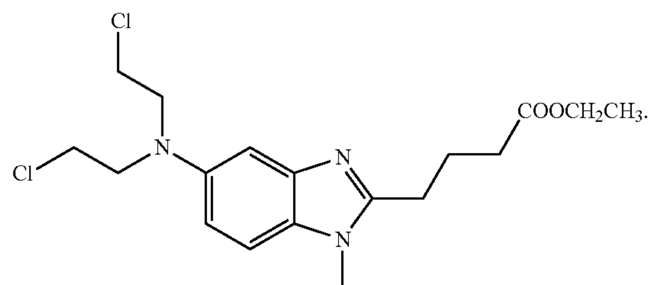
Bendamustine ethylester (BM1EE)
