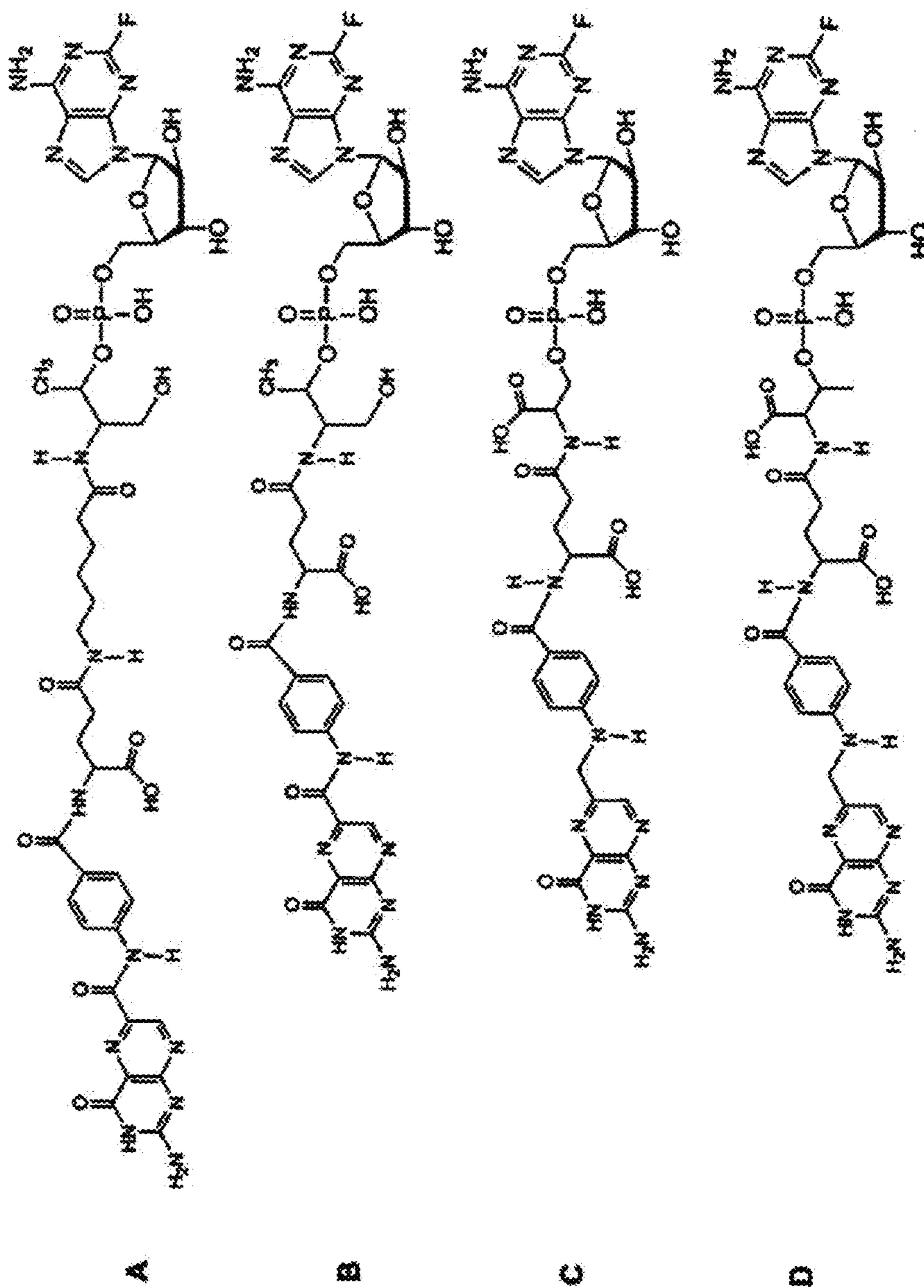
Figure 6: Fludarabine-Folate conjugates
