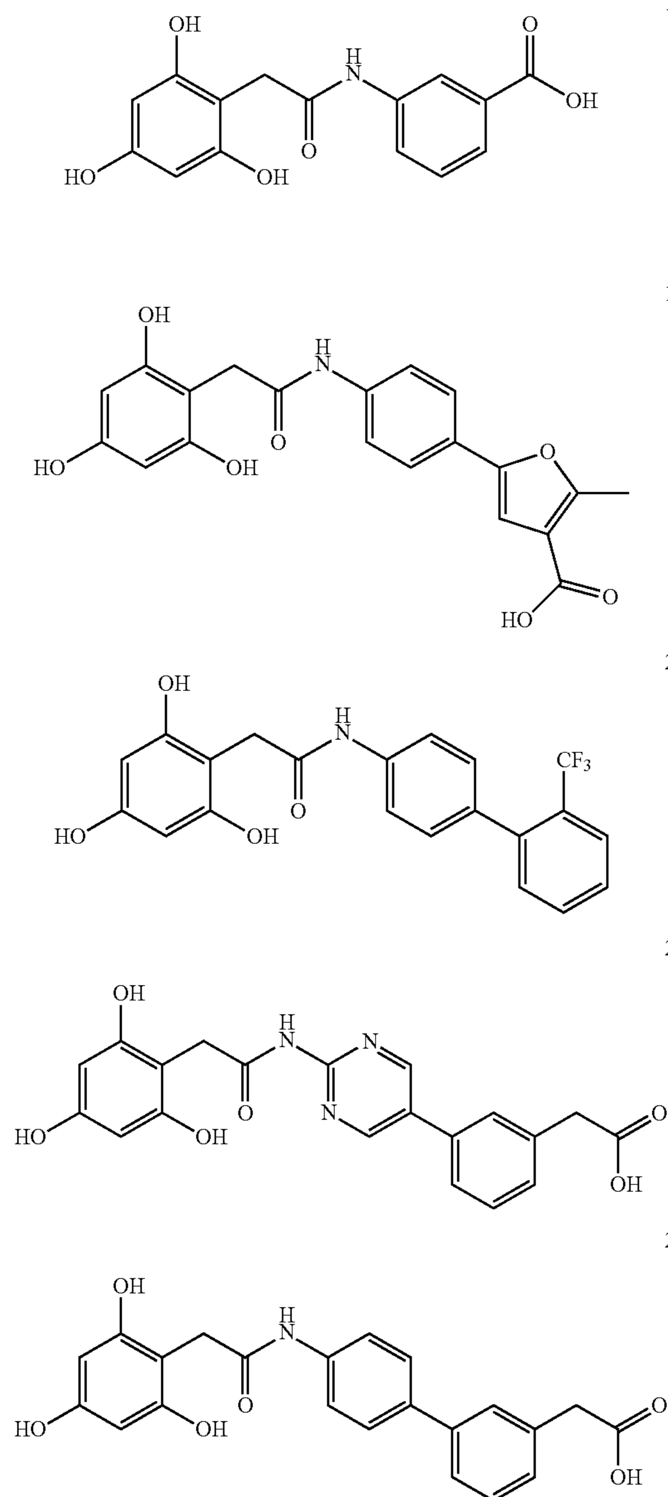
SCHEME 6
