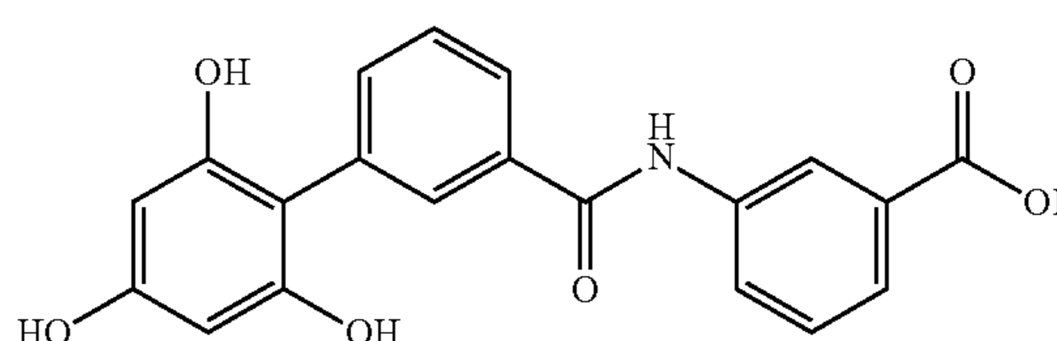
SCHEME 20
