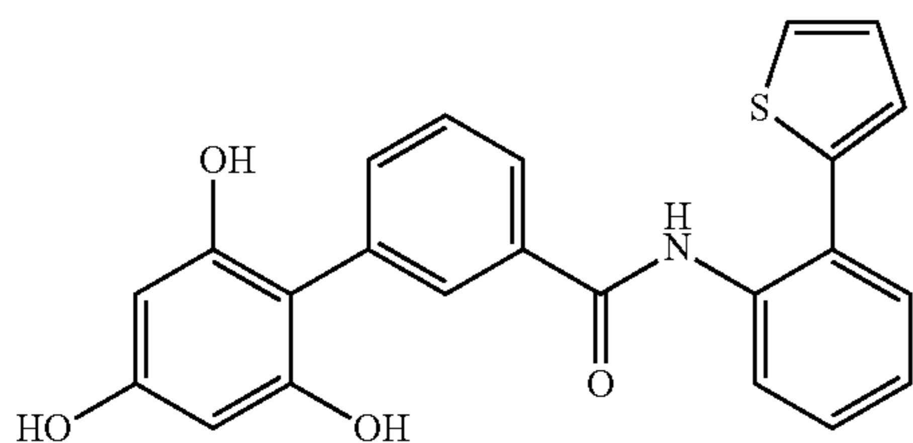
SCHEME 18
