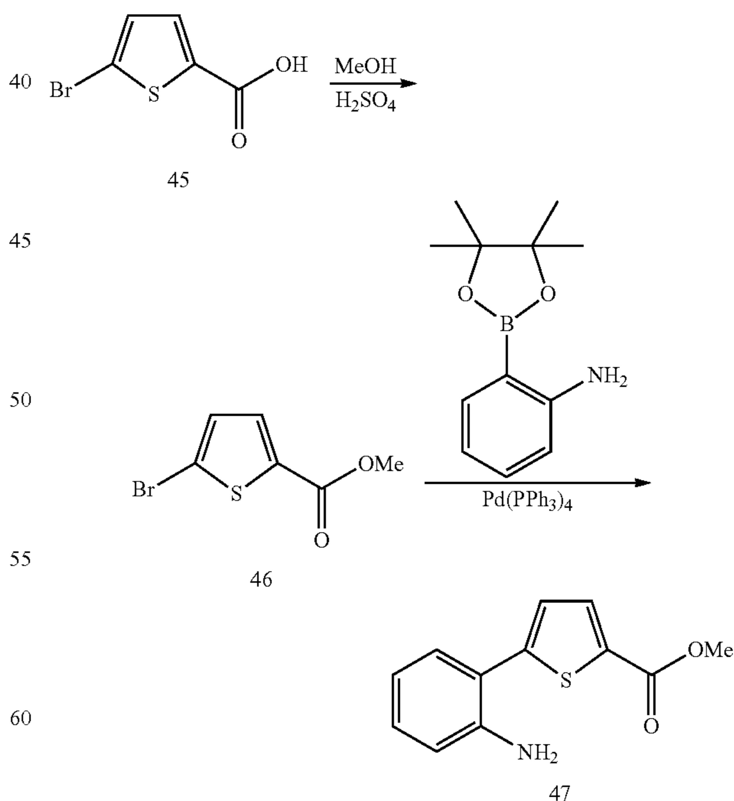
SCHEME 8
