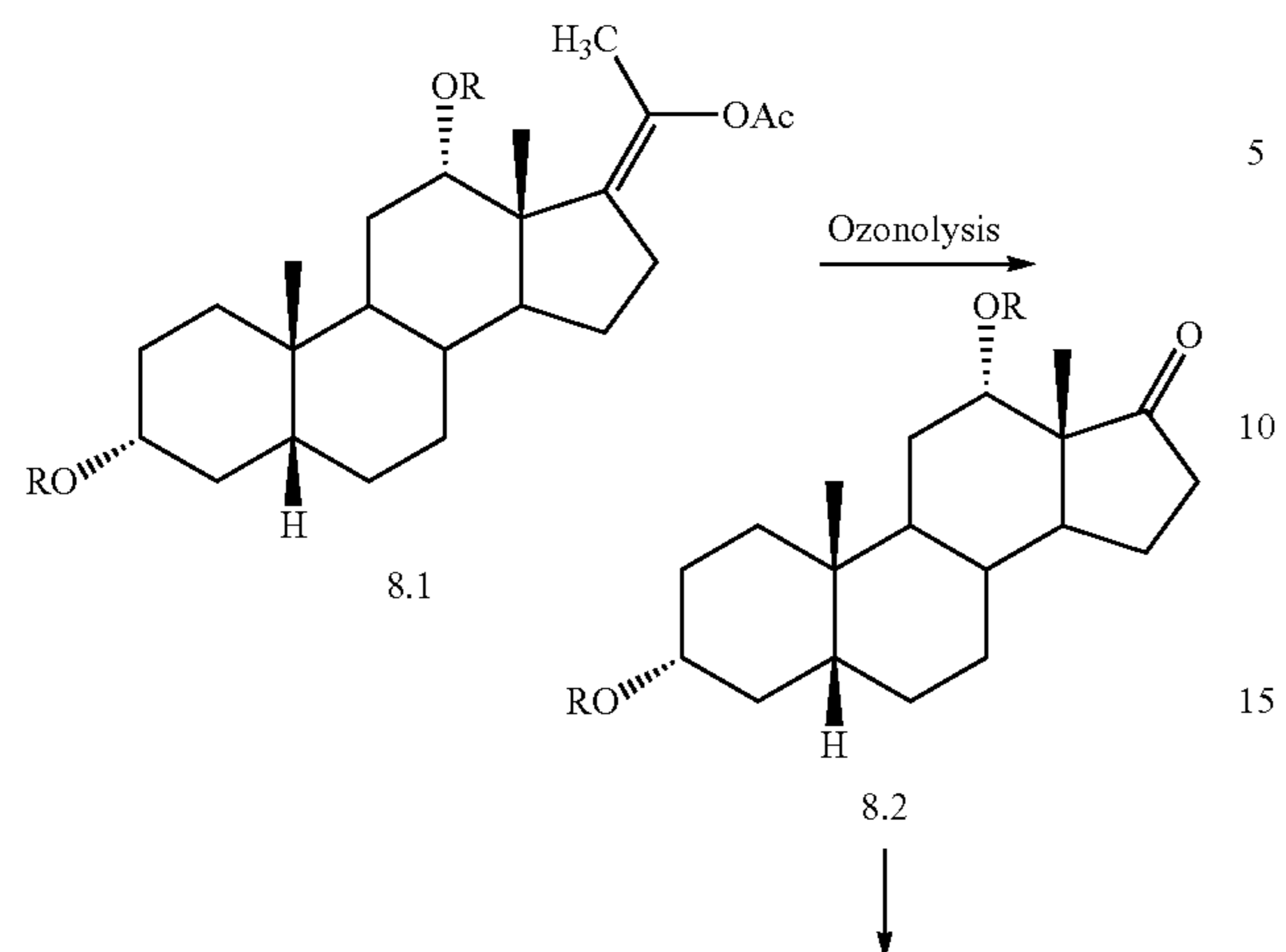
Scheme 8. Side-chain introduction
